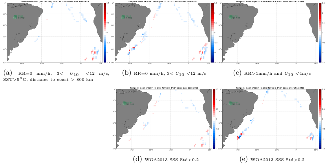
Figure 12: Temporal mean gridded over spatial boxes of size 1^\circ \times 1^\circ of \Delta SSS (SMAP-L3-RSS-V3-MONTHLY-70KM - TSG-POLARSTERN) for 5 different subdatasets corresponding to: RR=0 mm/h, 3 < U_{10} < 12 m/s, SST > 5^\circ C , distance to coast > 800 km (a), RR=0 mm/h, 3 < U_{10} < 12 m/s (b), RR > 1 mm/h and U_{10} < 4 m/s (c), WOA2013 SSS Std < 0.2 (d), WOA2013 SSS Std > 0.2 (e).
