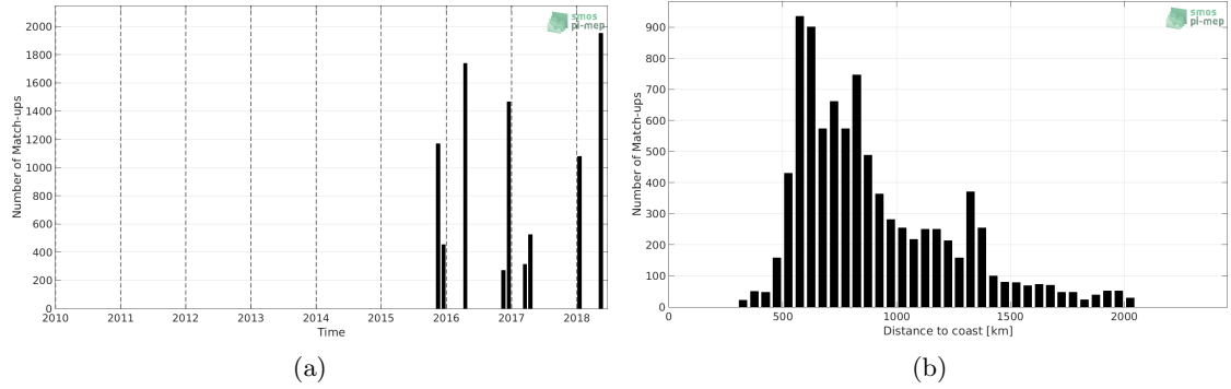
Figure 1: Number of match-ups between TSG-POLARSTERN and SMAP-L3-RSS-V3-MONTHLY-70KM SSS as a function of time (a) and as function of the distance to coast (b) over the South Atlantic Ocean Pi-MEP region and for the full satellite product period.
