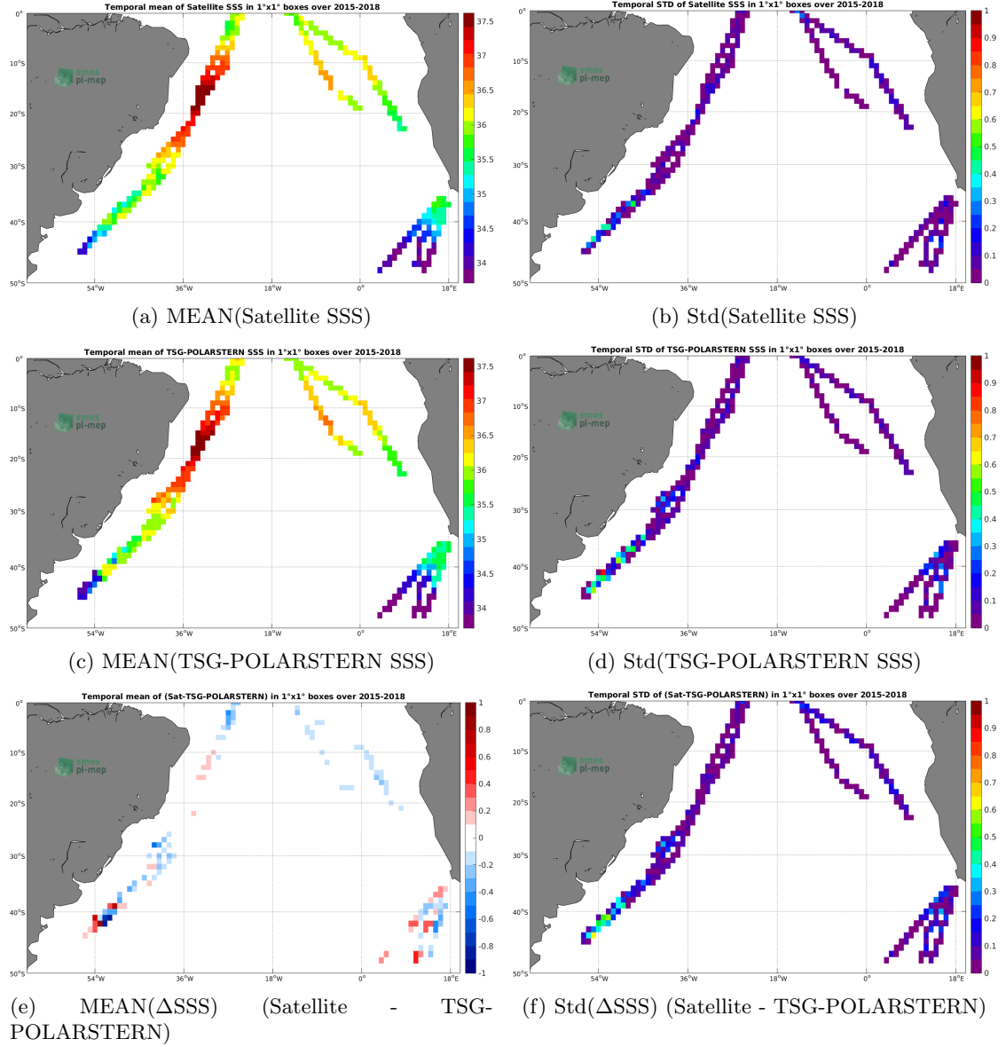
Figure 6: Temporal mean (left) and Std (right) of SSS from SMAP-L3-RSS-V3-MONTHLY-70KM (top), TSG-POLARSTERN (middle), and of \Delta SSS (Satellite - TSG-POLARSTERN). Only match-up pairs are used to generate these maps.
