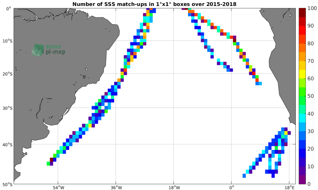
Figure 4: Number of SSS match-ups between TSG-POLARSTERN SSS and the SMAP-L3-RSS-V3-MONTHLY-70KM SSS product for the South Atlantic Ocean Pi-MEP region over 1^\circ \times 1^\circ boxes and for the full satellite product period.
