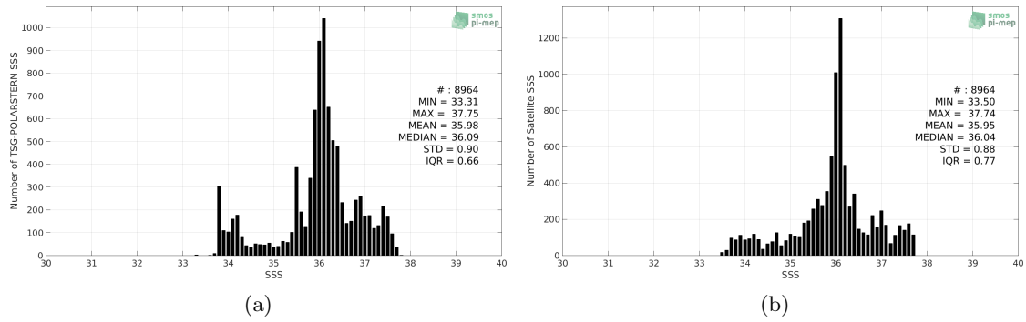
Figure 2: Histograms of SSS from TSG-POLARSTERN (a) and SMAP-L3-RSS-V3-MONTHLY-70KM (b) considering all match-up pairs per bins of 0.1 over the South Atlantic Ocean Pi-MEP region and for the full satellite product period.
