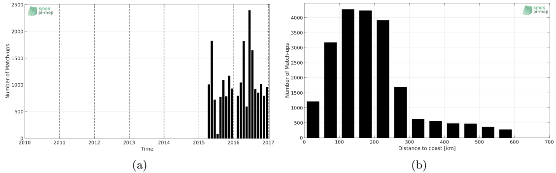
Figure 1: Number of match-ups between TSG-LEGOS-DM and SMAP-L3-RSS-V3-MONTHLY-70KM SSS as a function of time (a) and as function of the distance to coast (b) over the South Atlantic Ocean Pi-MEP region and for the full satellite product period.
