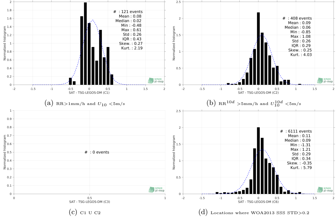
Figure 13: Normalized histogram of \Delta\text{SSS} (SMAP-L3-RSS-V3-MONTHLY-70KM - TSG-LEGOS-DM) for 6 different subdatasets corresponding to: RR > 1\text{mm/h} and U_{10} < 5\text{m/s} (a), RR^{10d} > 5\text{mm/h} and U_{10}^{10d} < 5\text{m/s} (b), C1 \cup C2 (c), Locations where WOA2013 SSS STD > 0.2 (d).
