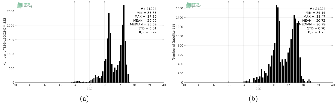
Figure 2: Histograms of SSS from TSG-LEGOS-DM (a) and SMAP-L3-RSS-V3-MONTHLY-70KM (b) considering all match-up pairs per bins of 0.1 over the South Atlantic Ocean Pi-MEP region and for the full satellite product period.
