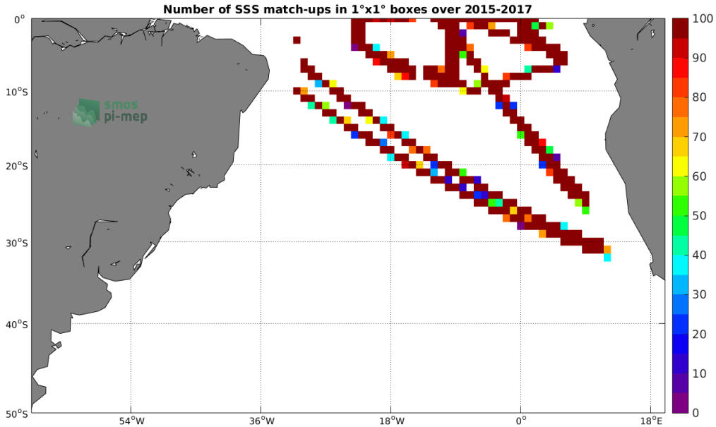
Figure 4: Number of SSS match-ups between TSG-GOSUD-Research-vessel SSS and the SMAP-L3-RSS-V3-MONTHLY-70KM SSS product for the South Atlantic Ocean Pi-MEP region over 1^\circ \times 1^\circ boxes and for the full satellite product period.
