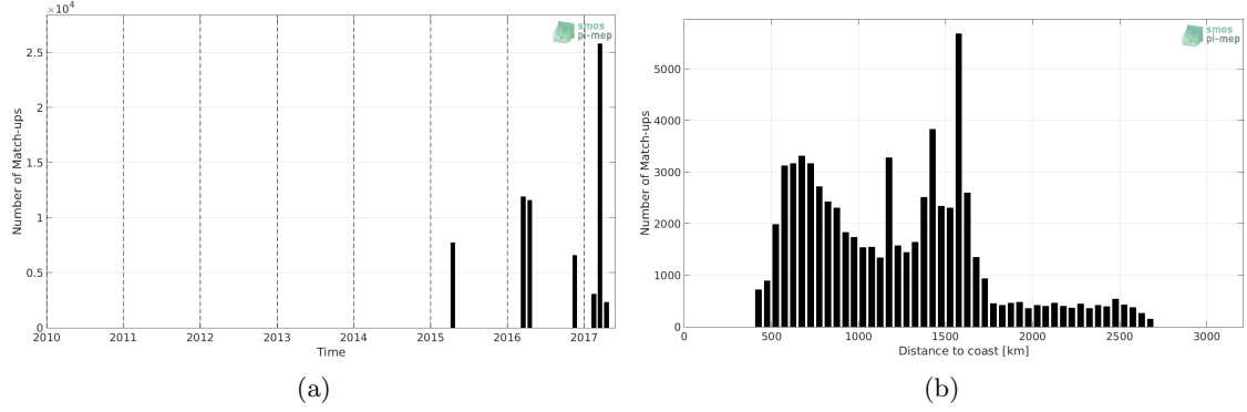
Figure 1: Number of match-ups between TSG-GOSUD-Research-vessel and SMAP-L3-RSS-V3-MONTHLY-70KM SSS as a function of time (a) and as function of the distance to coast (b) over the South Atlantic Ocean Pi-MEP region and for the full satellite product period.
