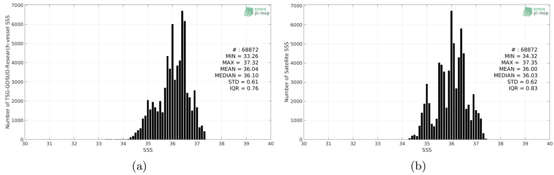
Figure 2: Histograms of SSS from TSG-GOSUD-Research-vessel (a) and SMAP-L3-RSS-V3-MONTHLY-70KM (b) considering all match-up pairs per bins of 0.1 over the South Atlantic Ocean Pi-MEP region and for the full satellite product period.
