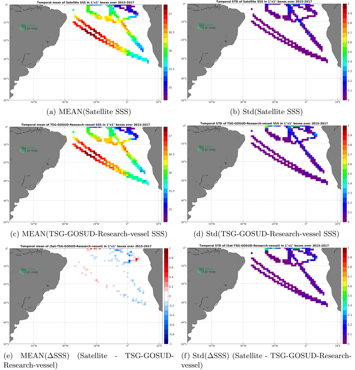
Figure 6: Temporal mean (left) and Std (right) of SSS from SMAP-L3-RSS-V3-MONTHLY-70KM (top), TSG-GOSUD-Research-vessel (middle), and of \Delta SSS (Satellite - TSG-GOSUD-Research-vessel). Only match-up pairs are used to generate these maps.
