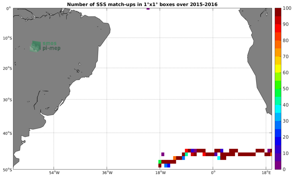
Figure 3: Number of SSS match-ups between Surface drifters SSS and the SMAP-L3-RSS-V3-MONTHLY-70KM SSS product for the South Atlantic Ocean Pi-MEP region over 1^\circ \times 1^\circ boxes and for the full satellite product period.
