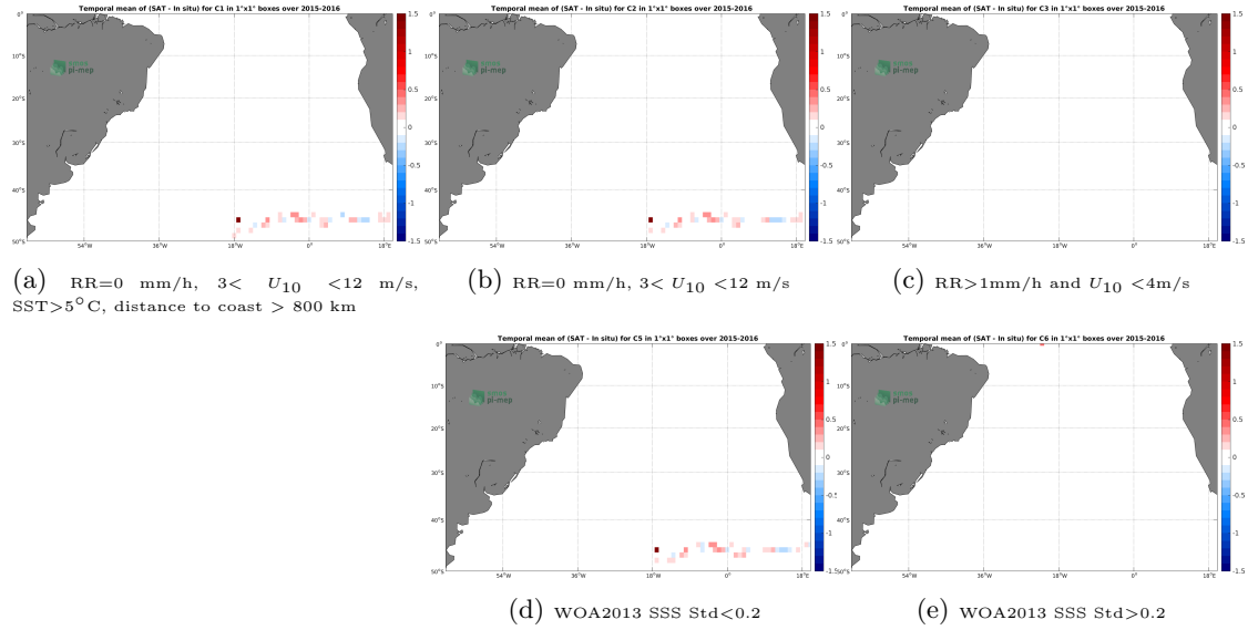
Figure 11: Temporal mean gridded over spatial boxes of size 1^\circ \times 1^\circ of \Delta SSS (SMAP-L3-RSS-V3-MONTHLY-70KM - Surface drifters) for 5 different subdatasets corresponding to: RR=0 mm/h, 3 < U_{10} < 12 m/s, SST > 5^\circ C , distance to coast > 800 km (a), RR=0 mm/h, 3 < U_{10} < 12 m/s (b), RR > 1 mm/h and U_{10} < 4 m/s (c), WOA2013 SSS Std < 0.2 (d), WOA2013 SSS Std > 0.2 (e).
