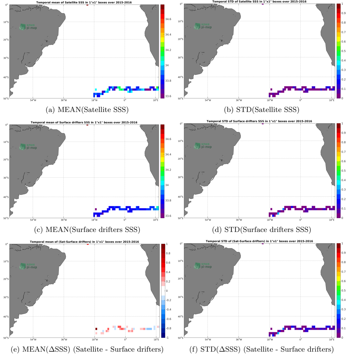
Figure 5: Temporal mean (left) and STD (right) of SSS from SMAP-L3-RSS-V3-MONTHLY-70KM (top), Surface drifters (middle), and of \Delta SSS (Satellite - Surface drifters). Only match-up pairs are used to generate these maps.
