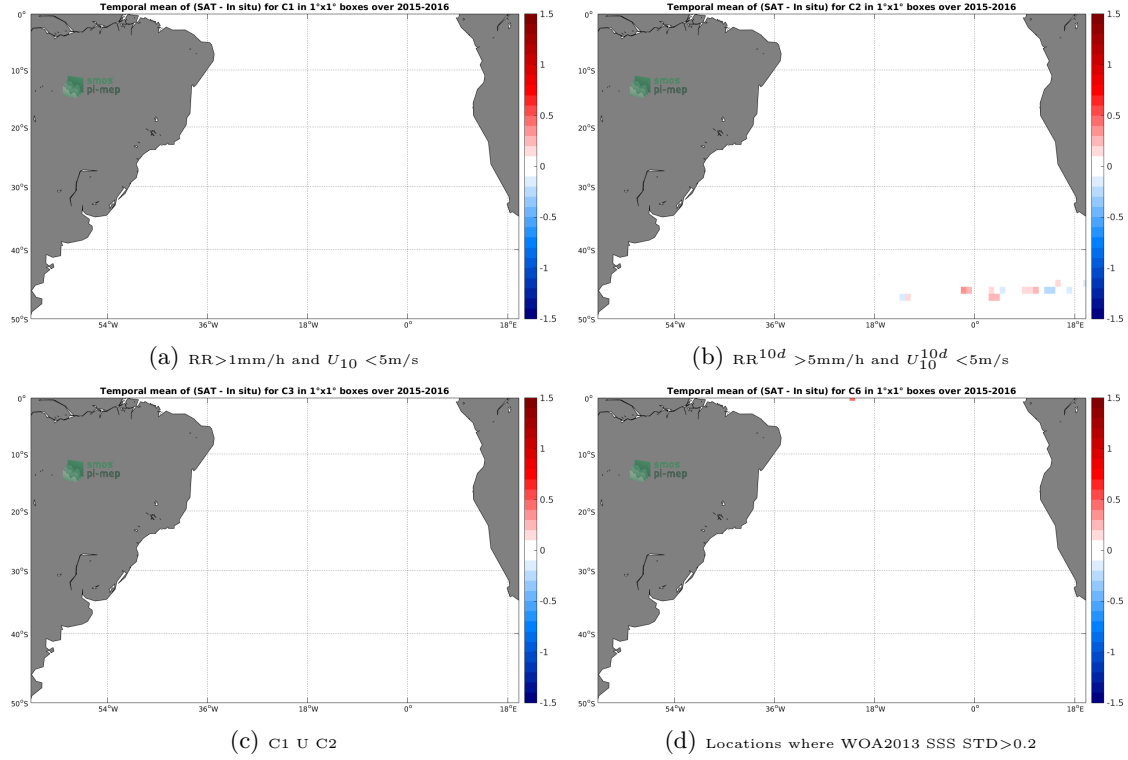
Figure 11: Temporal mean gridded over spatial boxes of size 1^\circ \times 1^\circ of \Delta SSS (SMAP-L3-RSS-V3-MONTHLY-70KM - Surface drifters) for 4 different subdatasets corresponding to: RR > 1\text{mm/h} and U_{10} < 5\text{m/s} (a), RR^{10d} > 5\text{mm/h} and U_{10}^{10d} < 5\text{m/s} (b), C1 U C2 (c), Locations where WOA2013 SSS STD > 0.2 (d).
