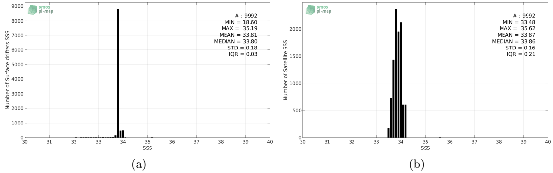
Figure 2: Histograms of SSS from Surface drifters (a) and SMAP-L3-RSS-V3-MONTHLY-70KM (b) considering all match-up pairs per bins of 0.1 over the South Atlantic Ocean Pi-MEP region and for the full satellite product period.
