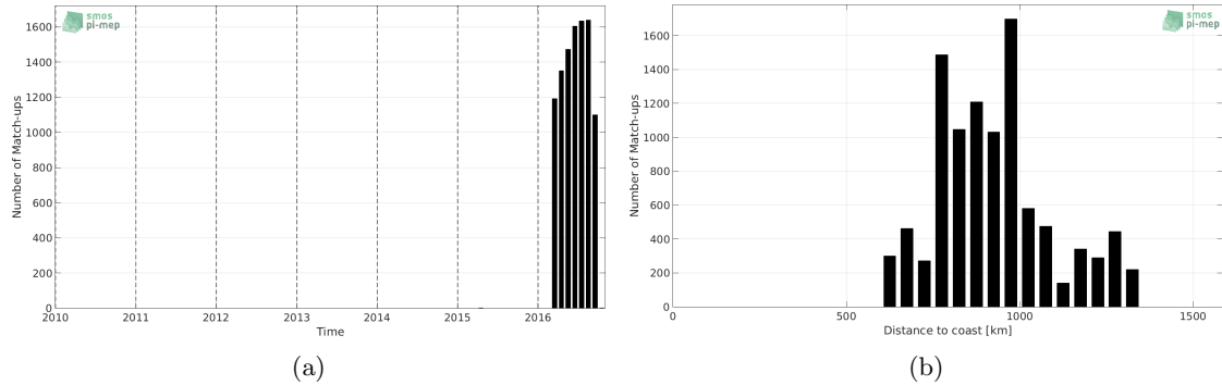
Figure 1: Number of match-ups between Surface drifters and SMAP-L3-RSS-V3-MONTHLY-70KM SSS as a function of time (a) and as function of the distance to coast (b) over the South Atlantic Ocean Pi-MEP region and for the full satellite product period.
