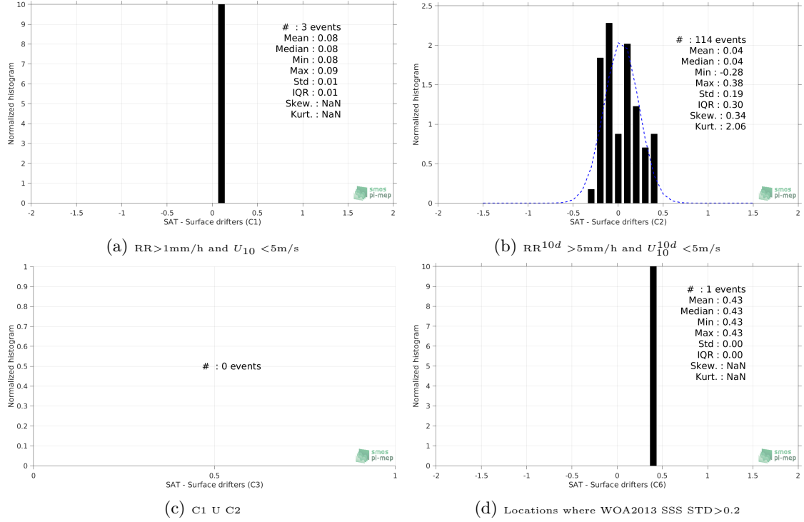
Figure 12: Normalized histogram of \Delta SSS (SMAP-L3-RSS-V3-MONTHLY-70KM - Surface drifters) for 6 different subdatasets corresponding to: RR > 1mm/h and U_{10} < 5\text{m/s} (a), RR^{10d} > 5\text{mm/h} and U_{10}^{10d} < 5\text{m/s} (b), C1 U C2 (c), Locations where WOA2013 SSS STD > 0.2 (d).
