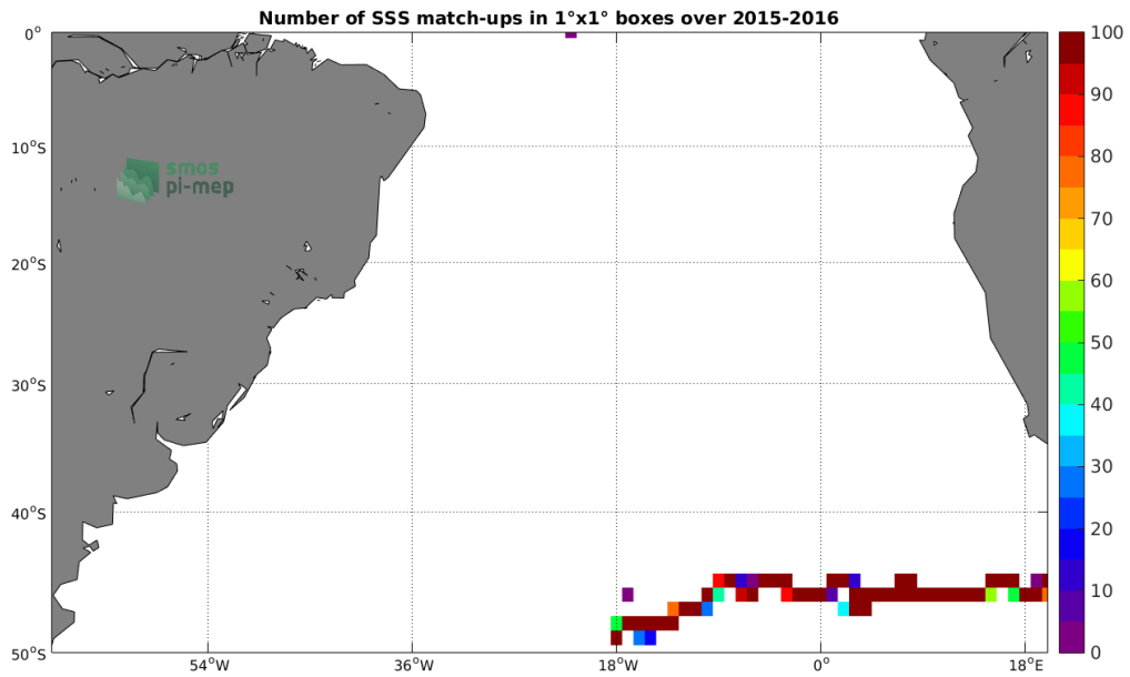
Figure 3: Number of SSS match-ups between Surface drifters SSS and the SMAP-L3-RSS-V3-MONTHLY-70KM SSS product for the South Atlantic Ocean Pi-MEP region over 1°x1° boxes and for the full satellite product period.
