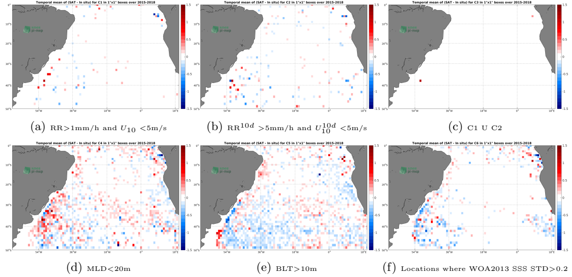
Figure 12: Temporal mean gridded over spatial boxes of size 1^\circ \times 1^\circ of \Delta\text{SSS} (SMAP-L3-RSS-V3-MONTHLY-70KM - Argo) for 6 different subdatasets corresponding to: \text{RR} > 1\text{mm/h} and U_{10} < 5\text{m/s} (a), \text{RR}^{10d} > 5\text{mm/h} and U_{10}^{10d} < 5\text{m/s} (b), C1 U C2 (c), \text{MLD} < 20\text{m} (d), \text{BLT} > 10\text{m} (e), Locations where WOA2013 SSS STD > 0.2 (f).
