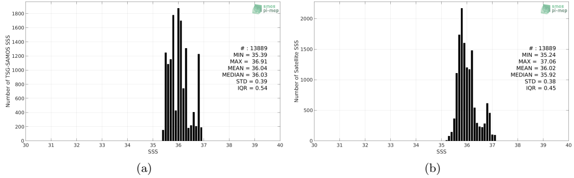
Figure 2: Histograms of SSS from TSG-SAMOS (a) and SMAP-L3-RSS-V3-MONTHLY-0.25DEG-40KM (b) considering all match-up pairs per bins of 0.1 over the South Atlantic Ocean Pi-MEP region and for the full satellite product period.
