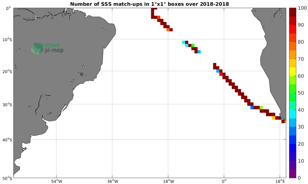
Figure 4: Number of SSS match-ups between TSG-SAMOS SSS and the SMAP-L3-RSS-V3-MONTHLY-0.25DEG-40KM SSS product for the South Atlantic Ocean Pi-MEP region over 1^\circ \times 1^\circ boxes and for the full satellite product period.
