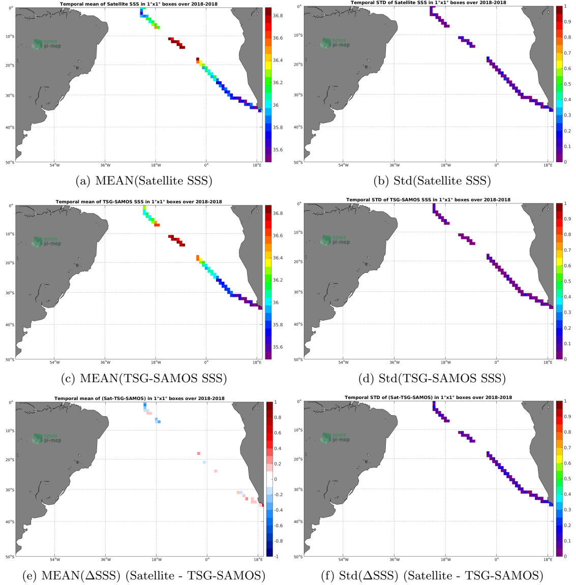
Figure 6: Temporal mean (left) and Std (right) of SSS from SMAP-L3-RSS-V3-MONTHLY-0.25DEG-40KM (top), TSG-SAMOS (middle), and of \Delta SSS (Satellite - TSG-SAMOS). Only match-up pairs are used to generate these maps.
