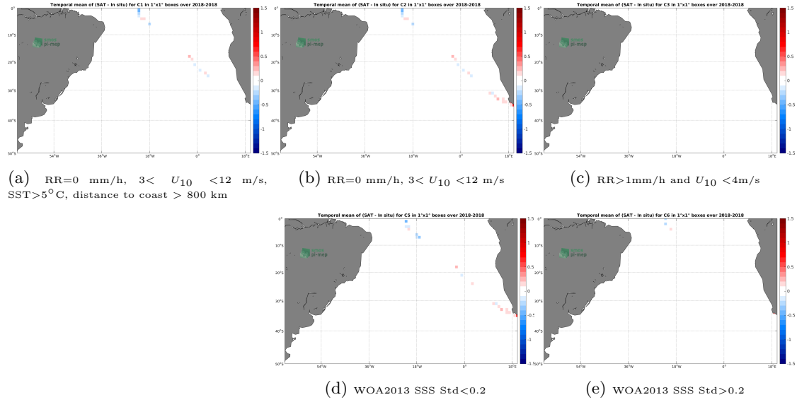
Figure 12: Temporal mean gridded over spatial boxes of size 1^\circ \times 1^\circ of \Delta SSS (SMAP-L3-RSS-V3-MONTHLY-0.25DEG-40KM - TSG-SAMOS) for 5 different subdatasets corresponding to: RR=0 mm/h, 3 < U_{10} < 12 m/s, SST > 5^\circ C , distance to coast > 800 km (a), RR=0 mm/h, 3 < U_{10} < 12 m/s (b), RR > 1 mm/h and U_{10} < 4 m/s (c), WOA2013 SSS Std < 0.2 (d), WOA2013 SSS Std > 0.2 (e).
