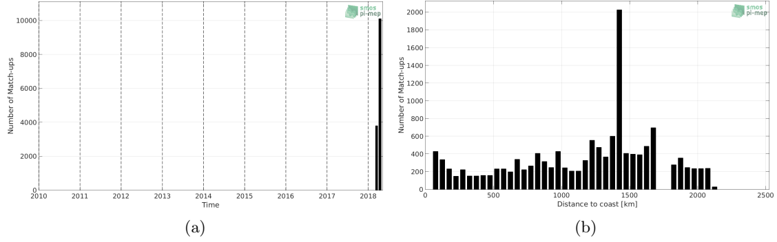
Figure 1: Number of match-ups between TSG-SAMOS and SMAP-L3-RSS-V3-MONTHLY-0.25DEG-40KM SSS as a function of time (a) and as function of the distance to coast (b) over the South Atlantic Ocean Pi-MEP region and for the full satellite product period.
