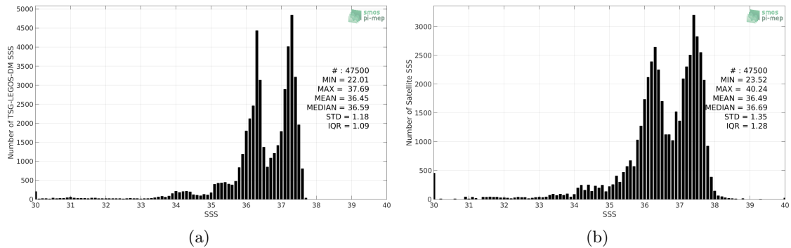
Figure 2: Histograms of SSS from TSG-LEGOS-DM (a) and SMAP-L3-RSS-V3-MONTHLY-0.25DEG-40KM (b) considering all match-up pairs per bins of 0.1 over the South Atlantic Ocean Pi-MEP region and for the full satellite product period.
