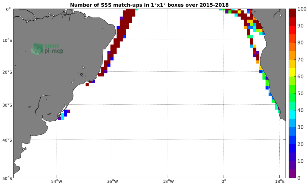
Figure 4: Number of SSS match-ups between TSG-LEGOS-DM SSS and the SMAP-L3-RSS-V3-MONTHLY-0.25DEG-40KM SSS product for the South Atlantic Ocean Pi-MEP region over 1^\circ \times 1^\circ boxes and for the full satellite product period.
