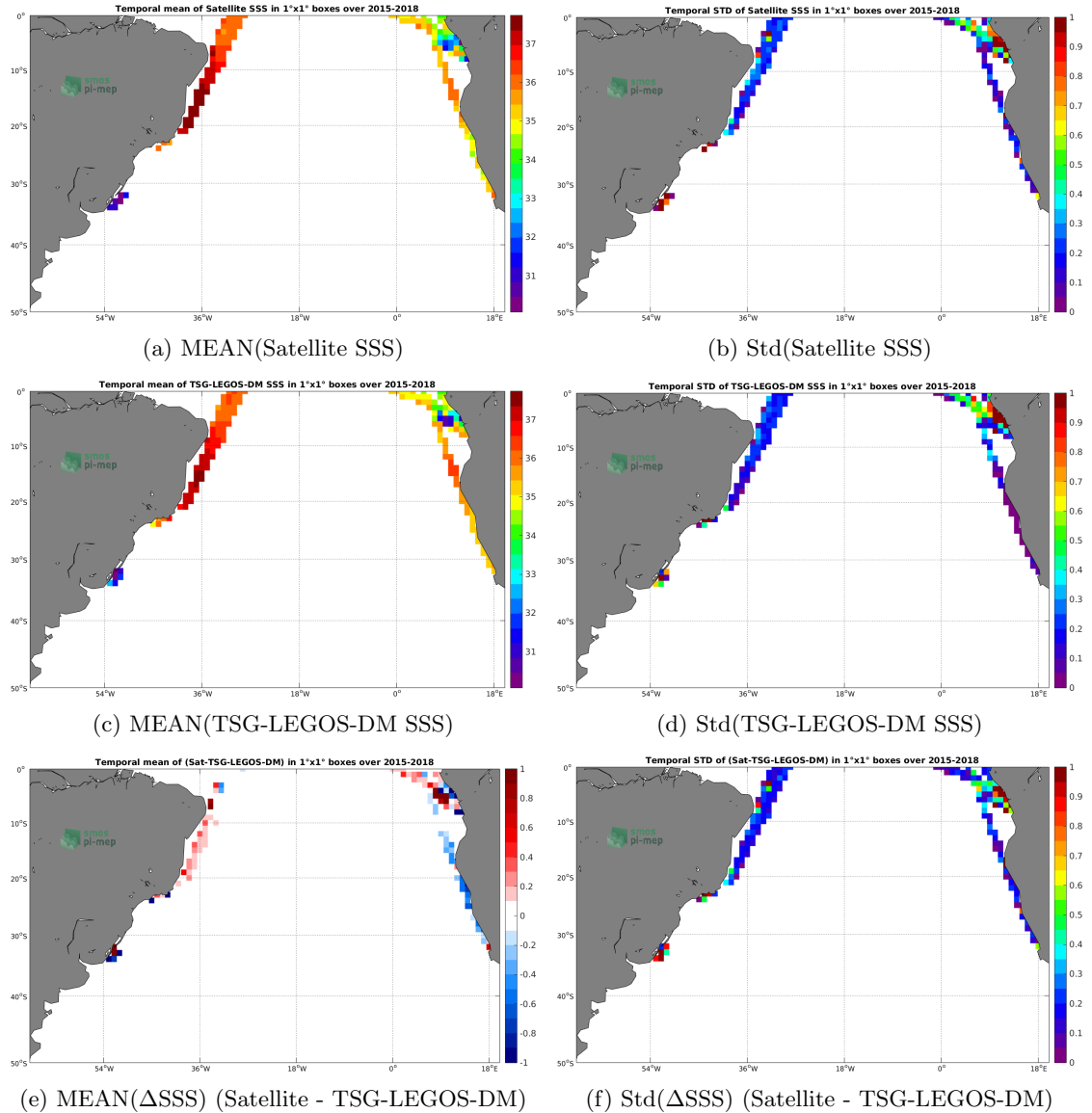
Figure 6: Temporal mean (left) and Std (right) of SSS from SMAP-L3-RSS-V3-MONTHLY-0.25DEG-40KM (top), TSG-LEGOS-DM (middle), and of \Delta SSS (Satellite - TSG-LEGOS-DM). Only match-up pairs are used to generate these maps.
