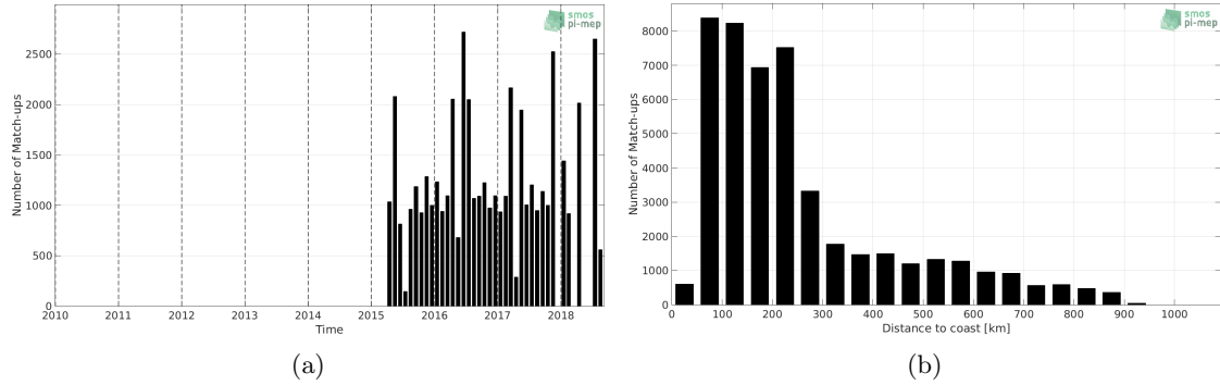
Figure 1: Number of match-ups between TSG-LEGOS-DM and SMAP-L3-RSS-V3-MONTHLY-0.25DEG-40KM SSS as a function of time (a) and as function of the distance to coast (b) over the South Atlantic Ocean Pi-MEP region and for the full satellite product period.
