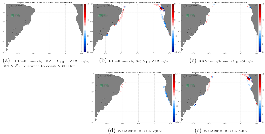
Figure 12: Temporal mean gridded over spatial boxes of size 1^\circ \times 1^\circ of \Delta SSS (SMAP-L3-RSS-V3-MONTHLY-0.25DEG-40KM - TSG-LEGOS-DM) for 5 different subdatasets corresponding to:RR=0 mm/h, 3 < U_{10} < 12 m/s, SST >5^\circ\text{C} , distance to coast > 800 km (a), RR=0 mm/h, 3 < U_{10} < 12 m/s (b), RR >1 mm/h and U_{10} < 4 m/s (c), WOA2013 SSS Std <0.2 (d), WOA2013 SSS Std >0.2 (e).
