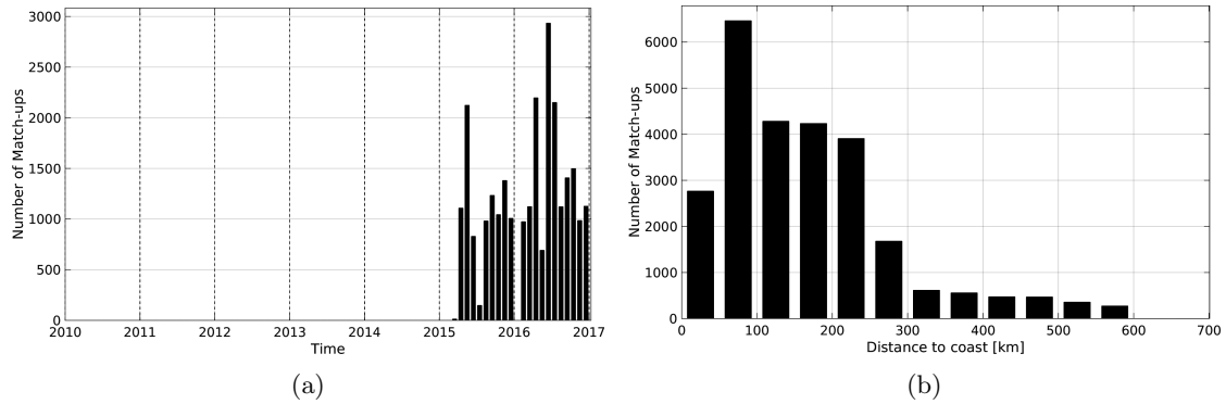
Figure 1: Number of match-ups between TSG-LEGOS-DM and SMAP-L3-RSS-V2-8DAY-RUNNING-40KM SSS as a function of time (a) and as function of the distance to coast (b) over the South Atlantic Ocean Pi-MEP region and for the full satellite product period.
