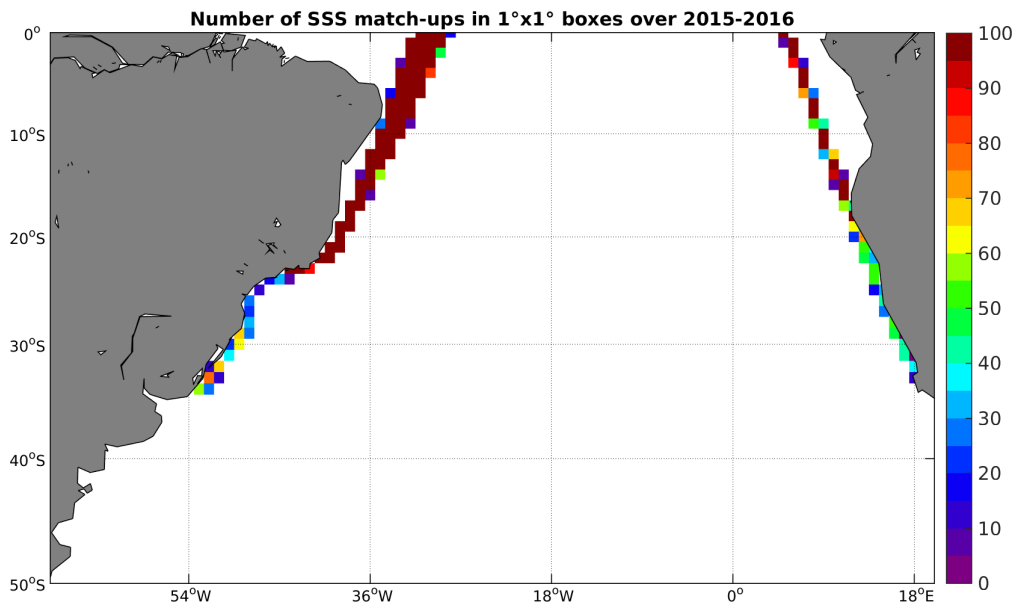
Figure 4: Number of SSS match-ups between TSG-LEGOS-DM SSS and the SMAP-L3-RSS-V2-8DAY-RUNNING-40KM SSS product for the South Atlantic Ocean Pi-MEP region over 1^\circ \times 1^\circ boxes and for the full satellite product period.
