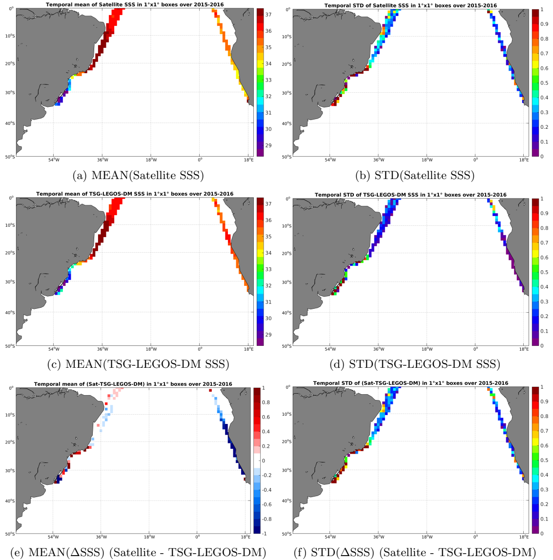
Figure 6: Temporal mean (left) and STD (right) of SSS from SMAP-L3-RSS-V2-8DAY-RUNNING-40KM (top), TSG-LEGOS-DM (middle), and of \Delta SSS (Satellite - TSG-LEGOS-DM). Only match-up pairs are used to generate these maps.
