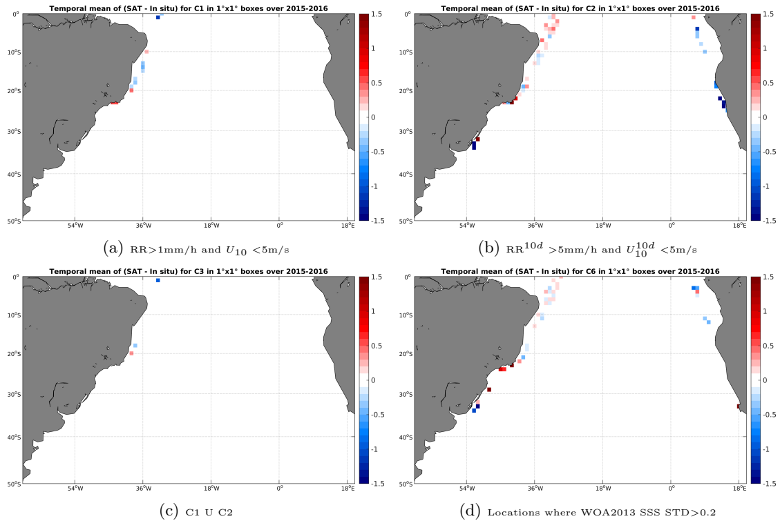
Figure 12: Temporal mean gridded over spatial boxes of size 1^\circ \times 1^\circ of \Delta SSS (SMAP-L3-RSS-V2-8DAY-RUNNING-40KM - TSG-LEGOS-DM) for 4 different subdatasets corresponding to: RR > 1mm/h and U_{10} < 5\text{m/s} (a), RR^{10d} > 5\text{mm/h} and U_{10}^{10d} < 5\text{m/s} (b), C1 U C2 (c), Locations where WOA2013 SSS STD > 0.2 (d).
