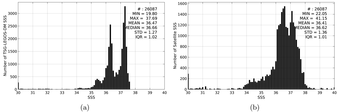
Figure 2: Histograms of SSS from TSG-LEGOS-DM (a) and SMAP-L3-RSS-V2-8DAY-RUNNING-40KM (b) considering all match-up pairs per bins of 0.1 over the South Atlantic Ocean Pi-MEP region and for the full satellite product period.
