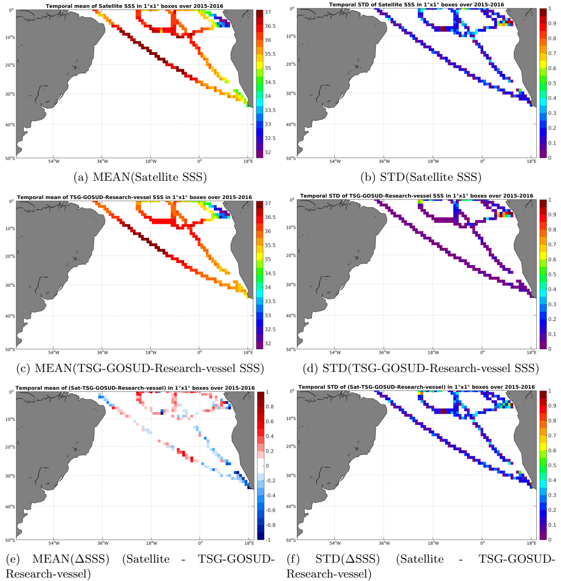
Figure 6: Temporal mean (left) and STD (right) of SSS from SMAP-L3-RSS-V2-8DAY-RUNNING-40KM (top), TSG-GOSUD-Research-vessel (middle), and of \Delta SSS (Satellite - TSG-GOSUD-Research-vessel). Only match-up pairs are used to generate these maps.
