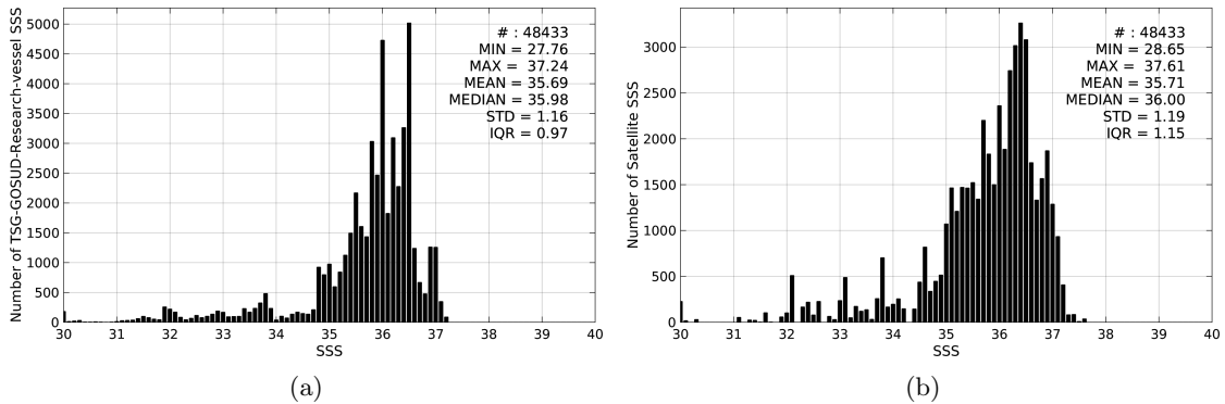
Figure 2: Histograms of SSS from TSG-GOSUD-Research-vessel (a) and SMAP-L3-RSS-V2-8DAY-RUNNING-40KM (b) considering all match-up pairs per bins of 0.1 over the South Atlantic Ocean Pi-MEP region and for the full satellite product period.
