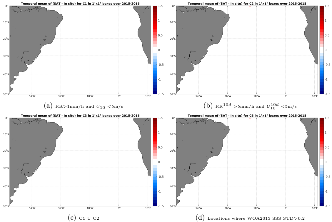
Figure 11: Temporal mean gridded over spatial boxes of size 1^\circ \times 1^\circ of \Delta SSS (SMAP-L3-RSS-V2-8DAY-RUNNING-40KM - Surface drifters) for 4 different subdatasets corresponding to: RR > 1\text{mm/h} and U_{10} < 5\text{m/s} (a), RR^{10d} > 5\text{mm/h} and U_{10}^{10d} < 5\text{m/s} (b), C1 U C2 (c), Locations where WOA2013 SSS STD > 0.2 (d).
