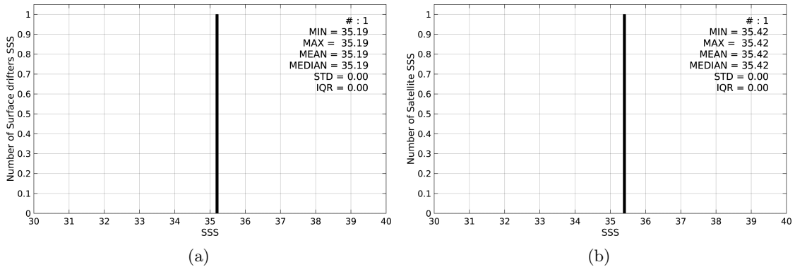
Figure 2: Histograms of SSS from Surface drifters (a) and SMAP-L3-RSS-V2-8DAY-RUNNING-40KM (b) considering all match-up pairs per bins of 0.1 over the South Atlantic Ocean Pi-MEP region and for the full satellite product period.
