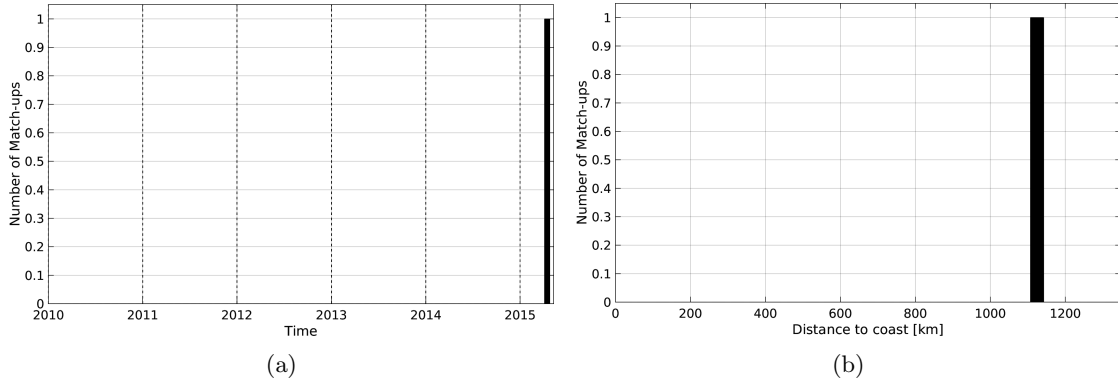
Figure 1: Number of match-ups between Surface drifters and SMAP-L3-RSS-V2-8DAY-RUNNING-40KM SSS as a function of time (a) and as function of the distance to coast (b) over the South Atlantic Ocean Pi-MEP region and for the full satellite product period.
