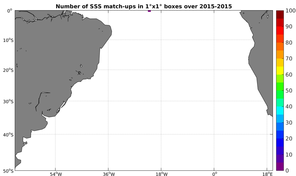
Figure 3: Number of SSS match-ups between Surface drifters SSS and the SMAP-L3-RSS-V2-8DAY-RUNNING-40KM SSS product for the South Atlantic Ocean Pi-MEP region over 1°x1° boxes and for the full satellite product period.
