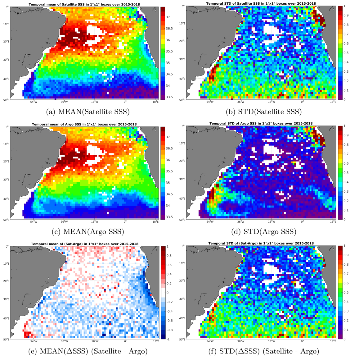
Figure 6: Temporal mean (left) and STD (right) of SSS from SMAP-L3-RSS-V2-8DAY-RUNNING-40KM (top), Argo (middle), and of \Delta SSS (Satellite - Argo). Only match-up pairs are used to generate these maps.
