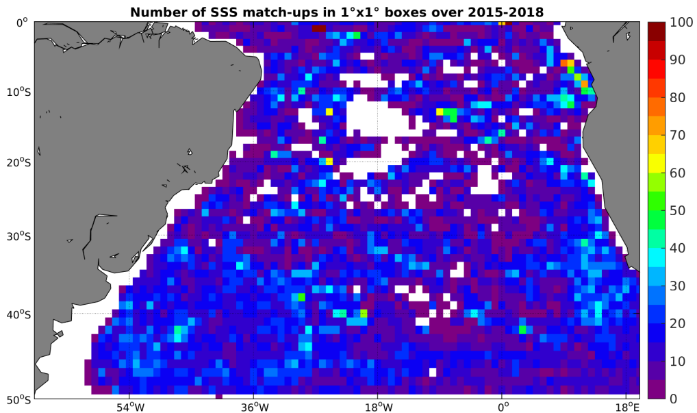
Figure 4: Number of SSS match-ups between Argo SSS and the SMAP-L3-RSS-V2-8DAY-RUNNING-40KM SSS product for the South Atlantic Ocean Pi-MEP region over 1^{\circ} \times 1^{\circ} boxes and for the full satellite product period.
