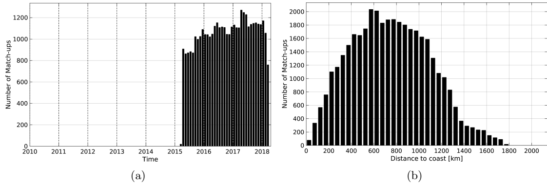
Figure 1: Number of match-ups between Argo and SMAP-L3-RSS-V2-8DAY-RUNNING-40KM SSS as a function of time (a) and as function of the distance to coast (b) over the South Atlantic Ocean Pi-MEP region and for the full satellite product period.
