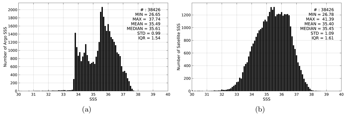
Figure 2: Histograms of SSS from Argo (a) and SMAP-L3-RSS-V2-8DAY-RUNNING-40KM (b) considering all match-up pairs per bins of 0.1 over the South Atlantic Ocean Pi-MEP region and for the full satellite product period.
