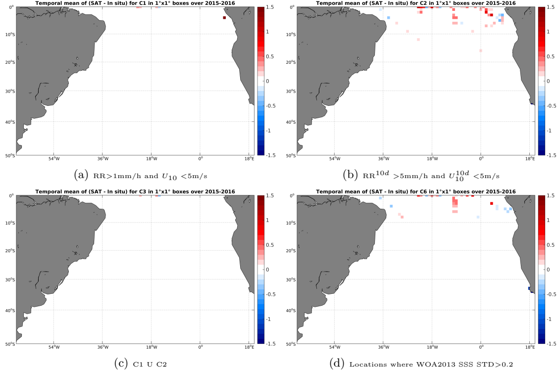
Figure 12: Temporal mean gridded over spatial boxes of size 1^\circ \times 1^\circ of \Delta SSS (SMAP-L3-RSS-V2-8DAY-RUNNING-70KM - TSG-GOSUD-Research-vessel) for 4 different subdatasets corresponding to: RR > 1\text{mm/h} and U_{10} < 5\text{m/s} (a), RR^{10d} > 5\text{mm/h} and U_{10}^{10d} < 5\text{m/s} (b), C1 U C2 (c), Locations where WOA2013 SSS STD > 0.2 (d).
