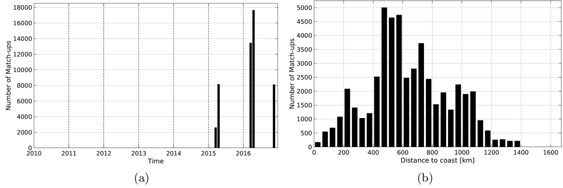
Figure 1: Number of match-ups between TSG-GOSUD-Research-vessel and SMAP-L3-RSS-V2-8DAY-RUNNING-70KM SSS as a function of time (a) and as function of the distance to coast (b) over the South Atlantic Ocean Pi-MEP region and for the full satellite product period.
