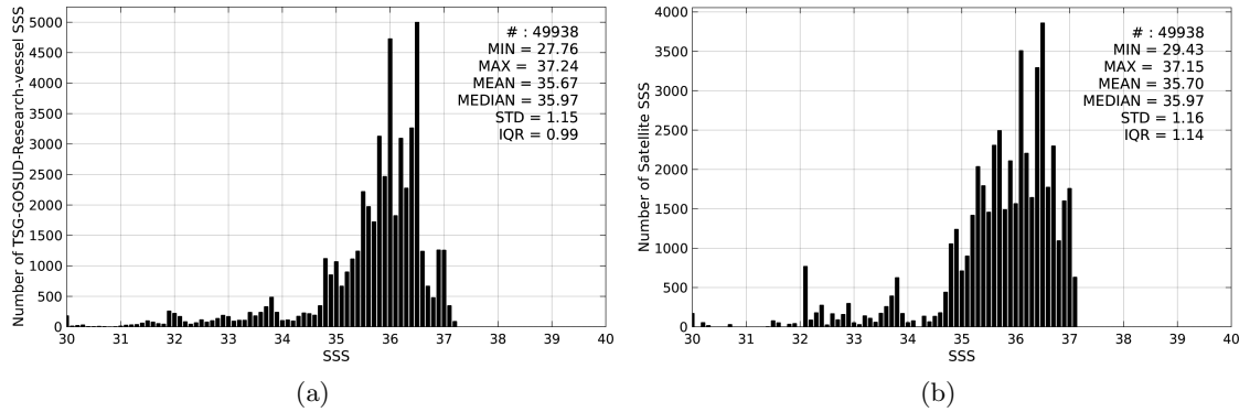
Figure 2: Histograms of SSS from TSG-GOSUD-Research-vessel (a) and SMAP-L3-RSS-V2-8DAY-RUNNING-70KM (b) considering all match-up pairs per bins of 0.1 over the South Atlantic Ocean Pi-MEP region and for the full satellite product period.
