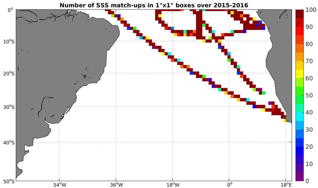
Figure 4: Number of SSS match-ups between TSG-GOSUD-Research-vessel SSS and the SMAP-L3-RSS-V2-8DAY-RUNNING-70KM SSS product for the South Atlantic Ocean Pi-MEP region over 1^\circ \times 1^\circ boxes and for the full satellite product period.
