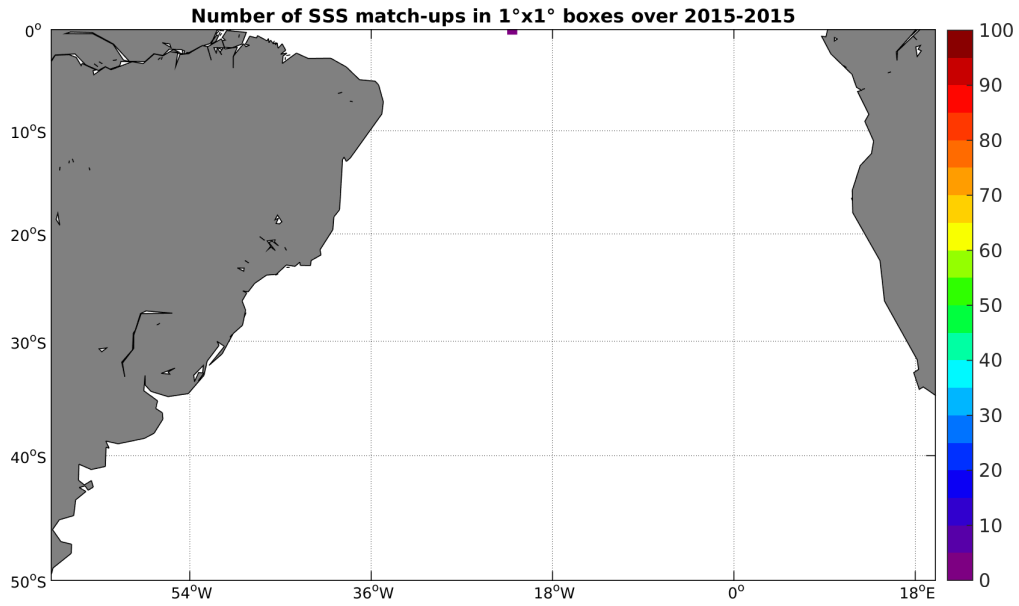
Figure 3: Number of SSS match-ups between Surface drifters SSS and the SMAP-L3-RSS-V2-8DAY-RUNNING-70KM SSS product for the South Atlantic Ocean Pi-MEP region over 1^\circ \times 1^\circ boxes and for the full satellite product period.
