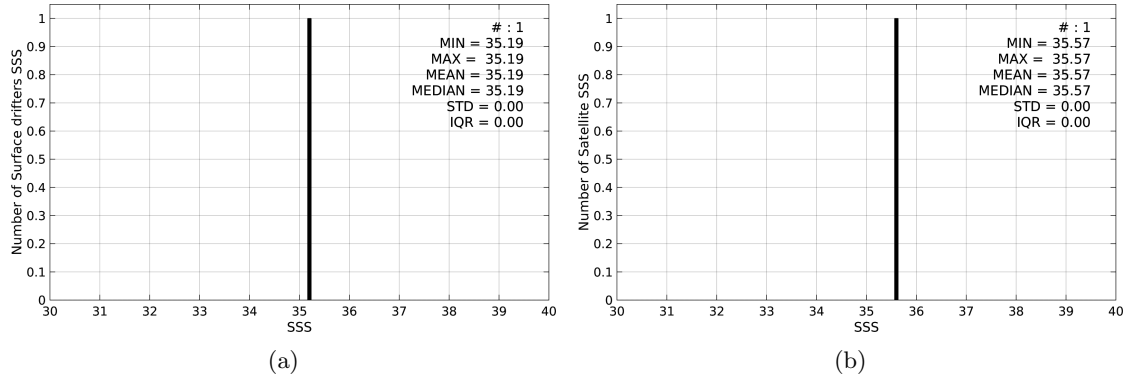
Figure 2: Histograms of SSS from Surface drifters (a) and SMAP-L3-RSS-V2-8DAY-RUNNING-70KM (b) considering all match-up pairs per bins of 0.1 over the South Atlantic Ocean Pi-MEP region and for the full satellite product period.
