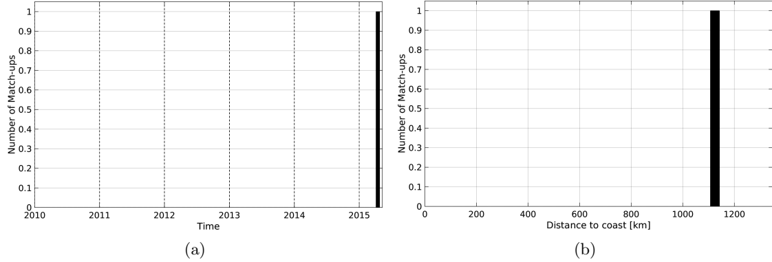
Figure 1: Number of match-ups between Surface drifters and SMAP-L3-RSS-V2-8DAY-RUNNING-70KM SSS as a function of time (a) and as function of the distance to coast (b) over the South Atlantic Ocean Pi-MEP region and for the full satellite product period.
