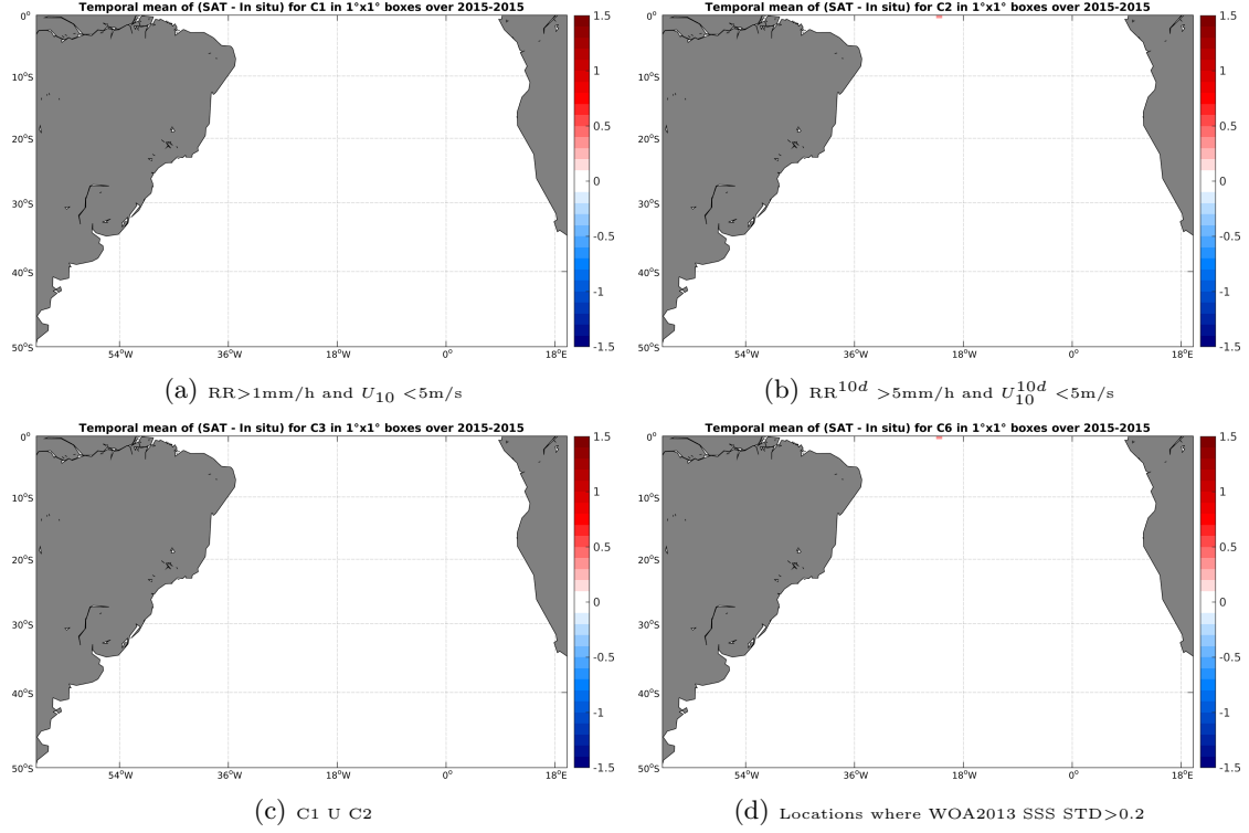
Figure 11: Temporal mean gridded over spatial boxes of size 1^\circ \times 1^\circ of \Delta SSS (SMAP-L3-RSS-V2-8DAY-RUNNING-70KM - Surface drifters) for 4 different subdatasets corresponding to: RR > 1\text{mm/h} and U_{10} < 5\text{m/s} (a), RR^{10d} > 5\text{mm/h} and U_{10}^{10d} < 5\text{m/s} (b), C1 U C2 (c), Locations where WOA2013 SSS STD > 0.2 (d).
