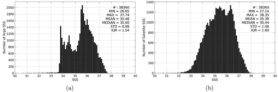
Figure 2: Histograms of SSS from Argo (a) and SMAP-L3-RSS-V2-8DAY-RUNNING-70KM (b) considering all match-up pairs per bins of 0.1 over the South Atlantic Ocean Pi-MEP region and for the full satellite product period.
