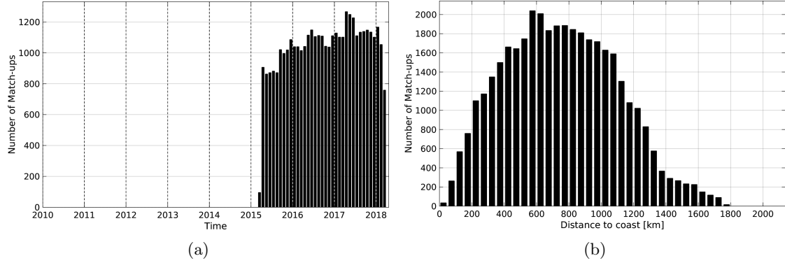
Figure 1: Number of match-ups between Argo and SMAP-L3-RSS-V2-8DAY-RUNNING-70KM SSS as a function of time (a) and as function of the distance to coast (b) over the South Atlantic Ocean Pi-MEP region and for the full satellite product period.
