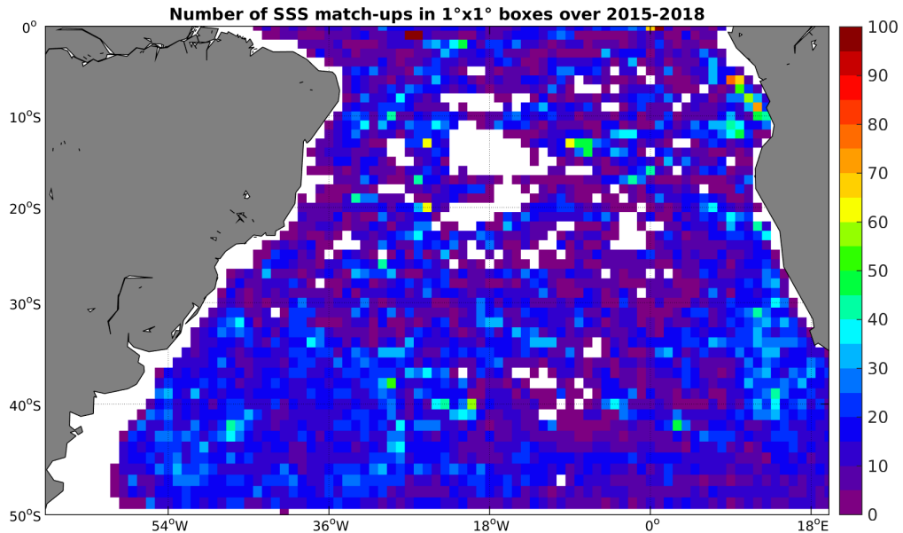
Figure 4: Number of SSS match-ups between Argo SSS and the SMAP-L3-RSS-V2-8DAY-RUNNING-70KM SSS product for the South Atlantic Ocean Pi-MEP region over 1^\circ \times 1^\circ boxes and for the full satellite product period.
