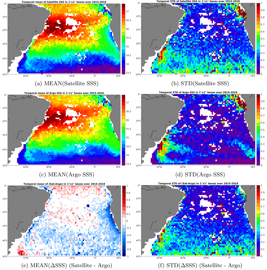
Figure 6: Temporal mean (left) and STD (right) of SSS from SMAP-L3-RSS-V2-8DAY-RUNNING-70KM (top), Argo (middle), and of \Delta SSS (Satellite - Argo). Only match-up pairs are used to generate these maps.
