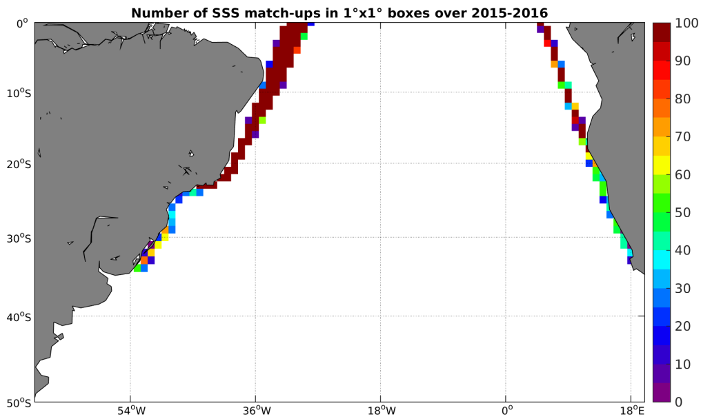
Figure 4: Number of SSS match-ups between TSG-LEGOS-DM SSS and the SMAP-L3-RSS-V2-MONTHLY-0.25DEG-40KM SSS product for the South Atlantic Ocean Pi-MEP region over 1^\circ \times 1^\circ boxes and for the full satellite product period.
