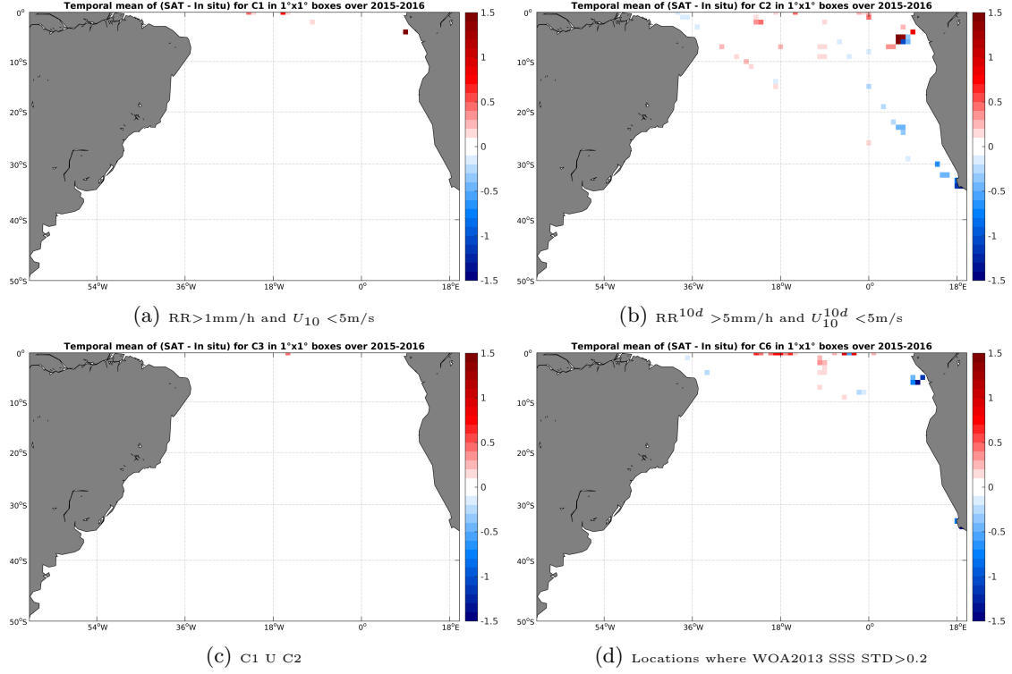
Figure 12: Temporal mean gridded over spatial boxes of size 1^\circ \times 1^\circ of \Delta SSS (SMAP-L3-RSS-V2-MONTHLY-0.25DEG-40KM - TSG-GOSUD-Research-vessel) for 4 different subdatasets corresponding to: RR > 1mm/h and U_{10} < 5 m/s (a), RR^{10d} > 5 mm/h and U_{10}^{10d} < 5 m/s (b), C1 U C2 (c), Locations where WOA2013 SSS STD > 0.2 (d).
