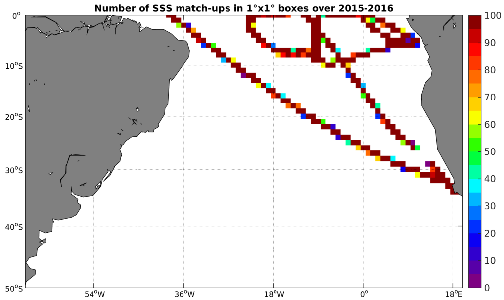
Figure 4: Number of SSS match-ups between TSG-GOSUD-Research-vessel SSS and the SMAP-L3-RSS-V2-MONTHLY-0.25DEG-40KM SSS product for the South Atlantic Ocean Pi-MEP region over 1^\circ \times 1^\circ boxes and for the full satellite product period.
