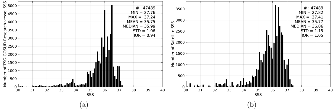
Figure 2: Histograms of SSS from TSG-GOSUD-Research-vessel (a) and SMAP-L3-RSS-V2-MONTHLY-0.25DEG-40KM (b) considering all match-up pairs per bins of 0.1 over the South Atlantic Ocean Pi-MEP region and for the full satellite product period.
