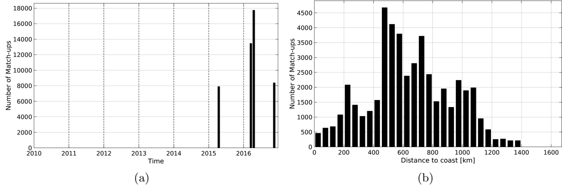
Figure 1: Number of match-ups between TSG-GOSUD-Research-vessel and SMAP-L3-RSS-V2-MONTHLY-0.25DEG-40KM SSS as a function of time (a) and as function of the distance to coast (b) over the South Atlantic Ocean Pi-MEP region and for the full satellite product period.
