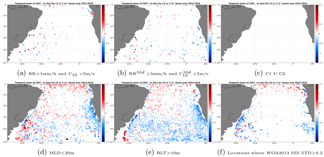
Figure 12: Temporal mean gridded over spatial boxes of size 1^\circ \times 1^\circ of \Delta SSS (SMAP-L3-RSS-V2-MONTHLY-0.25DEG-40KM - Argo) for 6 different subdatasets corresponding to: RR > 1\text{mm/h} and U_{10} < 5\text{m/s} (a), RR^{10d} > 5\text{mm/h} and U_{10}^{10d} < 5\text{m/s} (b), C1 U C2 (c), MLD < 20\text{m} (d), BLT > 10\text{m} (e), Locations where WOA2013 SSS STD > 0.2 (f).
