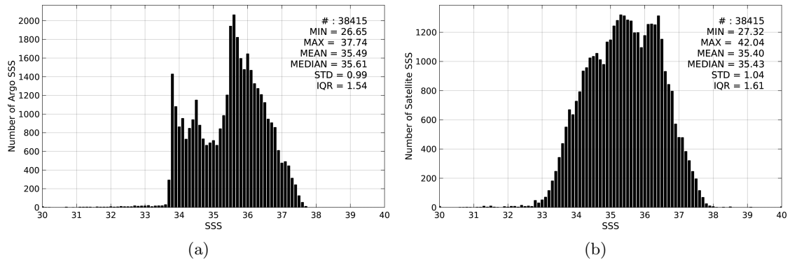
Figure 2: Histograms of SSS from Argo (a) and SMAP-L3-RSS-V2-MONTHLY-0.25DEG-40KM (b) considering all match-up pairs per bins of 0.1 over the South Atlantic Ocean Pi-MEP region and for the full satellite product period.
