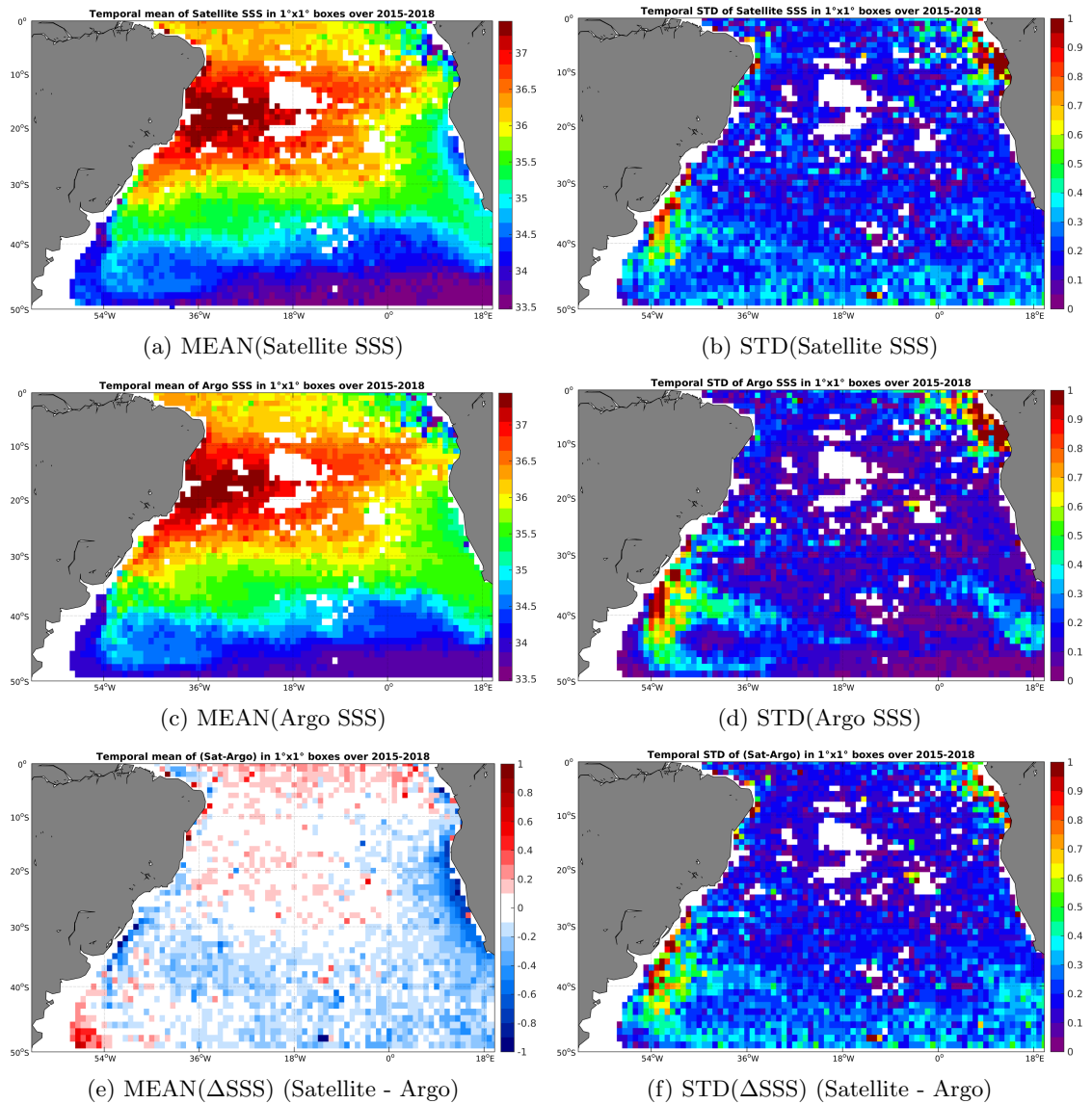
Figure 6: Temporal mean (left) and STD (right) of SSS from SMAP-L3-RSS-V2-MONTHLY-0.25DEG-40KM (top), Argo (middle), and of \Delta SSS (Satellite - Argo). Only match-up pairs are used to generate these maps.
