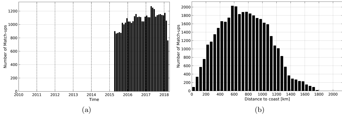
Figure 1: Number of match-ups between Argo and SMAP-L3-RSS-V2-MONTHLY-0.25DEG-40KM SSS as a function of time (a) and as function of the distance to coast (b) over the South Atlantic Ocean Pi-MEP region and for the full satellite product period.
