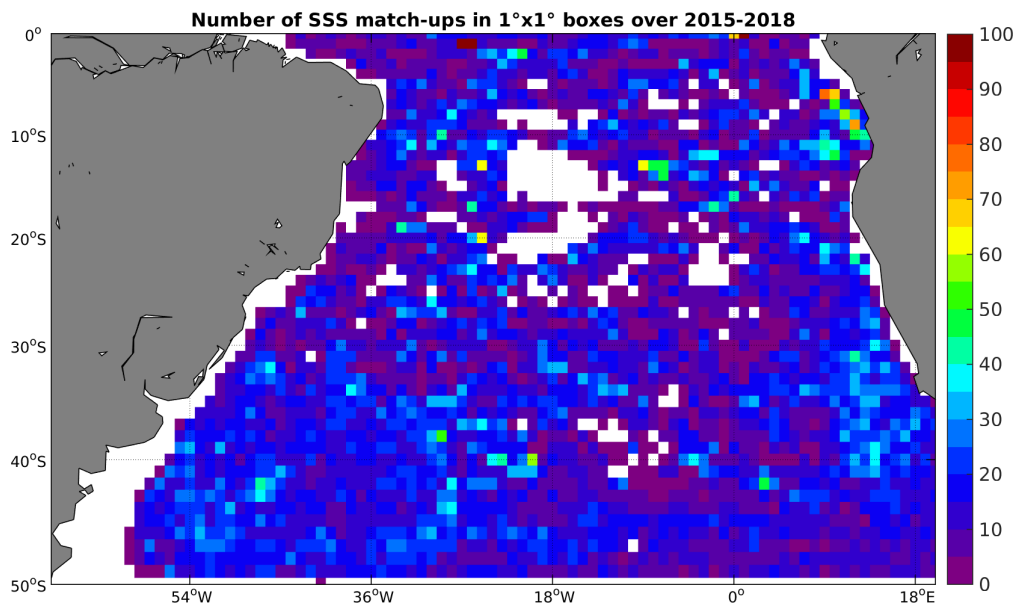
Figure 4: Number of SSS match-ups between Argo SSS and the SMAP-L3-RSS-V2-MONTHLY-0.25DEG-40KM SSS product for the South Atlantic Ocean Pi-MEP region over 1^\circ \times 1^\circ boxes and for the full satellite product period.
