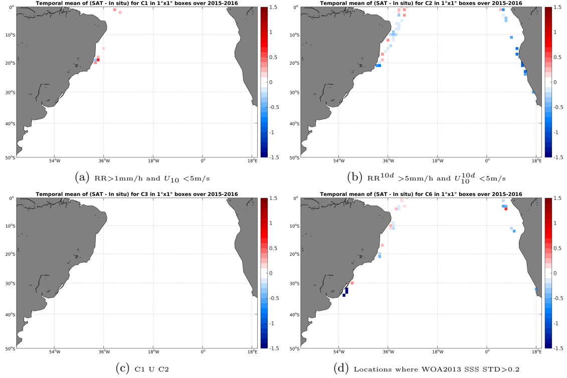
Figure 12: Temporal mean gridded over spatial boxes of size 1^\circ \times 1^\circ of \Delta SSS (SMAP-L3-RSS-V2-MONTHLY-70KM - TSG-LEGOS-DM) for 4 different subdatasets corresponding to: RR > 1 mm/h and U_{10} < 5 m/s (a), RR^{10d} > 5 mm/h and U_{10}^{10d} < 5 m/s (b), C1 U C2 (c), Locations where WOA2013 SSS STD > 0.2 (d).
