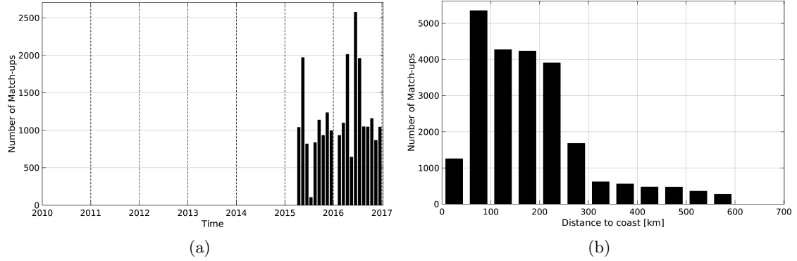
Figure 1: Number of match-ups between TSG-LEGOS-DM and SMAP-L3-RSS-V2-MONTHLY-70KM SSS as a function of time (a) and as function of the distance to coast (b) over the South Atlantic Ocean Pi-MEP region and for the full satellite product period.
