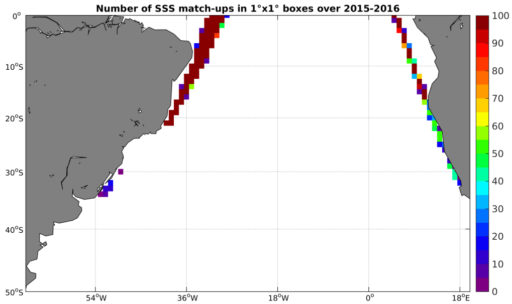
Figure 4: Number of SSS match-ups between TSG-LEGOS-DM SSS and the SMAP-L3-RSS-V2-MONTHLY-70KM SSS product for the South Atlantic Ocean Pi-MEP region over 1^\circ \times 1^\circ boxes and for the full satellite product period.
