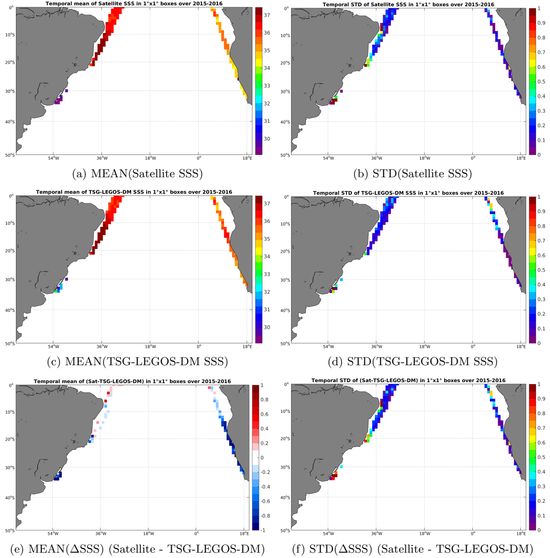
Figure 6: Temporal mean (left) and STD (right) of SSS from SMAP-L3-RSS-V2-MONTHLY-70KM (top), TSG-LEGOS-DM (middle), and of \Delta SSS (Satellite - TSG-LEGOS-DM). Only match-up pairs are used to generate these maps.
