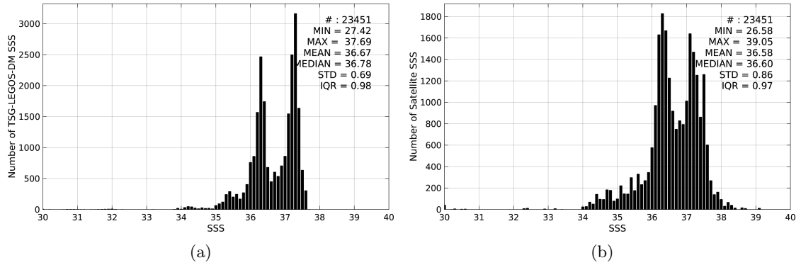
Figure 2: Histograms of SSS from TSG-LEGOS-DM (a) and SMAP-L3-RSS-V2-MONTHLY-70KM (b) considering all match-up pairs per bins of 0.1 over the South Atlantic Ocean Pi-MEP region and for the full satellite product period.
