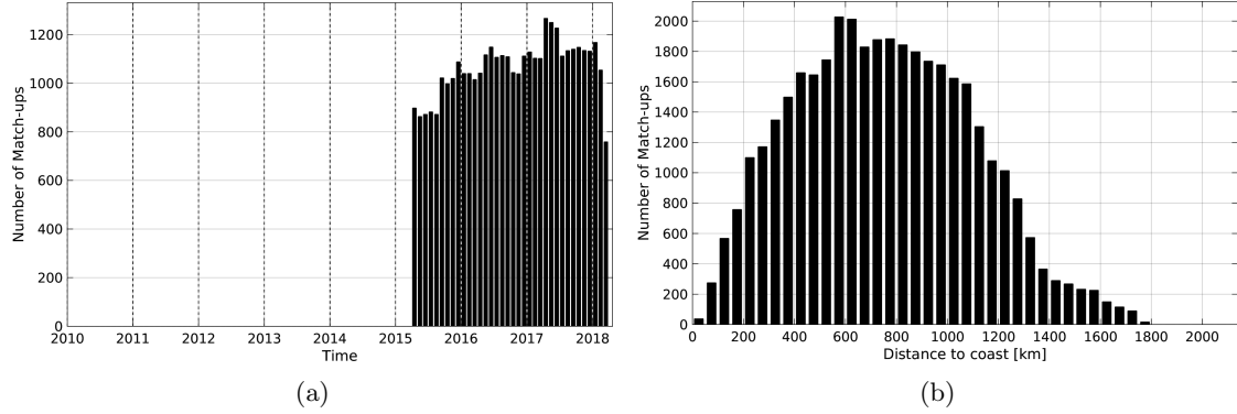
Figure 1: Number of match-ups between Argo and SMAP-L3-RSS-V2-MONTHLY-70KM SSS as a function of time (a) and as function of the distance to coast (b) over the South Atlantic Ocean Pi-MEP region and for the full satellite product period.
