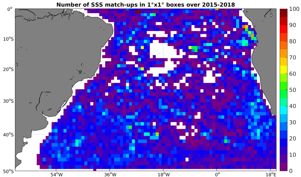
Figure 4: Number of SSS match-ups between Argo SSS and the SMAP-L3-RSS-V2-MONTHLY-70KM SSS product for the South Atlantic Ocean Pi-MEP region over 1^\circ \times 1^\circ boxes and for the full satellite product period.
