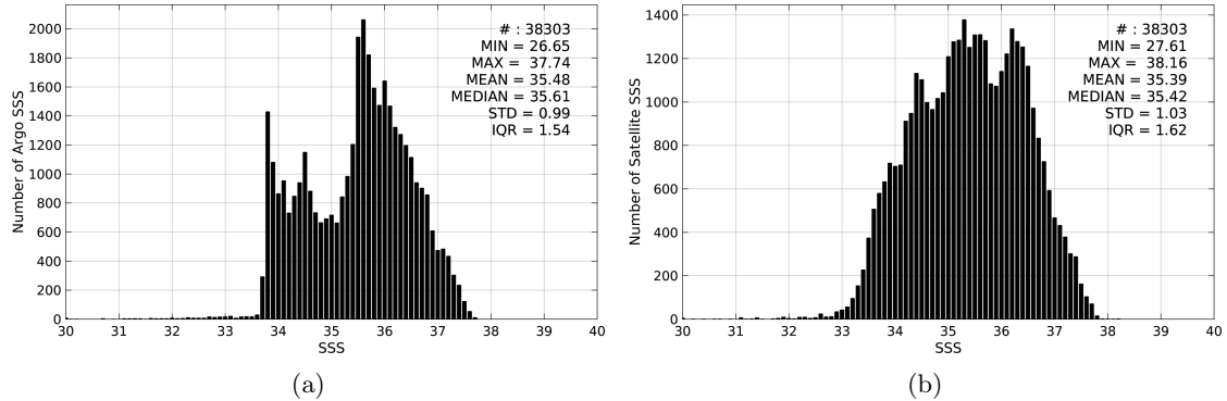
Figure 2: Histograms of SSS from Argo (a) and SMAP-L3-RSS-V2-MONTHLY-70KM (b) considering all match-up pairs per bins of 0.1 over the South Atlantic Ocean Pi-MEP region and for the full satellite product period.
