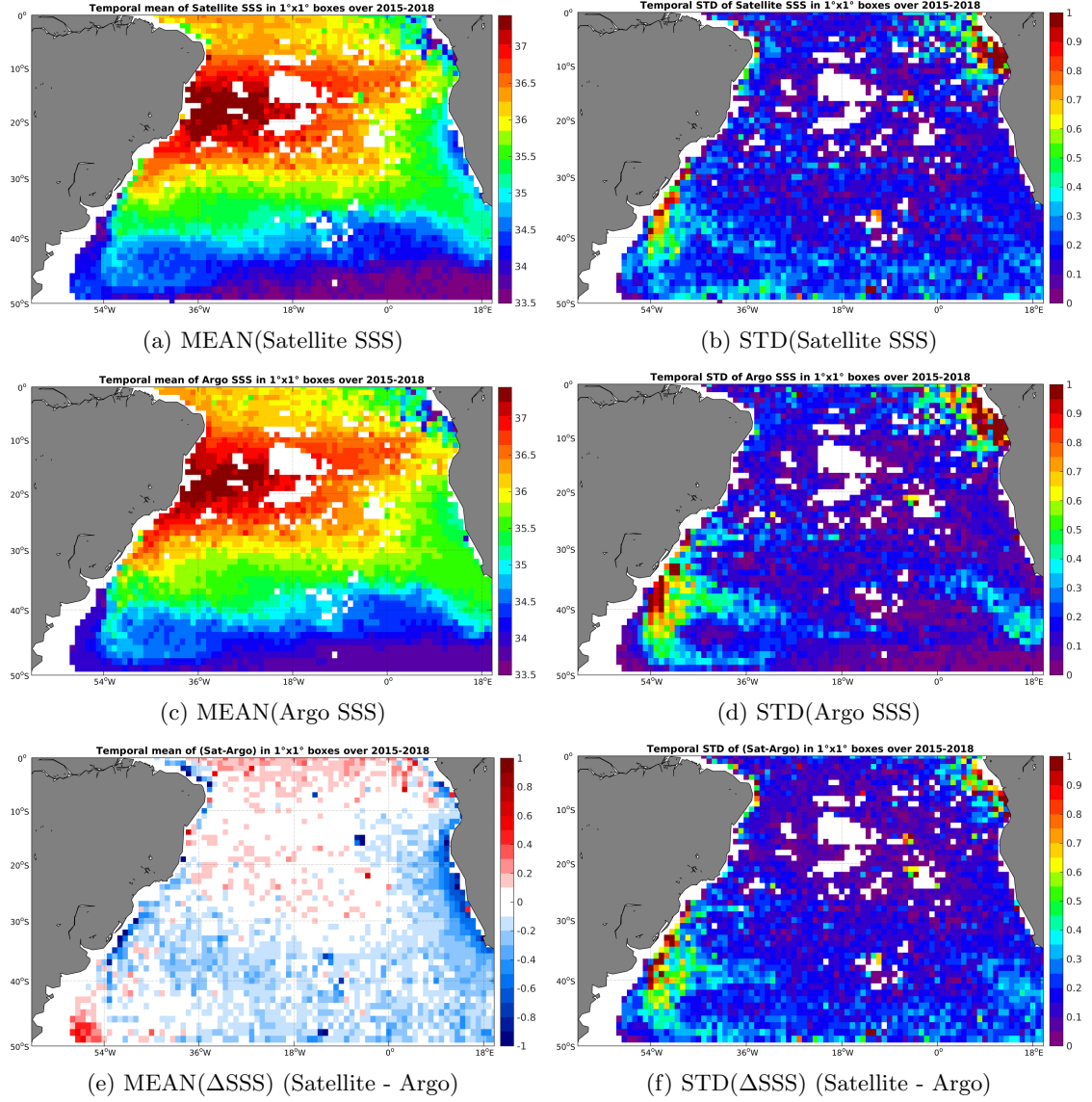
Figure 6: Temporal mean (left) and STD (right) of SSS from SMAP-L3-RSS-V2-MONTHLY-70KM (top), Argo (middle), and of \Delta SSS (Satellite - Argo). Only match-up pairs are used to generate these maps.
