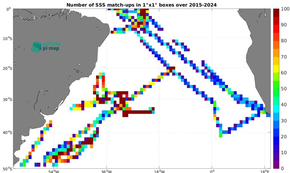
Figure 5: Number of SSS match-ups between TSG (SAMOS) SSS and the SMAP SSS L3 v5.0 - 8-Day running (JPL) SSS product for the South Atlantic Ocean Pi-MEP region over 1^\circ \times 1^\circ boxes and for the full satellite product period.
