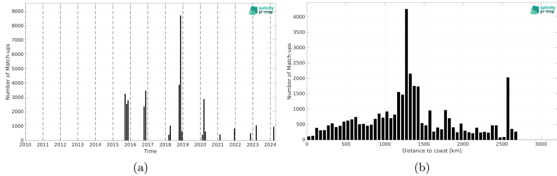
Figure 2: Number of match-ups between TSG (SAMOS) and SMAP SSS L3 v5.0 - 8-Day running (JPL) SSS as a function of time (a) and as function of the distance to coast (b) over the South Atlantic Ocean Pi-MEP region and for the full satellite product period.
