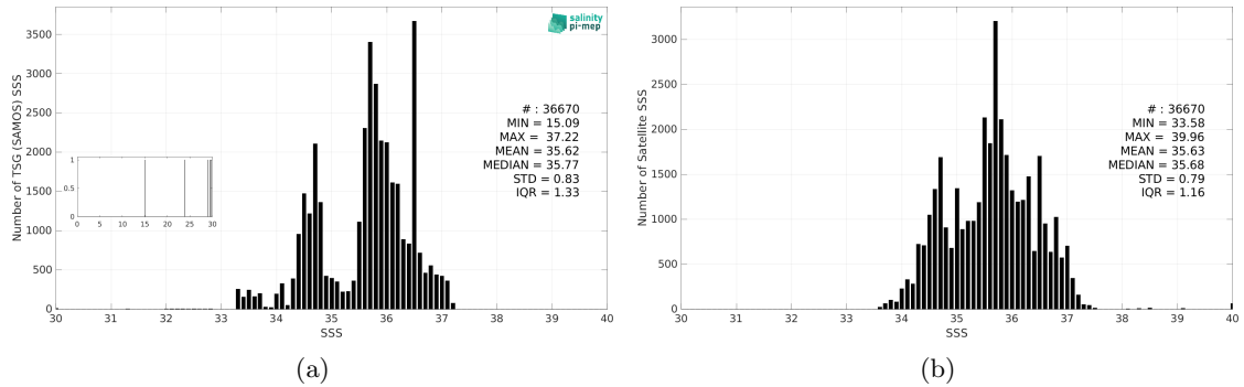
Figure 3: Histograms of SSS from TSG (SAMOS) (a) and SMAP SSS L3 v5.0 - 8-Day running (JPL) (b) considering all match-up pairs per bins of 0.1 over the South Atlantic Ocean Pi-MEP region and for the full satellite product period.
