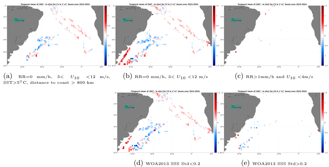
Figure 14: Temporal mean gridded over spatial boxes of size 1^\circ \times 1^\circ of \Delta\text{SSS} (SMAP SSS L3 v5.0 - 8-Day running (JPL) - TSG (SAMOS)) for 5 different subdatasets corresponding to:RR=0 mm/h, 3 < U_{10} < 12 m/s, SST >5^\circ\text{C} , distance to coast > 800 km (a), RR=0 mm/h, 3 < U_{10} < 12 m/s (b), RR >1 mm/h and U_{10} < 4 m/s (c), WOA2013 SSS Std <0.2 (d), WOA2013 SSS Std >0.2 (e).
