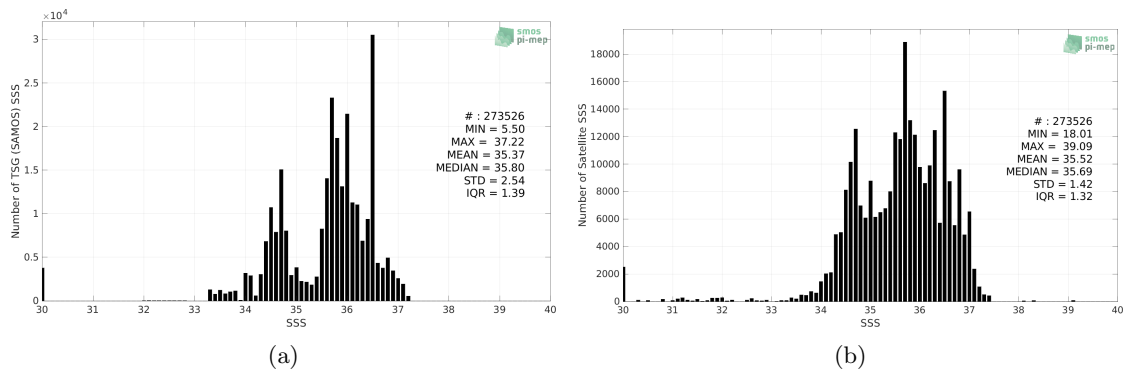
Figure 2: Histograms of SSS from TSG (SAMOS) (a) and SMAP SSS L3 v5.0 - 8-Day running (JPL) (b) considering all match-up pairs per bins of 0.1 over the South Atlantic Ocean Pi-MEP region and for the full satellite product period.
