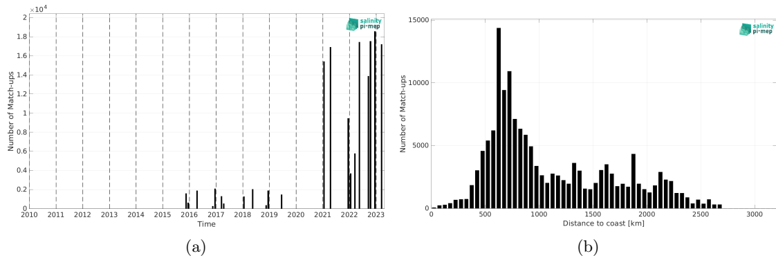
Figure 2: Number of match-ups between TSG (Polarstern) and SMAP SSS L3 v5.0 - 8-Day running (JPL) SSS as a function of time (a) and as function of the distance to coast (b) over the South Atlantic Ocean Pi-MEP region and for the full satellite product period.
