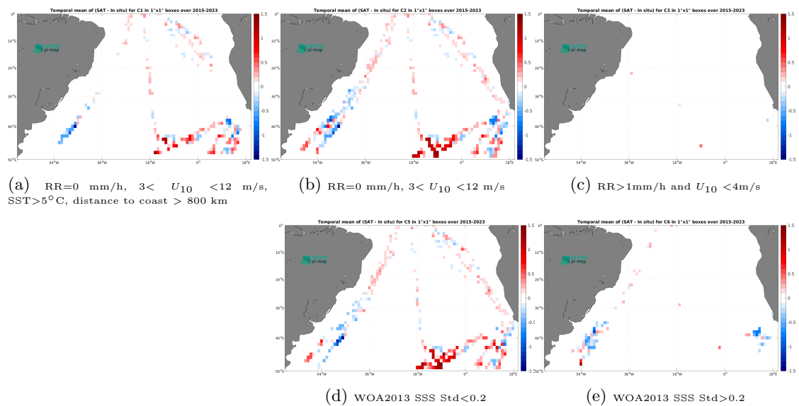
Figure 14: Temporal mean gridded over spatial boxes of size 1^\circ \times 1^\circ of \Delta\text{SSS} (SMAP SSS L3 v5.0 - 8-Day running (JPL) - TSG (Polarstern)) for 5 different subdatasets corresponding to:RR=0 mm/h, 3 < U_{10} < 12 m/s, SST >5^\circ\text{C} , distance to coast > 800 km (a), RR=0 mm/h, 3 < U_{10} < 12 m/s (b), RR >1 mm/h and U_{10} < 4 m/s (c), WOA2013 SSS Std <0.2 (d), WOA2013 SSS Std >0.2 (e).
