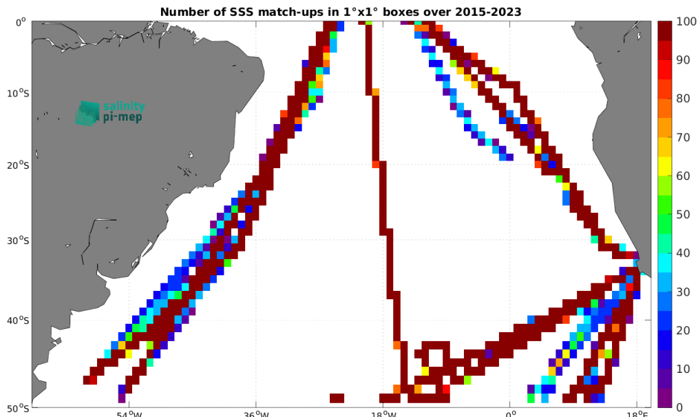
Figure 5: Number of SSS match-ups between TSG (Polarstern) SSS and the SMAP SSS L3 v5.0 - 8-Day running (JPL) SSS product for the South Atlantic Ocean Pi-MEP region over 1^\circ \times 1^\circ boxes and for the full satellite product period.
