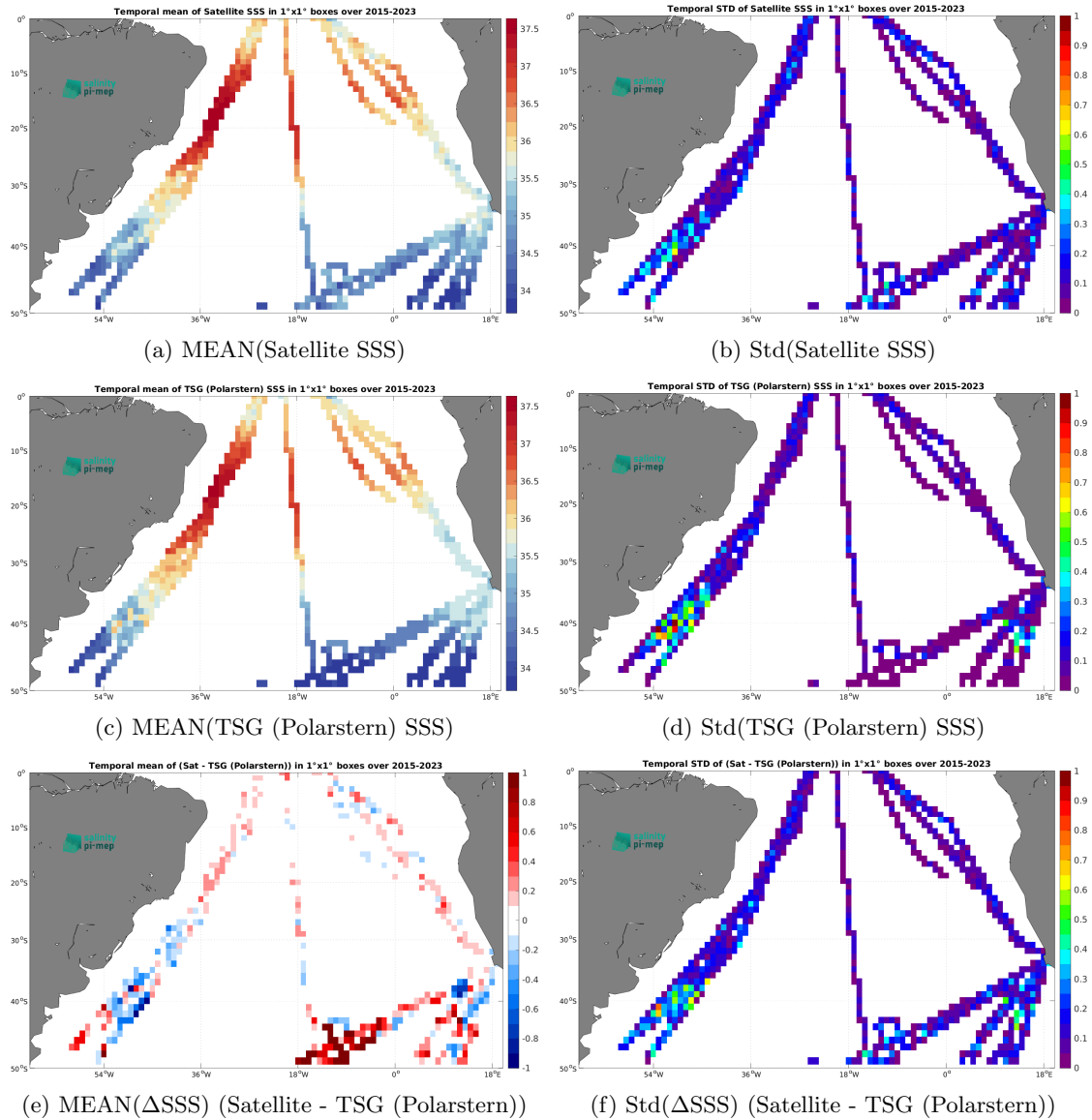
Figure 7: Temporal mean (left) and Std (right) of SSS from SMAP SSS L3 v5.0 - 8-Day running (JPL) (top), TSG (Polarstern) (middle), and of \Delta SSS (Satellite - TSG (Polarstern)). Only match-up pairs are used to generate these maps.
