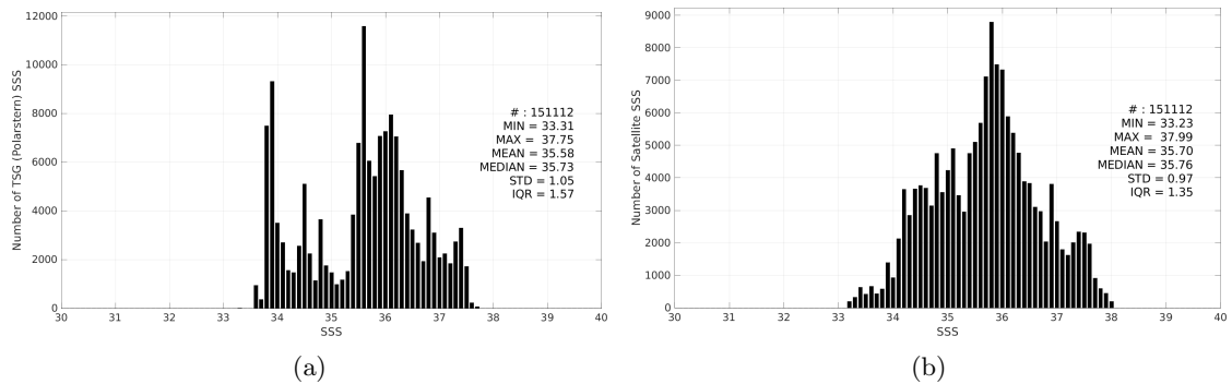
Figure 3: Histograms of SSS from TSG (Polarstern) (a) and SMAP SSS L3 v5.0 - 8-Day running (JPL) (b) considering all match-up pairs per bins of 0.1 over the South Atlantic Ocean Pi-MEP region and for the full satellite product period.
