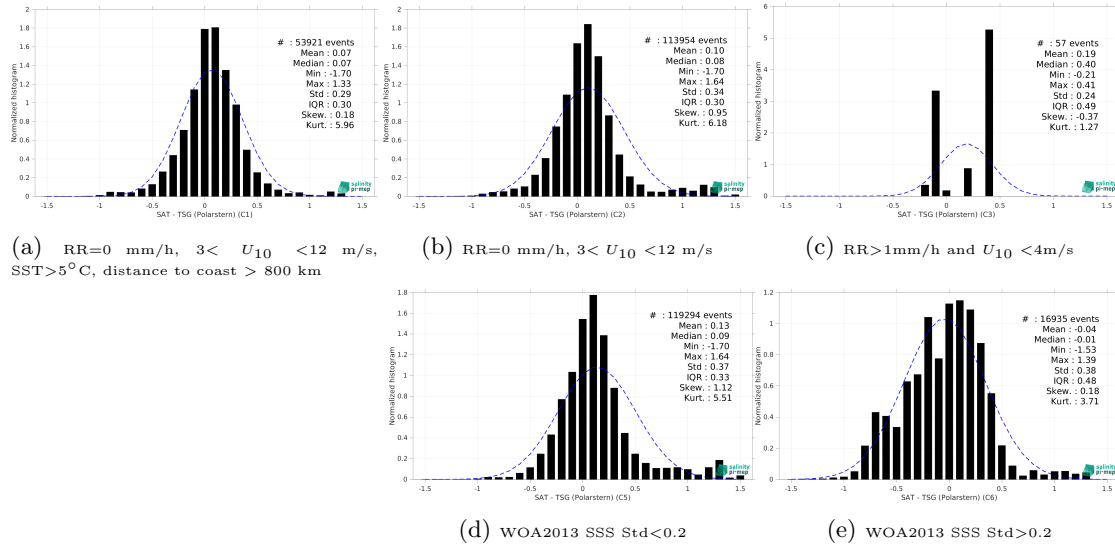
Figure 15: Normalized histogram of \Delta\text{SSS} (SMAP SSS L3 v5.0 - 8-Day running (JPL) - TSG (Polarstern)) for 5 different subdatasets corresponding to: RR=0 mm/h, 3 < U_{10} < 12 m/s, SST>5°C, distance to coast > 800 km (a), RR=0 mm/h, 3 < U_{10} < 12 m/s (b), RR>1mm/h and U_{10} < 4 m/s (c), WOA2013 SSS Std<0.2 (d), WOA2013 SSS Std>0.2 (e).
