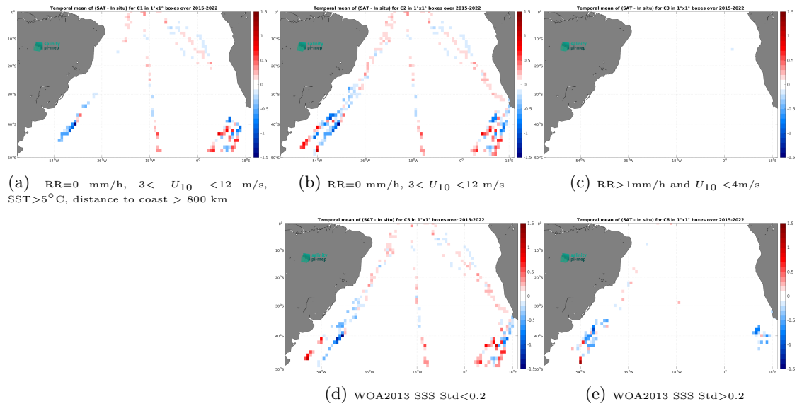
Figure 12: Temporal mean gridded over spatial boxes of size 1^\circ \times 1^\circ of \Delta\text{SSS} (SMAP SSS L3 v5.0 - 8-Day running (JPL) - TSG (Polarstern)) for 5 different subdatasets corresponding to:RR=0 mm/h, 3 < U_{10} < 12 m/s, SST >5^\circ\text{C} , distance to coast > 800 km (a), RR=0 mm/h, 3 < U_{10} < 12 m/s (b), RR >1 mm/h and U_{10} < 4 m/s (c), WOA2013 SSS Std <0.2 (d), WOA2013 SSS Std >0.2 (e).
