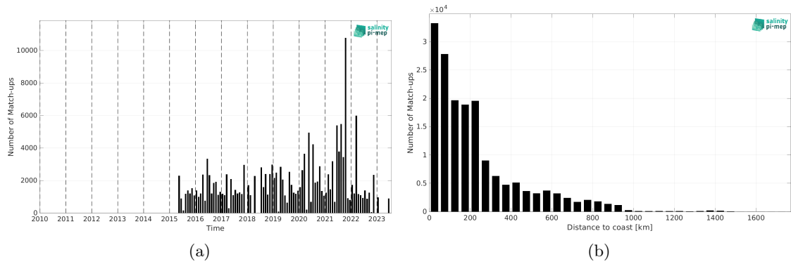
Figure 2: Number of match-ups between TSG (LEGOS-DM) and SMAP SSS L3 v5.0 - 8-Day running (JPL) SSS as a function of time (a) and as function of the distance to coast (b) over the South Atlantic Ocean Pi-MEP region and for the full satellite product period.
