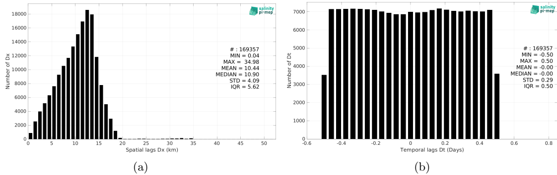
Figure 6: Histograms of the spatial (a) and temporal (b) lags between the location/time of the TSG (LEGOS-DM) measurement and the date of the corresponding SMAP SSS L3 v5.0 - 8-Day running (JPL) SSS pixel.
