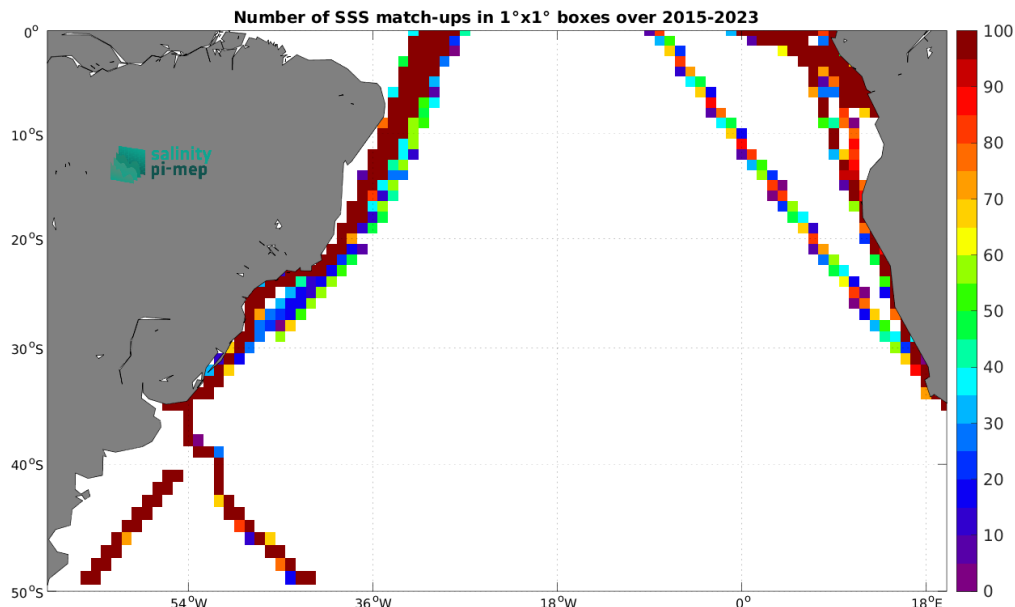
Figure 5: Number of SSS match-ups between TSG (LEGOS-DM) SSS and the SMAP SSS L3 v5.0 - 8-Day running (JPL) SSS product for the South Atlantic Ocean Pi-MEP region over 1^\circ \times 1^\circ boxes and for the full satellite product period.
