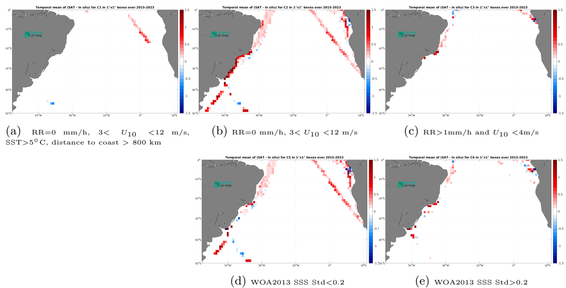
Figure 14: Temporal mean gridded over spatial boxes of size 1^\circ \times 1^\circ of \Delta SSS (SMAP SSS L3 v5.0 - 8-Day running (JPL) - TSG (LEGOS-DM)) for 5 different subdatasets corresponding to:RR=0 mm/h, 3 < U_{10} < 12 m/s, SST >5^\circ\text{C} , distance to coast > 800 km (a), RR=0 mm/h, 3 < U_{10} < 12 m/s (b), RR >1 mm/h and U_{10} < 4 m/s (c), WOA2013 SSS Std <0.2 (d), WOA2013 SSS Std >0.2 (e).
