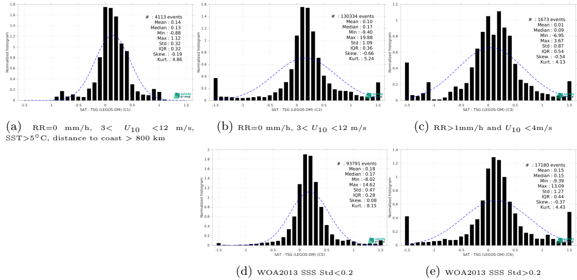
Figure 15: Normalized histogram of \Delta\text{SSS} (SMAP SSS L3 v5.0 - 8-Day running (JPL) - TSG (LEGOS-DM)) for 5 different subdatasets corresponding to: RR=0 mm/h, 3 < U_{10} < 12 m/s, SST>5°C, distance to coast > 800 km (a), RR=0 mm/h, 3 < U_{10} < 12 m/s (b), RR>1mm/h and U_{10} < 4 m/s (c), WOA2013 SSS Std<0.2 (d), WOA2013 SSS Std>0.2 (e).
