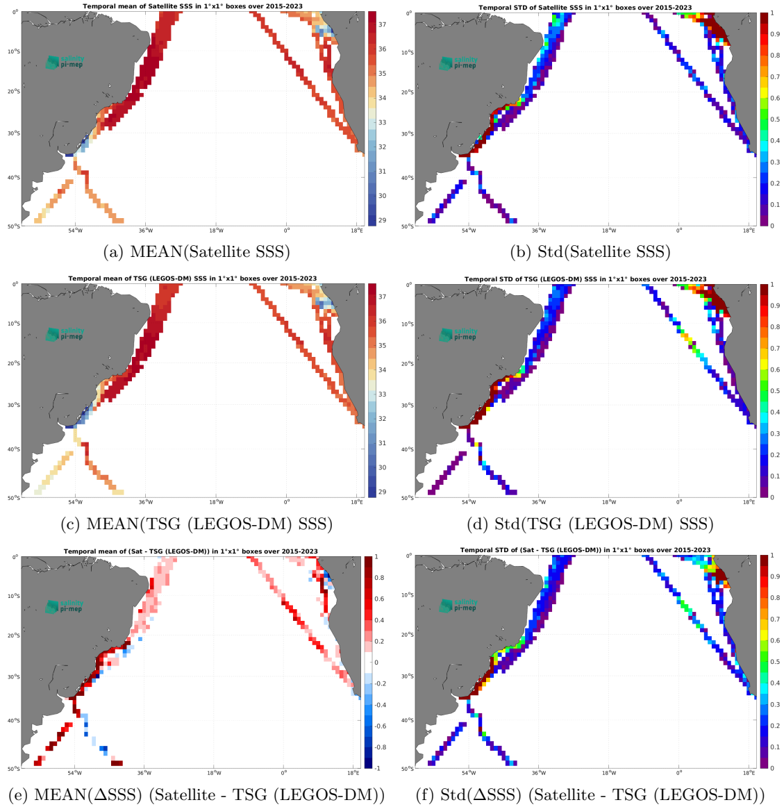
Figure 7: Temporal mean (left) and Std (right) of SSS from SMAP SSS L3 v5.0 - 8-Day running (JPL) (top), TSG (LEGOS-DM) (middle), and of \Delta SSS (Satellite - TSG (LEGOS-DM)). Only match-up pairs are used to generate these maps.
