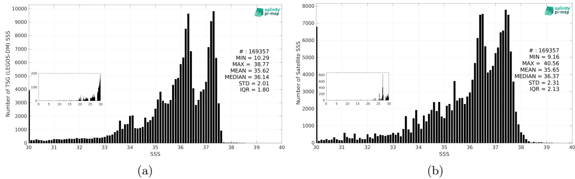
Figure 3: Histograms of SSS from TSG (LEGOS-DM) (a) and SMAP SSS L3 v5.0 - 8-Day running (JPL) (b) considering all match-up pairs per bins of 0.1 over the South Atlantic Ocean Pi-MEP region and for the full satellite product period.
