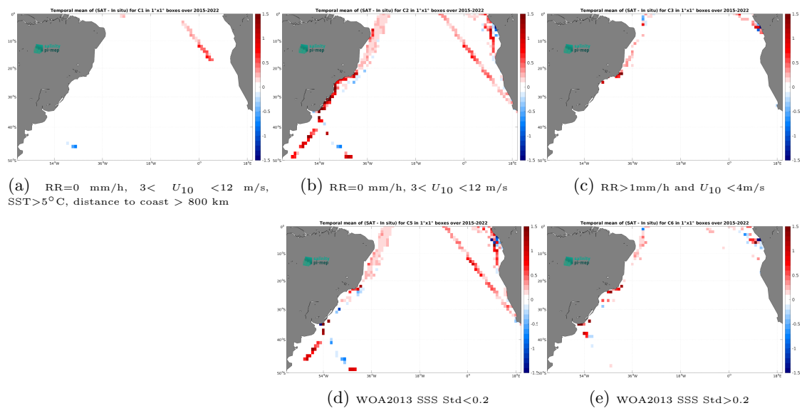
Figure 14: Temporal mean gridded over spatial boxes of size 1^\circ \times 1^\circ of \Delta\text{SSS} (SMAP SSS L3 v5.0 - 8-Day running (JPL) - TSG (LEGOS-DM)) for 5 different subdatasets corresponding to:RR=0 mm/h, 3 < U_{10} < 12 m/s, SST > 5°C, distance to coast > 800 km (a), RR=0 mm/h, 3 < U_{10} < 12 m/s (b), RR > 1mm/h and U_{10} < 4 m/s (c), WOA2013 SSS Std < 0.2 (d), WOA2013 SSS Std > 0.2 (e).
