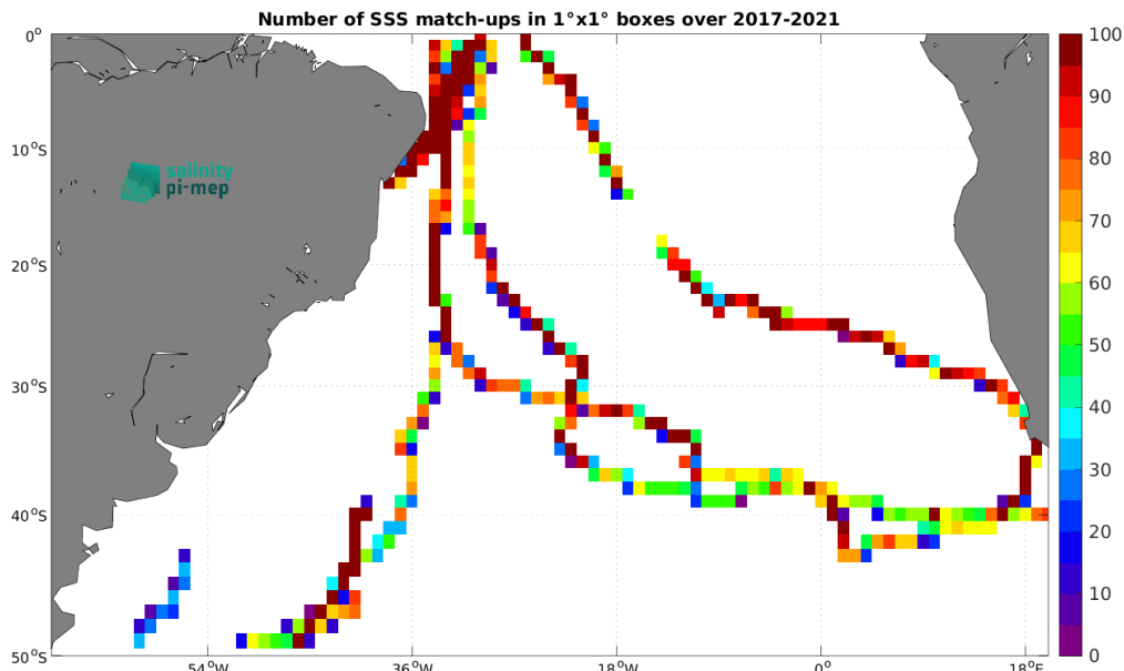
Figure 5: Number of SSS match-ups between TSG (GOSUD-Sailing-ship) SSS and the SMAP SSS L3 v5.0 - 8-Day running (JPL) SSS product for the South Atlantic Ocean Pi-MEP region over 1^\circ \times 1^\circ boxes and for the full satellite product period.
