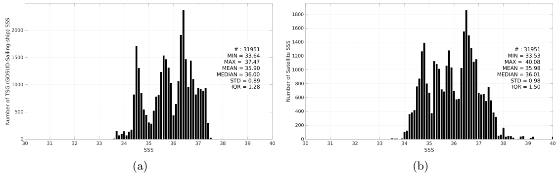
Figure 3: Histograms of SSS from TSG (GOSUD-Sailing-ship) (a) and SMAP SSS L3 v5.0 - 8-Day running (JPL) (b) considering all match-up pairs per bins of 0.1 over the South Atlantic Ocean Pi-MEP region and for the full satellite product period.
