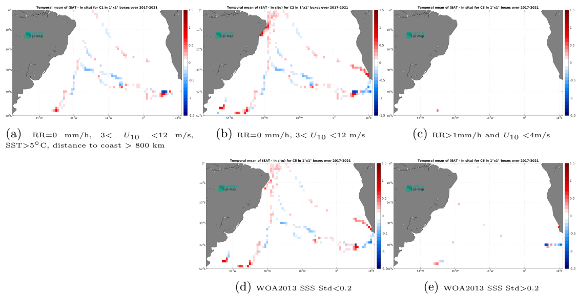
Figure 14: Temporal mean gridded over spatial boxes of size 1^\circ \times 1^\circ of \Delta\text{SSS} (SMAP SSS L3 v5.0 - 8-Day running (JPL) - TSG (GOSUD-Sailing-ship)) for 5 different subdatasets corresponding to:RR=0 mm/h, 3 < U_{10} < 12 m/s, SST >5^\circ\text{C} , distance to coast > 800 km (a), RR=0 mm/h, 3 < U_{10} < 12 m/s (b), RR >1 mm/h and U_{10} < 4 m/s (c), WOA2013 SSS Std <0.2 (d), WOA2013 SSS Std >0.2 (e).
