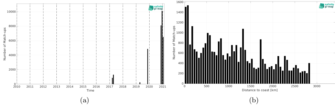
Figure 2: Number of match-ups between TSG (GOSUD-Sailing-ship) and SMAP SSS L3 v5.0 - 8-Day running (JPL) SSS as a function of time (a) and as function of the distance to coast (b) over the South Atlantic Ocean Pi-MEP region and for the full satellite product period.
