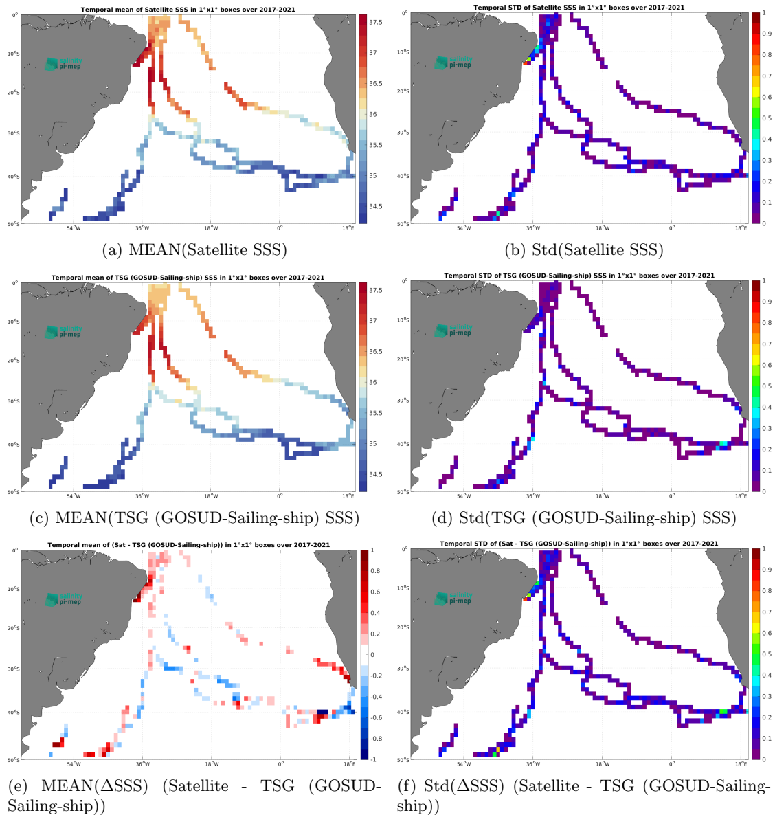
Figure 7: Temporal mean (left) and Std (right) of SSS from SMAP SSS L3 v5.0 - 8-Day running (JPL) (top), TSG (GOSUD-Sailing-ship) (middle), and of \Delta SSS (Satellite - TSG (GOSUD-Sailing-ship)). Only match-up pairs are used to generate these maps.
