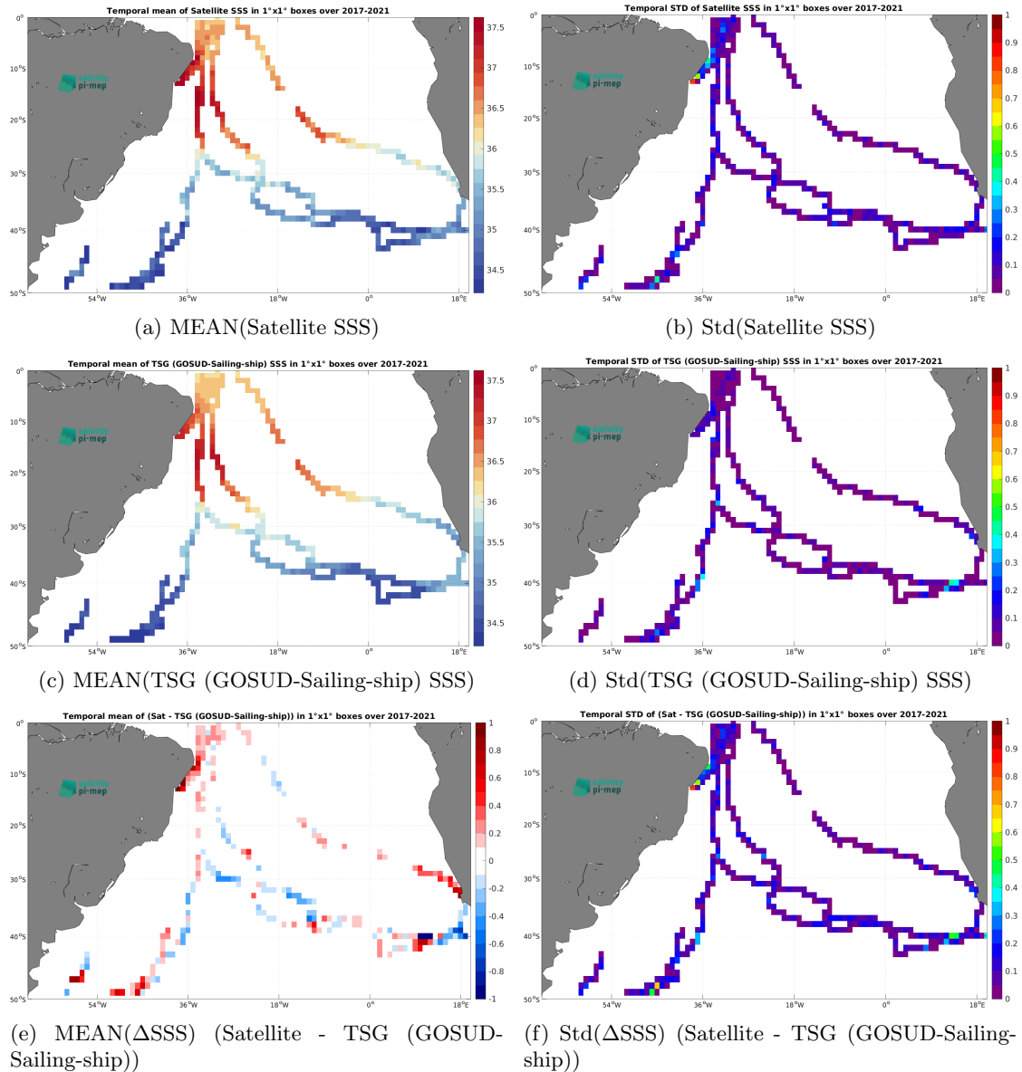
Figure 6: Temporal mean (left) and Std (right) of SSS from SMAP SSS L3 v5.0 - 8-Day running (JPL) (top), TSG (GOSUD-Sailing-ship) (middle), and of \Delta SSS (Satellite - TSG (GOSUD-Sailing-ship)). Only match-up pairs are used to generate these maps.
