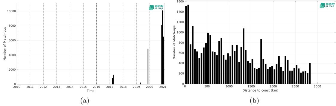
Figure 1: Number of match-ups between TSG (GOSUD-Sailing-ship) and SMAP SSS L3 v5.0 - 8-Day running (JPL) SSS as a function of time (a) and as function of the distance to coast (b) over the South Atlantic Ocean Pi-MEP region and for the full satellite product period.
