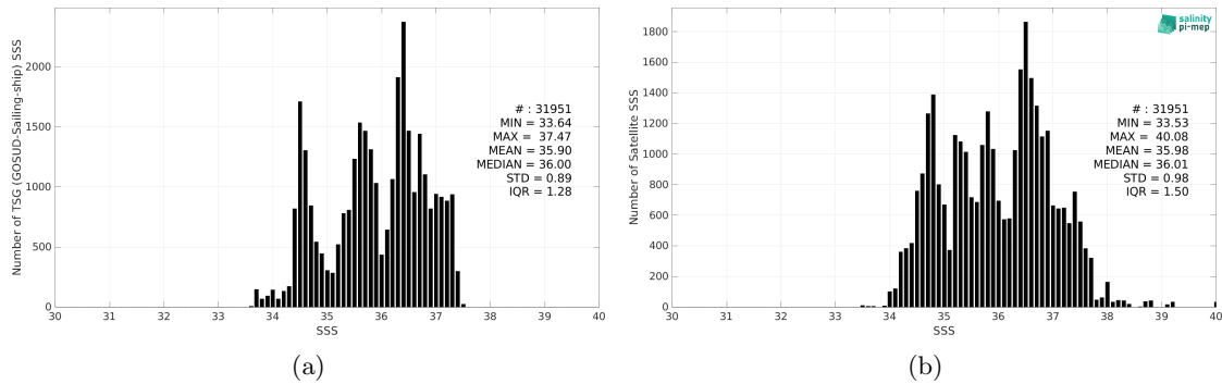
Figure 2: Histograms of SSS from TSG (GOSUD-Sailing-ship) (a) and SMAP SSS L3 v5.0 - 8-Day running (JPL) (b) considering all match-up pairs per bins of 0.1 over the South Atlantic Ocean Pi-MEP region and for the full satellite product period.
