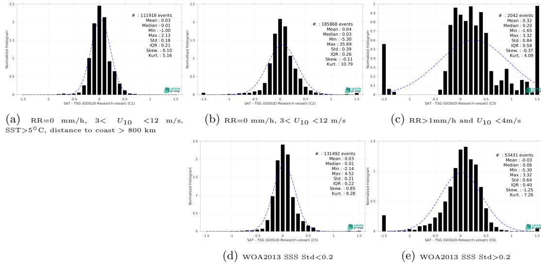
Figure 15: Normalized histogram of \Delta SSS (SMAP SSS L3 v5.0 - 8-Day running (JPL) - TSG (GOSUD-Research-vessel)) for 5 different subdatasets corresponding to: RR=0 mm/h, 3 < U_{10} < 12 m/s, SST>5°C, distance to coast > 800 km (a), RR=0 mm/h, 3 < U_{10} < 12 m/s (b), RR>1mm/h and U_{10} < 4 m/s (c), WOA2013 SSS Std<0.2 (d), WOA2013 SSS Std>0.2 (e).
