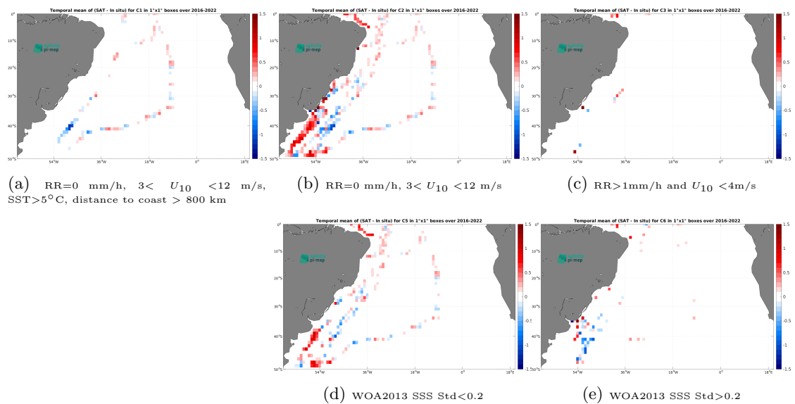
Figure 14: Temporal mean gridded over spatial boxes of size 1^\circ \times 1^\circ of \Delta SSS (SMAP SSS L3 v5.0 - 8-Day running (JPL) - TSG (CSIC-UTM)) for 5 different subdatasets corresponding to:RR=0 mm/h, 3 < U_{10} < 12 m/s, SST > 5°C, distance to coast > 800 km (a), RR=0 mm/h, 3 < U_{10} < 12 m/s (b), RR > 1mm/h and U_{10} < 4 m/s (c), WOA2013 SSS Std < 0.2 (d), WOA2013 SSS Std > 0.2 (e).
