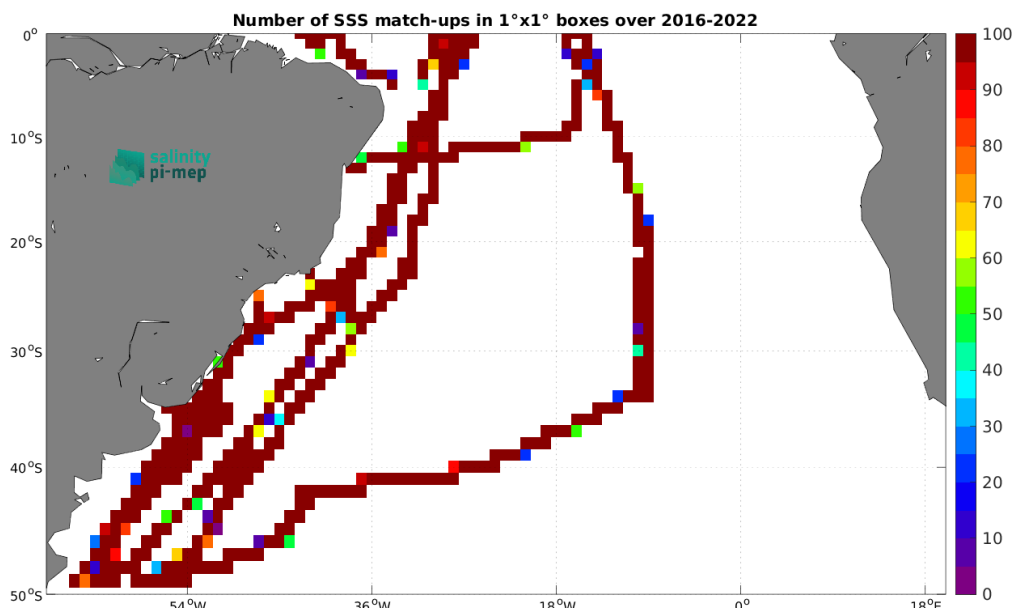
Figure 5: Number of SSS match-ups between TSG (CSIC-UTM) SSS and the SMAP SSS L3 v5.0 - 8-Day running (JPL) SSS product for the South Atlantic Ocean Pi-MEP region over 1^\circ \times 1^\circ boxes and for the full satellite product period.
