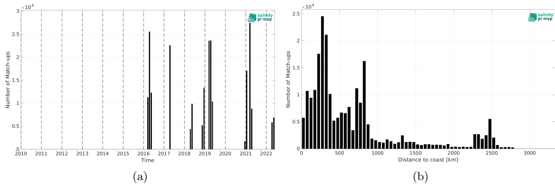
Figure 2: Number of match-ups between TSG (CSIC-UTM) and SMAP SSS L3 v5.0 - 8-Day running (JPL) SSS as a function of time (a) and as function of the distance to coast (b) over the South Atlantic Ocean Pi-MEP region and for the full satellite product period.
