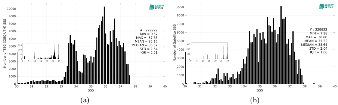
Figure 3: Histograms of SSS from TSG (CSIC-UTM) (a) and SMAP SSS L3 v5.0 - 8-Day running (JPL) (b) considering all match-up pairs per bins of 0.1 over the South Atlantic Ocean Pi-MEP region and for the full satellite product period.
