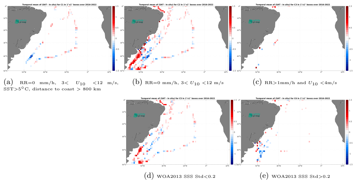
Figure 14: Temporal mean gridded over spatial boxes of size 1^\circ \times 1^\circ of \Delta\text{SSS} (SMAP SSS L3 v5.0 - 8-Day running (JPL) - TSG (CSIC-UTM)) for 5 different subdatasets corresponding to:RR=0 mm/h, 3 < U_{10} < 12 m/s, SST >5^\circ\text{C} , distance to coast > 800 km (a), RR=0 mm/h, 3 < U_{10} < 12 m/s (b), RR >1 mm/h and U_{10} < 4 m/s (c), WOA2013 SSS Std <0.2 (d), WOA2013 SSS Std >0.2 (e).
