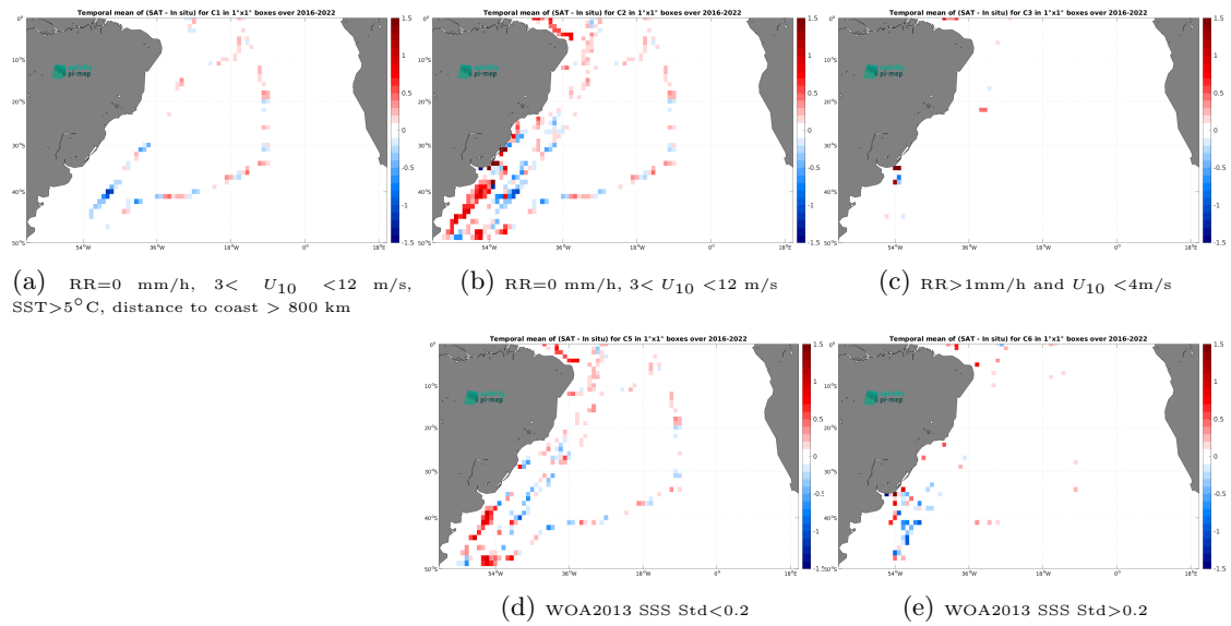
Figure 12: Temporal mean gridded over spatial boxes of size 1^\circ \times 1^\circ of \Delta\text{SSS} (SMAP SSS L3 v5.0 - 8-Day running (JPL) - TSG (CSIC-UTM)) for 5 different subdatasets corresponding to:RR=0 mm/h, 3 < U_{10} < 12 m/s, SST >5^\circ\text{C} , distance to coast > 800 km (a), RR=0 mm/h, 3 < U_{10} < 12 m/s (b), RR >1 mm/h and U_{10} < 4 m/s (c), WOA2013 SSS Std <0.2 (d), WOA2013 SSS Std >0.2 (e).
