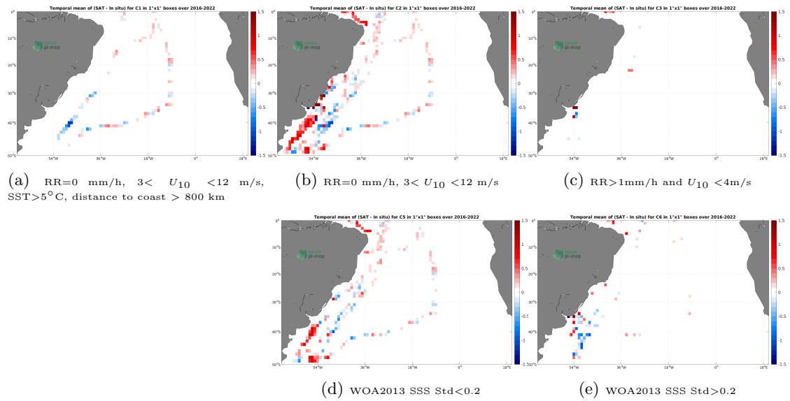
Figure 12: Temporal mean gridded over spatial boxes of size 1^\circ \times 1^\circ of \Delta SSS (SMAP SSS L3 v5.0 - 8-Day running (JPL) - TSG (CSIC-UTM)) for 5 different subdatasets corresponding to:RR=0 mm/h, 3 < U_{10} < 12 m/s, SST >5^\circ\text{C} , distance to coast > 800 km (a), RR=0 mm/h, 3 < U_{10} < 12 m/s (b), RR >1 mm/h and U_{10} < 4 m/s (c), WOA2013 SSS Std <0.2 (d), WOA2013 SSS Std >0.2 (e).
