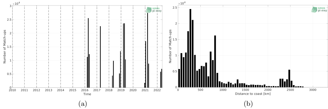
Figure 1: Number of match-ups between TSG (CSIC-UTM) and SMAP SSS L3 v5.0 - 8-Day running (JPL) SSS as a function of time (a) and as function of the distance to coast (b) over the South Atlantic Ocean Pi-MEP region and for the full satellite product period.
