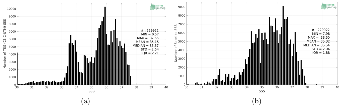
Figure 2: Histograms of SSS from TSG (CSIC-UTM) (a) and SMAP SSS L3 v5.0 - 8-Day running (JPL) (b) considering all match-up pairs per bins of 0.1 over the South Atlantic Ocean Pi-MEP region and for the full satellite product period.
