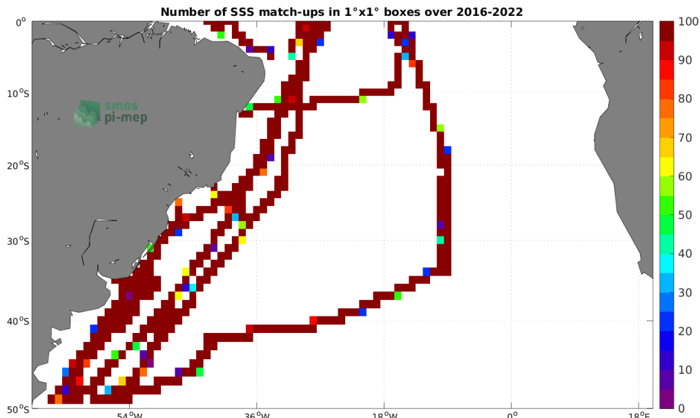
Figure 4: Number of SSS match-ups between TSG (CSIC-UTM) SSS and the SMAP SSS L3 v5.0 - 8-Day running (JPL) SSS product for the South Atlantic Ocean Pi-MEP region over 1^\circ \times 1^\circ boxes and for the full satellite product period.
