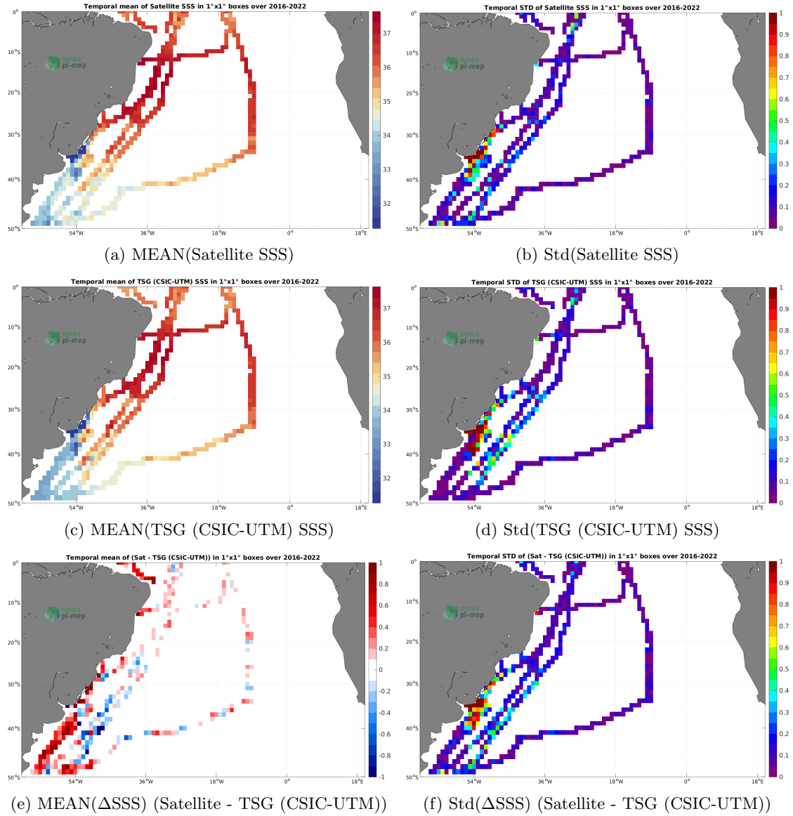
Figure 6: Temporal mean (left) and Std (right) of SSS from SMAP SSS L3 v5.0 - 8-Day running (JPL) (top), TSG (CSIC-UTM) (middle), and of \Delta SSS (Satellite - TSG (CSIC-UTM)). Only match-up pairs are used to generate these maps.
