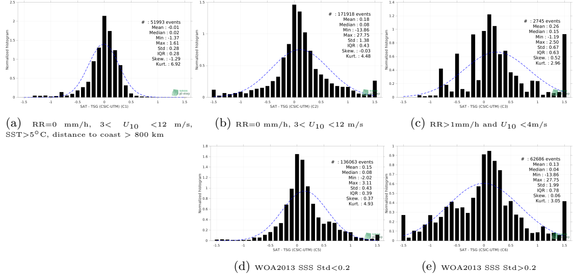
Figure 13: Normalized histogram of \Delta SSS (SMAP SSS L3 v5.0 - 8-Day running (JPL) - TSG (CSIC-UTM)) for 5 different subdatasets corresponding to: RR=0 mm/h, 3 < U_{10} < 12 m/s, SST > 5°C, distance to coast > 800 km (a), RR=0 mm/h, 3 < U_{10} < 12 m/s (b), RR > 1mm/h and U_{10} < 4 m/s (c), WOA2013 SSS Std < 0.2 (d), WOA2013 SSS Std > 0.2 (e).
