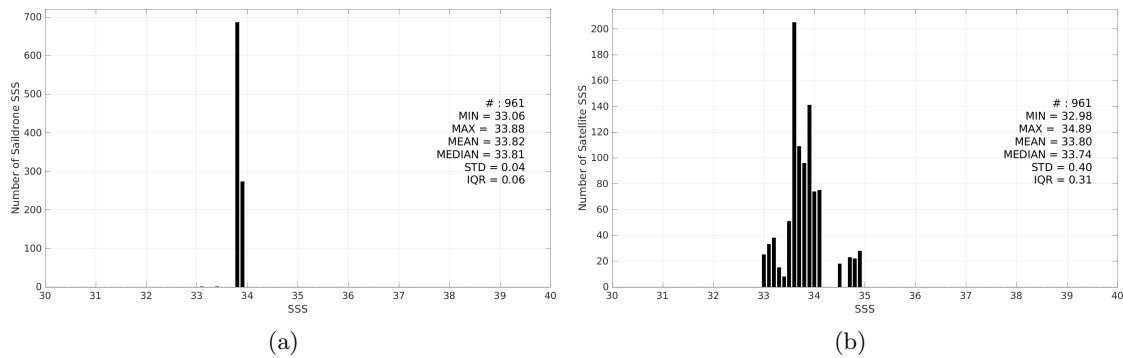
Figure 3: Histograms of SSS from Saildrone (a) and SMAP SSS L3 v5.0 - 8-Day running (JPL) (b) considering all match-up pairs per bins of 0.1 over the South Atlantic Ocean Pi-MEP region and for the full satellite product period.
