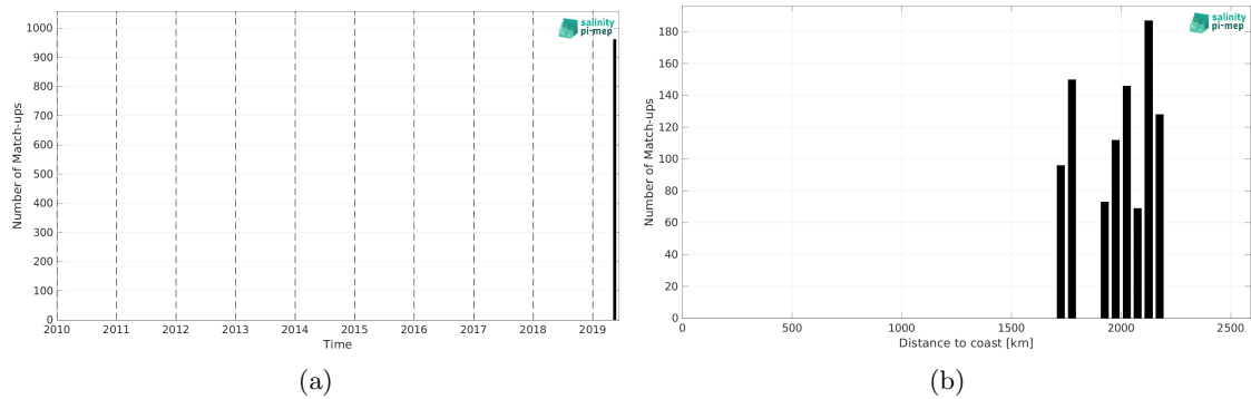
Figure 2: Number of match-ups between Saildrone and SMAP SSS L3 v5.0 - 8-Day running (JPL) SSS as a function of time (a) and as function of the distance to coast (b) over the South Atlantic Ocean Pi-MEP region and for the full satellite product period.
