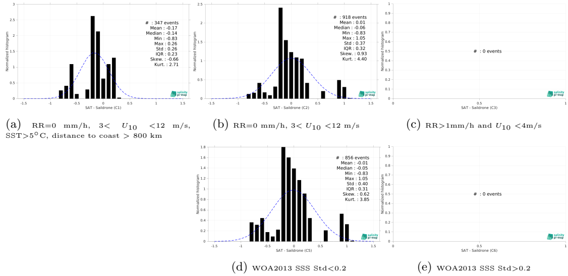
Figure 15: Normalized histogram of \Delta SSS (SMAP SSS L3 v5.0 - 8-Day running (JPL) - Salldrone) for 5 different subdatasets corresponding to: RR=0 mm/h, 3 < U_{10} < 12 m/s, SST > 5°C, distance to coast > 800 km (a), RR=0 mm/h, 3 < U_{10} < 12 m/s (b), RR > 1mm/h and U_{10} < 4 m/s (c), WOA2013 SSS Std < 0.2 (d), WOA2013 SSS Std > 0.2 (e).
