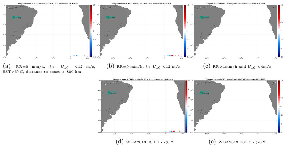
Figure 14: Temporal mean gridded over spatial boxes of size 1^\circ \times 1^\circ of \Delta SSS (SMAP SSS L3 v5.0 - 8-Day running (JPL) - Saildrone) for 5 different subdatasets corresponding to:RR=0 mm/h, 3 < U_{10} < 12 m/s, SST >5^\circ\text{C} , distance to coast > 800 km (a), RR=0 mm/h, 3 < U_{10} < 12 m/s (b), RR >1 mm/h and U_{10} < 4 m/s (c), WOA2013 SSS Std <0.2 (d), WOA2013 SSS Std >0.2 (e).
