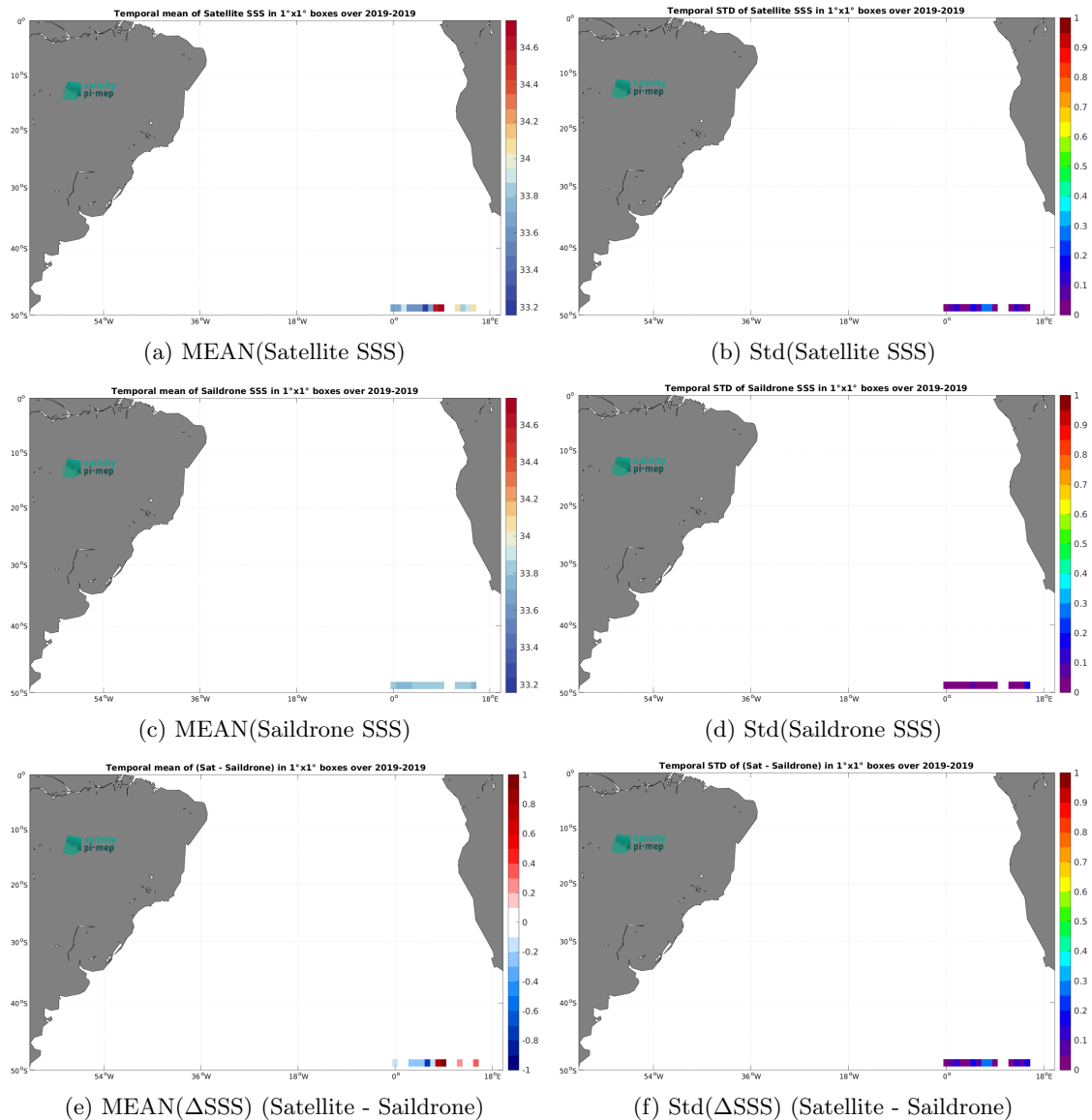
Figure 7: Temporal mean (left) and Std (right) of SSS from SMAP SSS L3 v5.0 - 8-Day running (JPL) (top), Saildrone (middle), and of \Delta SSS (Satellite - Saildrone). Only match-up pairs are used to generate these maps.
