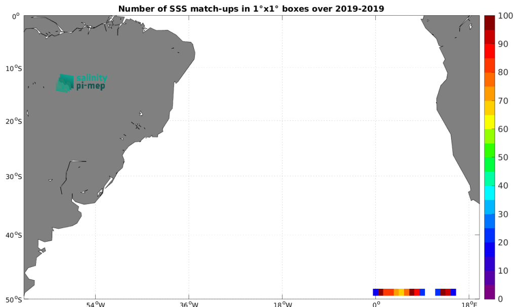
Figure 5: Number of SSS match-ups between Saildrone SSS and the SMAP SSS L3 v5.0 - 8-Day running (JPL) SSS product for the South Atlantic Ocean Pi-MEP region over 1^\circ \times 1^\circ boxes and for the full satellite product period.
