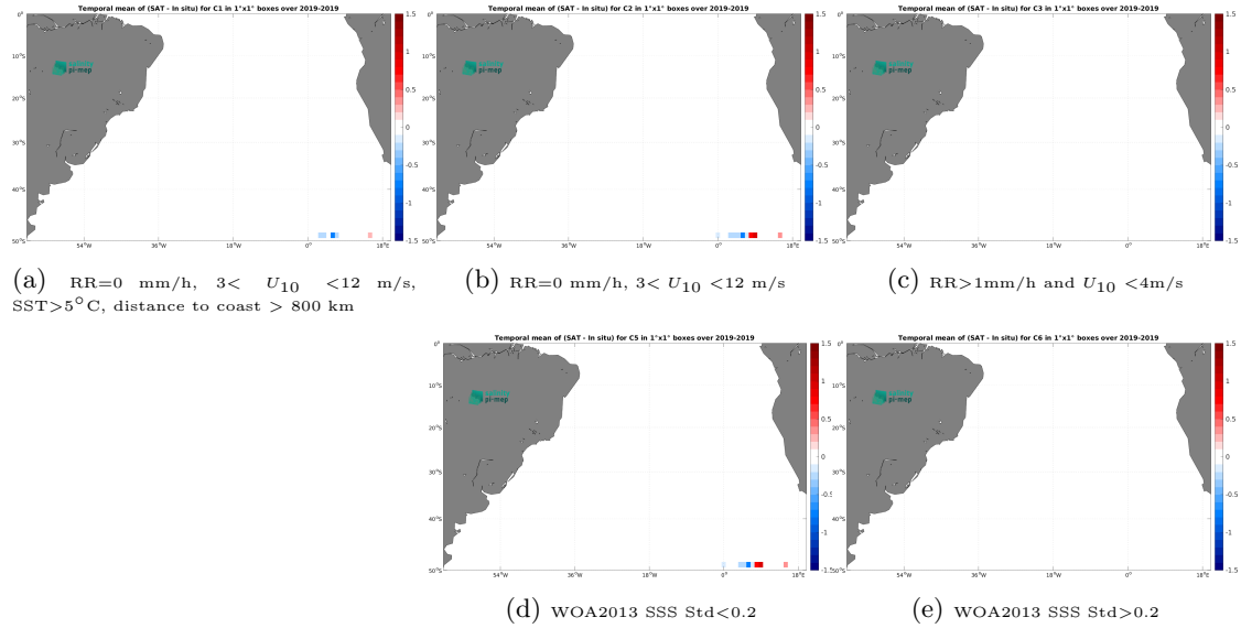
Figure 12: Temporal mean gridded over spatial boxes of size 1^{\circ}\times 1^{\circ} of \Delta\text{SSS} (SMAP SSS L3 v5.0 - 8-Day running (JPL) - Sairdron) for 5 different subdatasets corresponding to:RR=0 mm/h, 3 < U_{10} < 12 m/s, SST >5^{\circ}\text{C} , distance to coast > 800 km (a), RR=0 mm/h, 3 < U_{10} < 12 m/s (b), RR >1 mm/h and U_{10} < 4 m/s (c), WOA2013 SSS Std <0.2 (d), WOA2013 SSS Std >0.2 (e).
