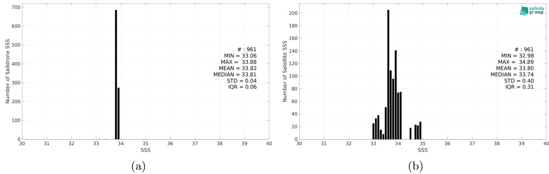
Figure 2: Histograms of SSS from Saildrone (a) and SMAP SSS L3 v5.0 - 8-Day running (JPL) (b) considering all match-up pairs per bins of 0.1 over the South Atlantic Ocean Pi-MEP region and for the full satellite product period.
