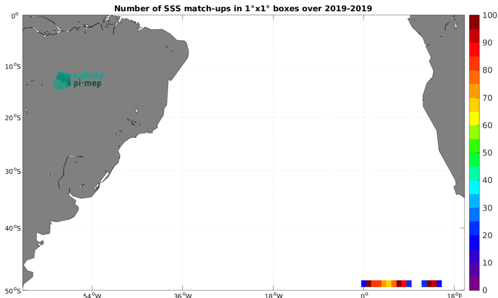
Figure 4: Number of SSS match-ups between Saildrone SSS and the SMAP SSS L3 v5.0 - 8-Day running (JPL) SSS product for the South Atlantic Ocean Pi-MEP region over 1^\circ \times 1^\circ boxes and for the full satellite product period.
