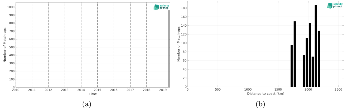
Figure 1: Number of match-ups between Saildrone and SMAP SSS L3 v5.0 - 8-Day running (JPL) SSS as a function of time (a) and as function of the distance to coast (b) over the South Atlantic Ocean Pi-MEP region and for the full satellite product period.
