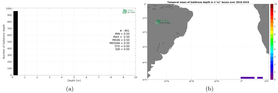
Figure 3: Histograms of the depth of the upper level SSS measurements from Sailldrone in the Match-up DataBase for the South Atlantic Ocean Pi-MEP region (a) and temporal mean spatial distribution of pressure of the in situ SSS data over 1^\circ \times 1^\circ boxes and for the full satellite product period (b).
