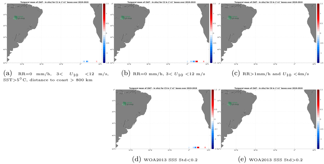
Figure 12: Temporal mean gridded over spatial boxes of size 1^{\circ}\times 1^{\circ} of \Delta\text{SSS} (SMAP SSS L3 v5.0 - 8-Day running (JPL) - Sairdrone) for 5 different subdatasets corresponding to:RR=0 mm/h, 3 < U_{10} < 12 m/s, SST >5^{\circ}\text{C} , distance to coast > 800 km (a), RR=0 mm/h, 3 < U_{10} < 12 m/s (b), RR >1 mm/h and U_{10} < 4 m/s (c), WOA2013 SSS Std <0.2 (d), WOA2013 SSS Std >0.2 (e).
