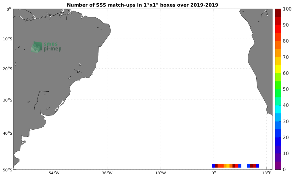
Figure 4: Number of SSS match-ups between Sailldrone SSS and the SMAP SSS L3 v5.0 - 8-Day running (JPL) SSS product for the South Atlantic Ocean Pi-MEP region over 1^\circ \times 1^\circ boxes and for the full satellite product period.
