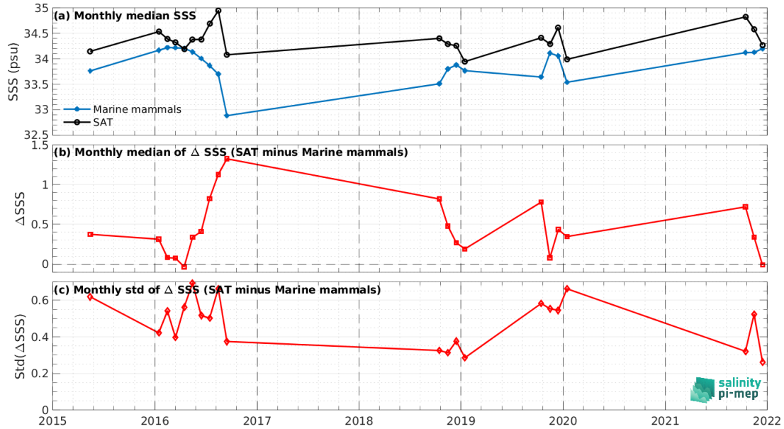
Figure 8: Time series of the monthly median SSS (top), median of \Delta\text{SSS} (Satellite - Marine mammals) and Std of \Delta\text{SSS} (Satellite - Marine mammals) over the South Atlantic Ocean Pi-MEP region considering all match-ups collected by the Pi-MEP.
