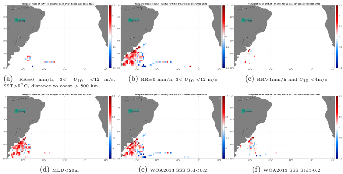
Figure 14: Temporal mean gridded over spatial boxes of size 1^\circ \times 1^\circ of \Delta\text{SSS} (SMAP SSS L3 v5.0 - 8-Day running (JPL) - Marine mammals) for 6 different subdatasets corresponding to: RR=0 mm/h, 3 < U_{10} < 12 m/s, SST > 5°C, distance to coast > 800 km (a), RR=0 mm/h, 3 < U_{10} < 12 m/s (b), RR > 1mm/h and U_{10} < 4 m/s (c),MLD < 20m (d),WOA2013 SSS Std < 0.2 (e),WOA2013 SSS Std > 0.2 (f).
