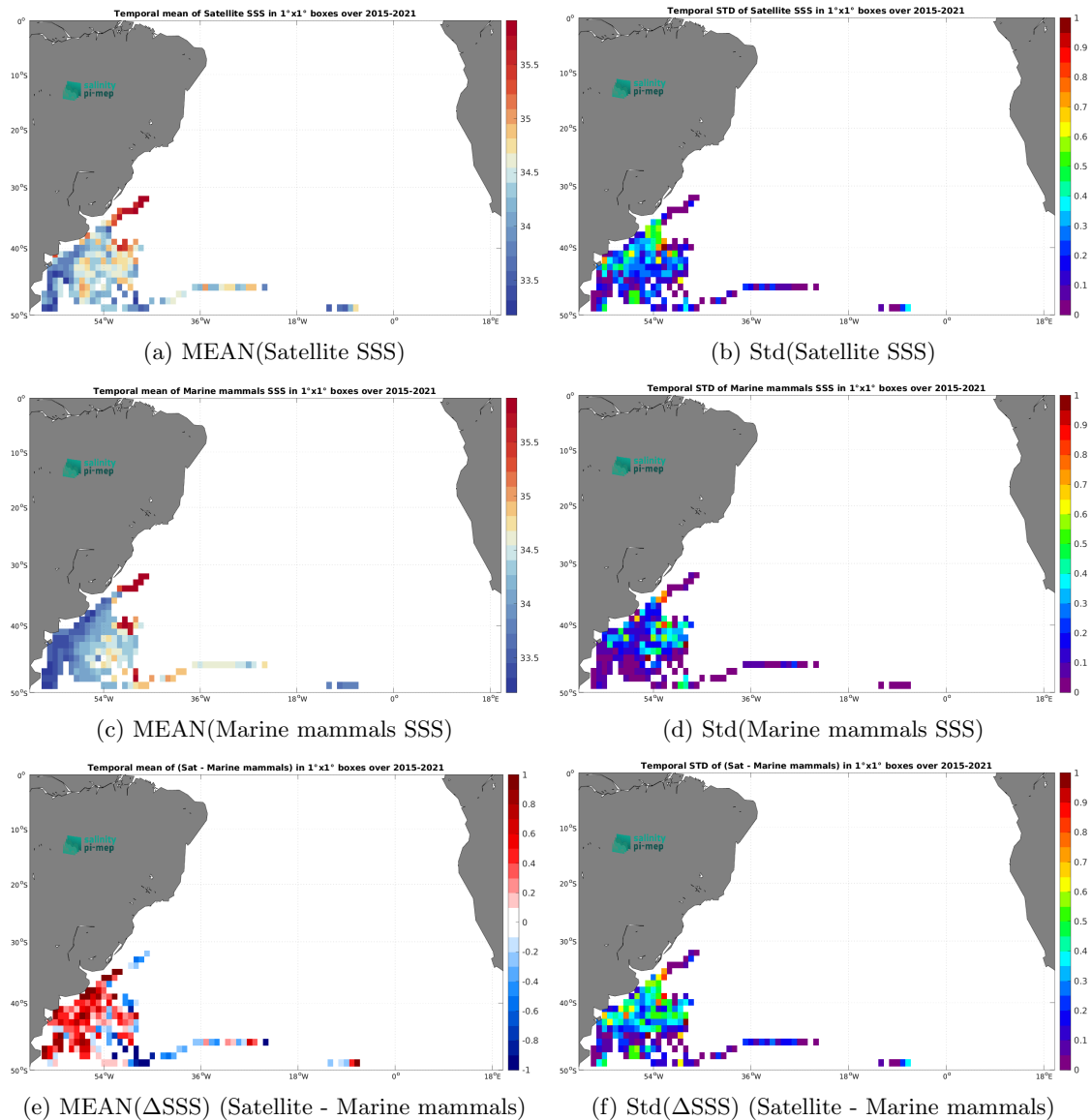
Figure 7: Temporal mean (left) and Std (right) of SSS from SMAP SSS L3 v5.0 - 8-Day running (JPL) (top), Marine mammals (middle), and of \Delta SSS (Satellite - Marine mammals). Only match-up pairs are used to generate these maps.
