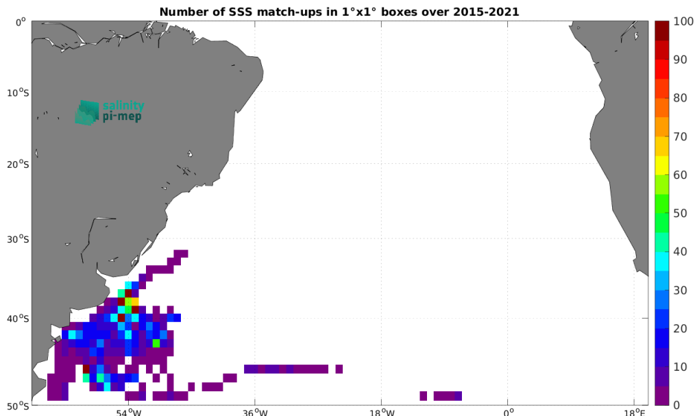
Figure 5: Number of SSS match-ups between Marine mammals SSS and the SMAP SSS L3 v5.0 - 8-Day running (JPL) SSS product for the South Atlantic Ocean Pi-MEP region over 1^\circ \times 1^\circ boxes and for the full satellite product period.
