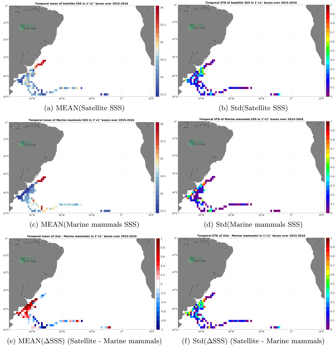
Figure 6: Temporal mean (left) and Std (right) of SSS from SMAP SSS L3 v5.0 - 8-Day running (JPL) (top), Marine mammals (middle), and of \Delta SSS (Satellite - Marine mammals). Only match-up pairs are used to generate these maps.
