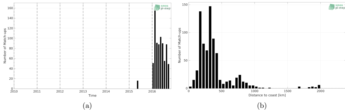
Figure 1: Number of match-ups between Marine mammals and SMAP SSS L3 v5.0 - 8-Day running (JPL) SSS as a function of time (a) and as function of the distance to coast (b) over the South Atlantic Ocean Pi-MEP region and for the full satellite product period.
