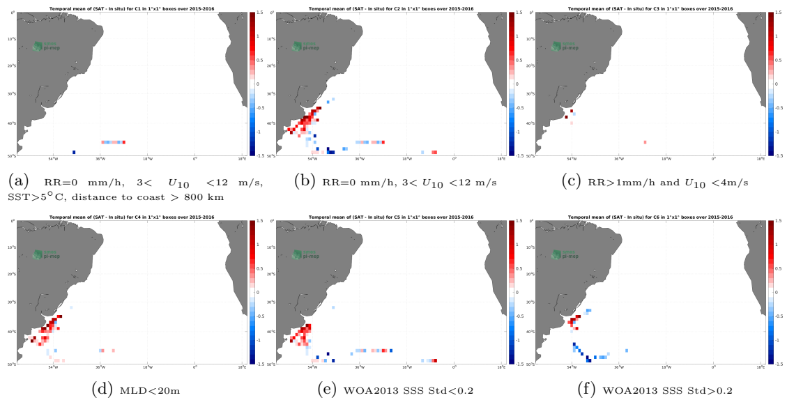
Figure 12: Temporal mean gridded over spatial boxes of size 1^\circ \times 1^\circ of \Delta SSS (SMAP SSS L3 v5.0 - 8-Day running (JPL) - Marine mammals) for 6 different subdatasets corresponding to:RR=0 mm/h, 3 < U_{10} < 12 m/s, SST > 5^\circ\text{C} , distance to coast > 800 km (a), RR=0 mm/h, 3 < U_{10} < 12 m/s (b), RR > 1 mm/h and U_{10} < 4 m/s (c),MLD < 20 m (d),WOA2013 SSS Std < 0.2 (e),WOA2013 SSS Std > 0.2 (f).
