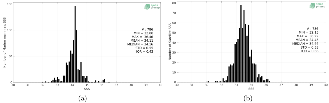
Figure 2: Histograms of SSS from Marine mammals (a) and SMAP SSS L3 v5.0 - 8-Day running (JPL) (b) considering all match-up pairs per bins of 0.1 over the South Atlantic Ocean Pi-MEP region and for the full satellite product period.
