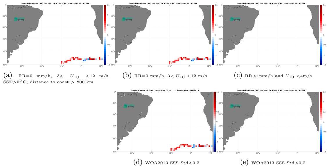
Figure 13: Temporal mean gridded over spatial boxes of size 1^\circ \times 1^\circ of \Delta\text{SSS} (SMAP SSS L3 v5.0 - 8-Day running (JPL) - Surface drifters) for 5 different subdatasets corresponding to:RR=0 mm/h, 3 < U_{10} < 12 m/s, SST >5^\circ\text{C} , distance to coast > 800 km (a), RR=0 mm/h, 3 < U_{10} < 12 m/s (b), RR >1 mm/h and U_{10} < 4 m/s (c), WOA2013 SSS Std <0.2 (d), WOA2013 SSS Std >0.2 (e).
