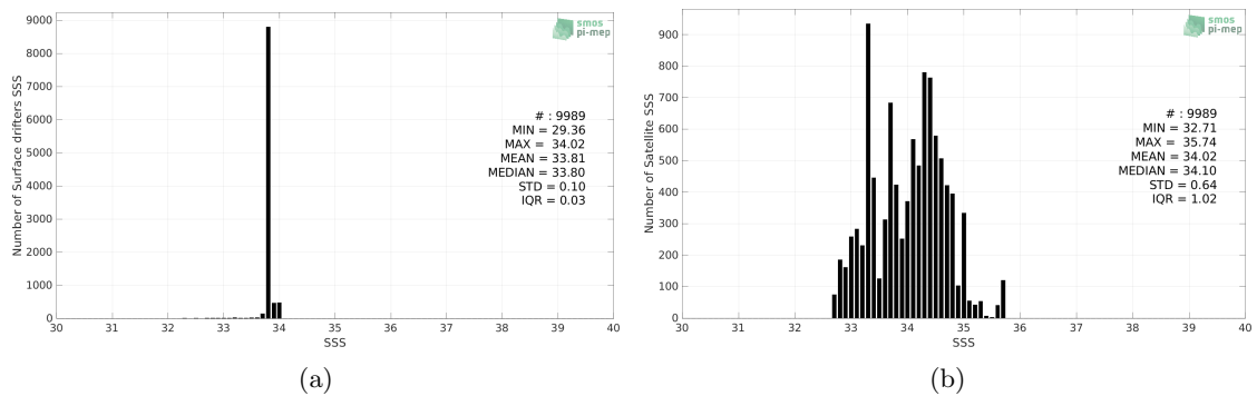
Figure 2: Histograms of SSS from Surface drifters (a) and SMAP SSS L3 v5.0 - 8-Day running (JPL) (b) considering all match-up pairs per bins of 0.1 over the South Atlantic Ocean Pi-MEP region and for the full satellite product period.
