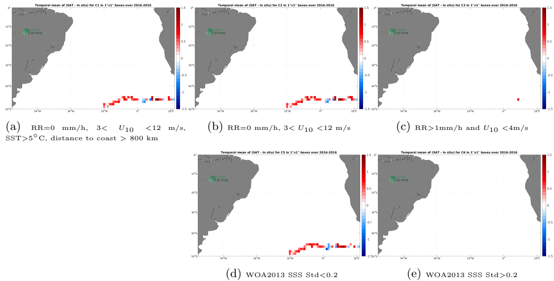
Figure 11: Temporal mean gridded over spatial boxes of size 1^{\circ}\times 1^{\circ} of \Delta\text{SSS} (SMAP SSS L3 v5.0 - 8-Day running (JPL) - Surface drifters) for 5 different subdatasets corresponding to:RR=0 mm/h, 3 < U_{10} < 12 m/s, SST >5^{\circ}\text{C} , distance to coast > 800 km (a), RR=0 mm/h, 3 < U_{10} < 12 m/s (b), RR >1 mm/h and U_{10} < 4 m/s (c), WOA2013 SSS Std <0.2 (d), WOA2013 SSS Std >0.2 (e).
