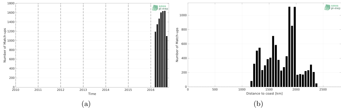
Figure 1: Number of match-ups between Surface drifters and SMAP SSS L3 v5.0 - 8-Day running (JPL) SSS as a function of time (a) and as function of the distance to coast (b) over the South Atlantic Ocean Pi-MEP region and for the full satellite product period.
