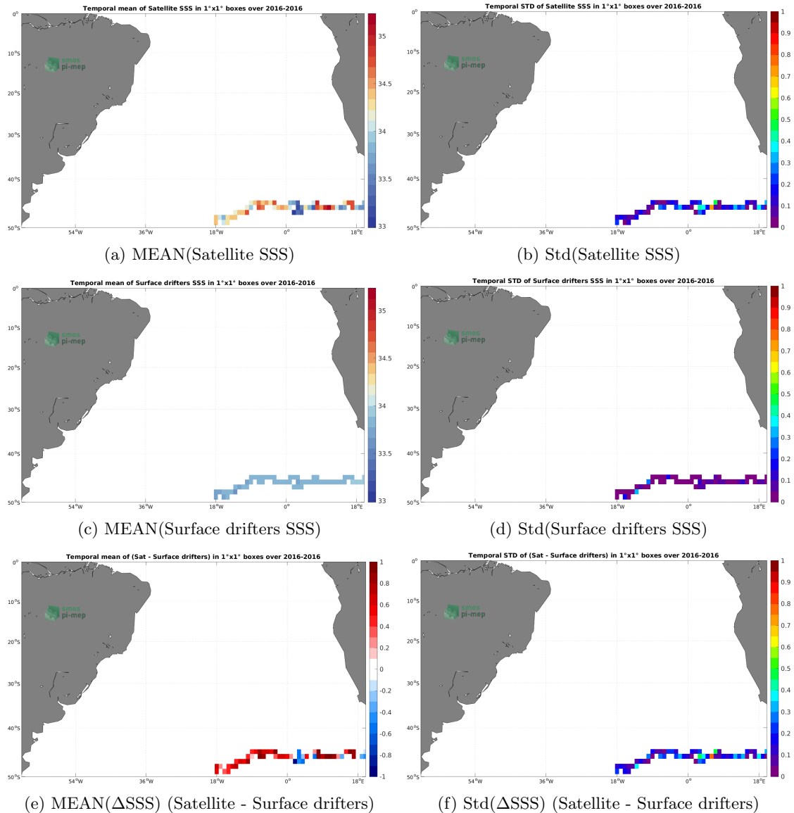
Figure 5: Temporal mean (left) and Std (right) of SSS from SMAP SSS L3 v5.0 - 8-Day running (JPL) (top), Surface drifters (middle), and of \Delta SSS (Satellite - Surface drifters). Only match-up pairs are used to generate these maps.
