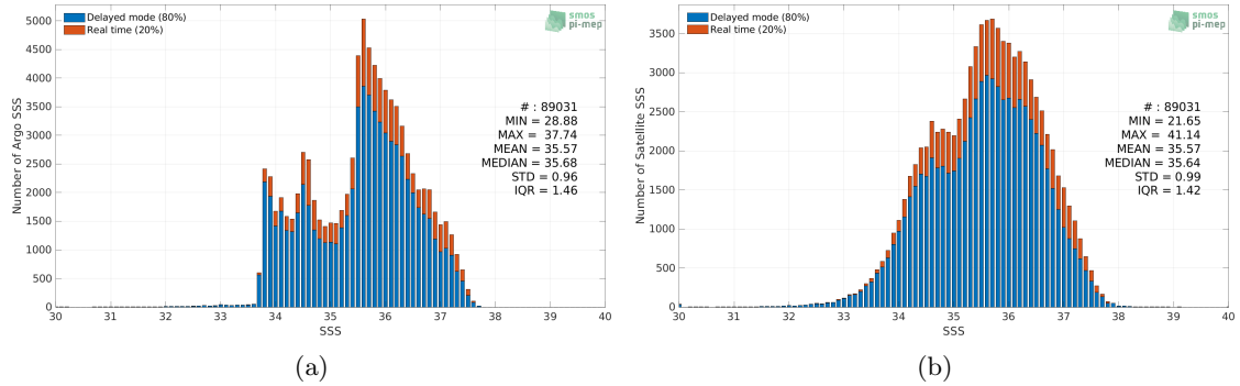
Figure 2: Histograms of SSS from Argo (a) and SMAP SSS L3 v5.0 - 8-Day running (JPL) (b) considering all match-up pairs per bins of 0.1 over the South Atlantic Ocean Pi-MEP region and for the full satellite product period.
