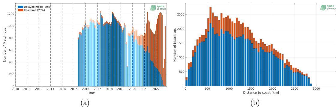
Figure 1: Number of match-ups between Argo and SMAP SSS L3 v5.0 - 8-Day running (JPL) SSS as a function of time (a) and as function of the distance to coast (b) over the South Atlantic Ocean Pi-MEP region and for the full satellite product period.
