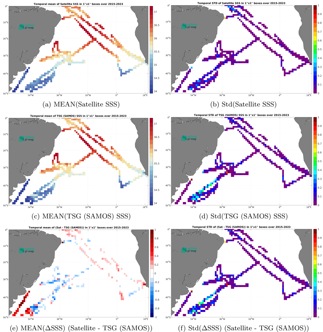
Figure 7: Temporal mean (left) and Std (right) of SSS from SMAP SSS L3 v5.0 - Monthly (JPL) (top), TSG (SAMOS) (middle), and of \Delta SSS (Satellite - TSG (SAMOS)). Only match-up pairs are used to generate these maps.
