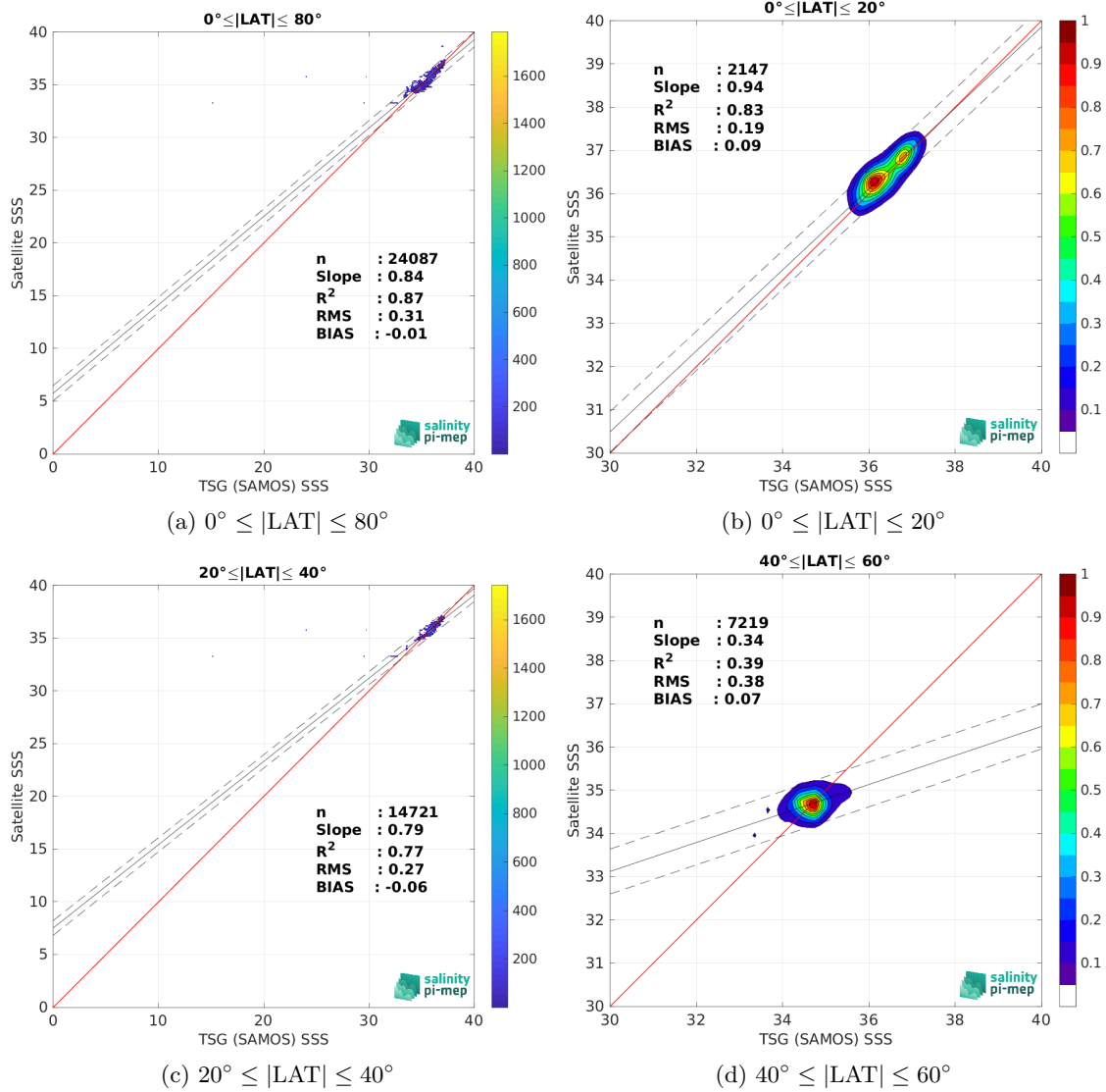
Figure 10: Contour maps of the concentration of SMAP SSS L3 v5.0 - Monthly (JPL) SSS (y-axis) versus TSG (SAMOS) SSS (x-axis) at match-up pairs for different latitude bands. For each plot, the red line shows x=y . The black thin and dashed lines indicate a linear fit through the data cloud and the \pm 95\% confidence levels, respectively. The number match-up pairs n , the slope and R^2 coefficient of the linear fit, the root mean square (RMS) and the mean bias between satellite and in situ data are indicated for each latitude band in each plots.
