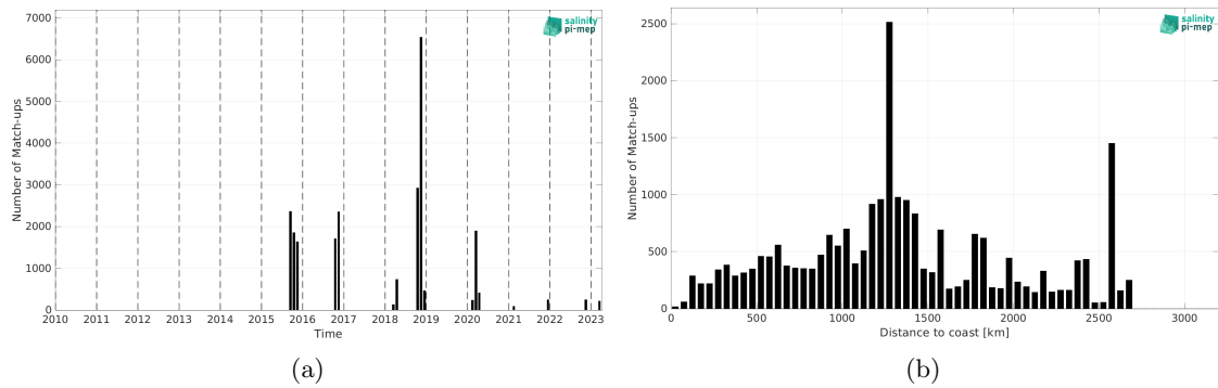
Figure 2: Number of match-ups between TSG (SAMOS) and SMAP SSS L3 v5.0 - Monthly (JPL) SSS as a function of time (a) and as function of the distance to coast (b) over the South Atlantic Ocean Pi-MEP region and for the full satellite product period.
