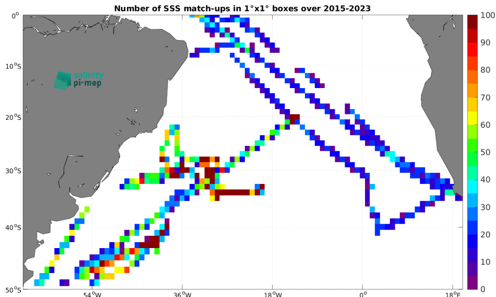
Figure 5: Number of SSS match-ups between TSG (SAMOS) SSS and the SMAP SSS L3 v5.0 - Monthly (JPL) SSS product for the South Atlantic Ocean Pi-MEP region over 1^\circ \times 1^\circ boxes and for the full satellite product period.
