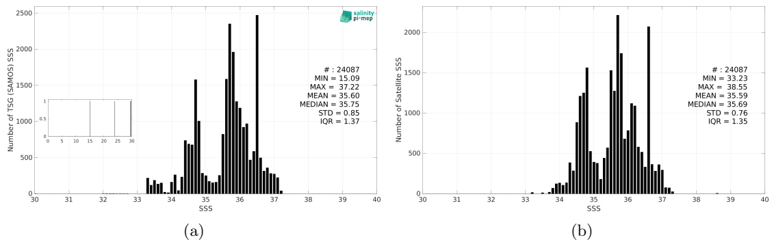
Figure 3: Histograms of SSS from TSG (SAMOS) (a) and SMAP SSS L3 v5.0 - Monthly (JPL) (b) considering all match-up pairs per bins of 0.1 over the South Atlantic Ocean Pi-MEP region and for the full satellite product period.
