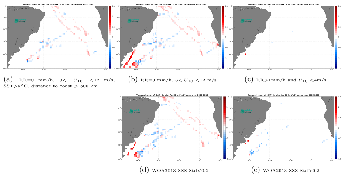
Figure 14: Temporal mean gridded over spatial boxes of size 1^\circ \times 1^\circ of \Delta SSS (SMAP SSS L3 v5.0 - Monthly (JPL) - TSG (SAMOS)) for 5 different subdatasets corresponding to:RR=0 mm/h, 3 < U_{10} < 12 m/s, SST>5°C, distance to coast > 800 km (a), RR=0 mm/h, 3 < U_{10} < 12 m/s (b), RR>1mm/h and U_{10} < 4 m/s (c), WOA2013 SSS Std<0.2 (d), WOA2013 SSS Std>0.2 (e).
