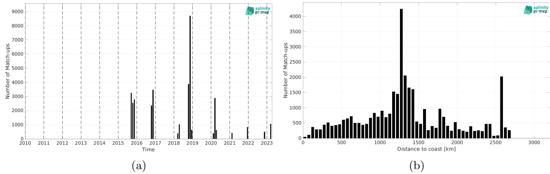
Figure 1: Number of match-ups between TSG (SAMOS) and SMAP SSS L3 v5.0 - Monthly (JPL) SSS as a function of time (a) and as function of the distance to coast (b) over the South Atlantic Ocean Pi-MEP region and for the full satellite product period.
