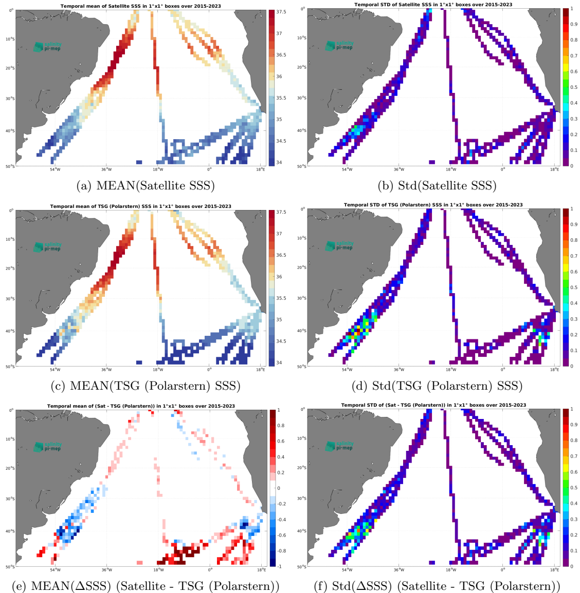
Figure 7: Temporal mean (left) and Std (right) of SSS from SMAP SSS L3 v5.0 - Monthly (JPL) (top), TSG (Polarstern) (middle), and of \Delta SSS (Satellite - TSG (Polarstern)). Only match-up pairs are used to generate these maps.
