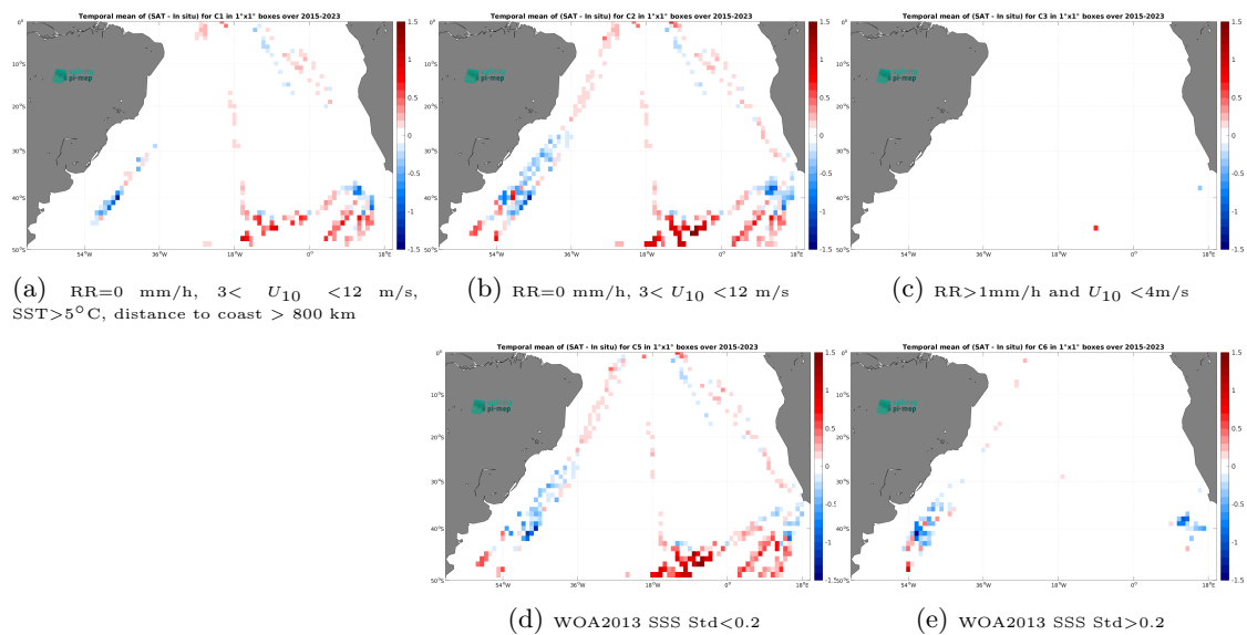
Figure 14: Temporal mean gridded over spatial boxes of size 1^\circ \times 1^\circ of \Delta\text{SSS} (SMAP SSS L3 v5.0 - Monthly (JPL) - TSG (Polarstern)) for 5 different subdatasets corresponding to:RR=0 mm/h, 3 < U_{10} < 12 m/s, SST >5^\circ\text{C} , distance to coast > 800 km (a), RR=0 mm/h, 3 < U_{10} < 12 m/s (b), RR >1 mm/h and U_{10} < 4 m/s (c), WOA2013 SSS Std <0.2 (d), WOA2013 SSS Std >0.2 (e).
