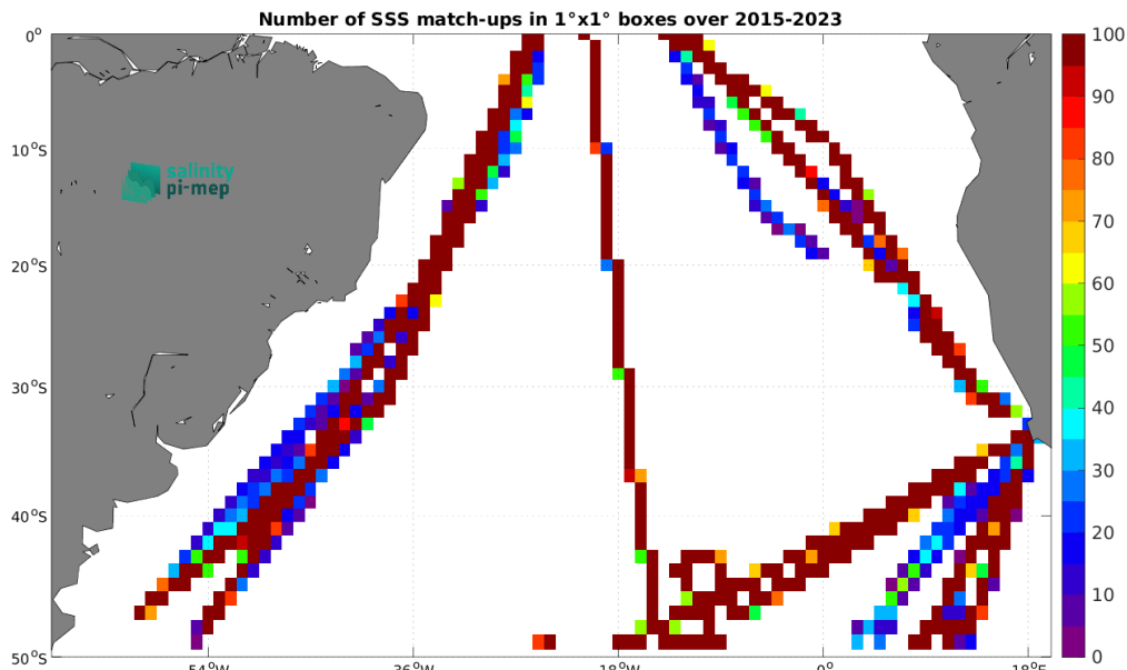
Figure 5: Number of SSS match-ups between TSG (Polarstern) SSS and the SMAP SSS L3 v5.0 - Monthly (JPL) SSS product for the South Atlantic Ocean Pi-MEP region over 1^\circ \times 1^\circ boxes and for the full satellite product period.
