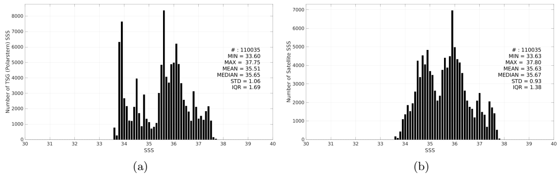
Figure 3: Histograms of SSS from TSG (Polarstern) (a) and SMAP SSS L3 v5.0 - Monthly (JPL) (b) considering all match-up pairs per bins of 0.1 over the South Atlantic Ocean Pi-MEP region and for the full satellite product period.
