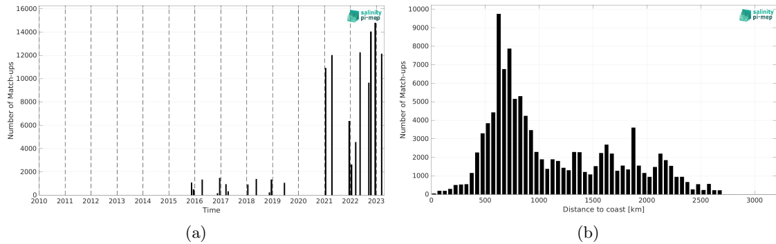
Figure 2: Number of match-ups between TSG (Polarstern) and SMAP SSS L3 v5.0 - Monthly (JPL) SSS as a function of time (a) and as function of the distance to coast (b) over the South Atlantic Ocean Pi-MEP region and for the full satellite product period.
