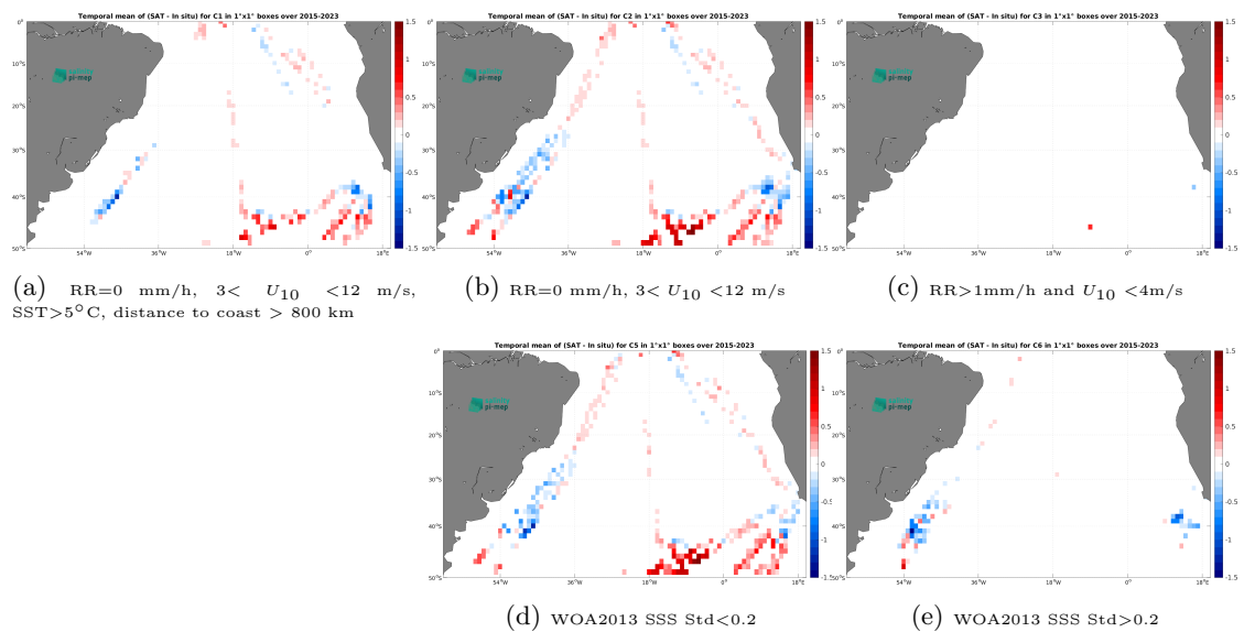
Figure 14: Temporal mean gridded over spatial boxes of size 1^\circ \times 1^\circ of \Delta SSS (SMAP SSS L3 v5.0 - Monthly (JPL) - TSG (Polarstern)) for 5 different subdatasets corresponding to:RR=0 mm/h, 3 < U_{10} < 12 m/s, SST>5°C, distance to coast > 800 km (a), RR=0 mm/h, 3 < U_{10} < 12 m/s (b), RR>1mm/h and U_{10} < 4 m/s (c), WOA2013 SSS Std<0.2 (d), WOA2013 SSS Std>0.2 (e).
