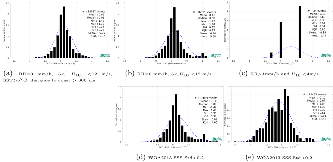
Figure 15: Normalized histogram of \Delta SSS (SMAP SSS L3 v5.0 - Monthly (JPL) - TSG (Polarstern)) for 5 different subdatasets corresponding to: RR=0 mm/h, 3 < U_{10} < 12 m/s, SST>5°C, distance to coast > 800 km (a), RR=0 mm/h, 3 < U_{10} < 12 m/s (b), RR>1mm/h and U_{10} < 4 m/s (c), WOA2013 SSS Std<0.2 (d), WOA2013 SSS Std>0.2 (e).
