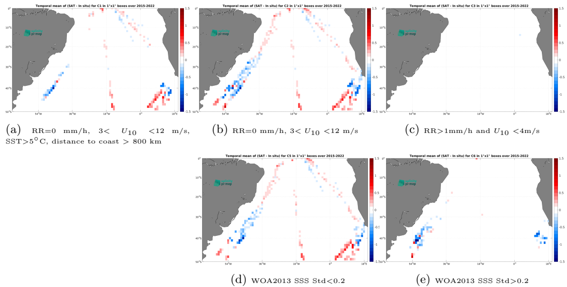
Figure 12: Temporal mean gridded over spatial boxes of size 1^\circ \times 1^\circ of \Delta\text{SSS} (SMAP SSS L3 v5.0 - Monthly (JPL) - TSG (Polarstern)) for 5 different subdatasets corresponding to:RR=0 mm/h, 3 < U_{10} < 12 m/s, SST >5^\circ\text{C} , distance to coast > 800 km (a), RR=0 mm/h, 3 < U_{10} < 12 m/s (b), RR >1 mm/h and U_{10} < 4 m/s (c), WOA2013 SSS Std <0.2 (d), WOA2013 SSS Std >0.2 (e).
