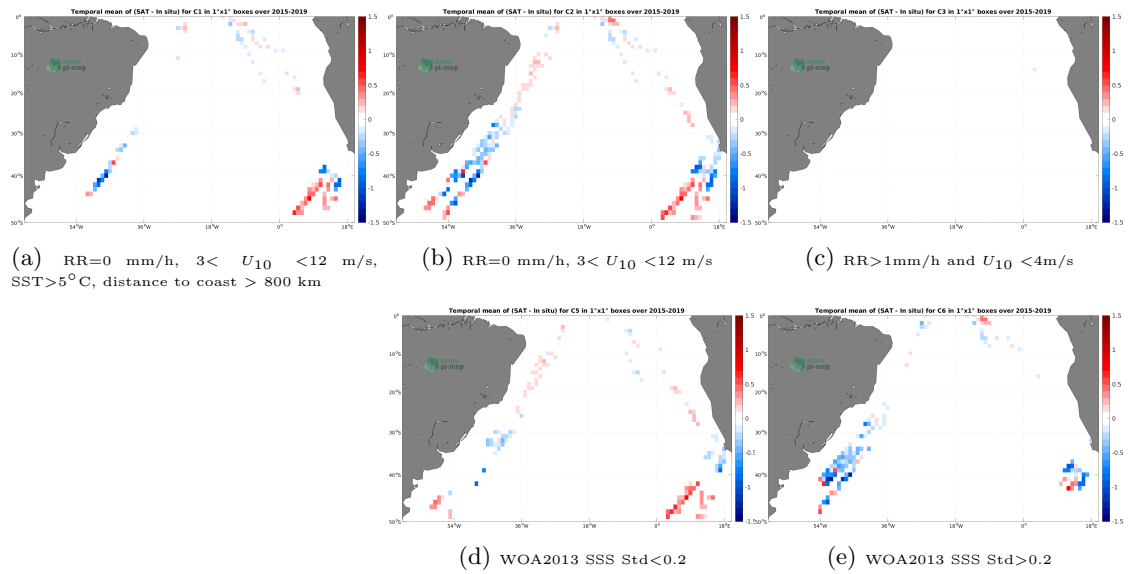
Figure 12: Temporal mean gridded over spatial boxes of size 1^\circ \times 1^\circ of \Delta SSS (SMAP SSS L3 v5.0 - Monthly (JPL) - TSG (Polarstern)) for 5 different subdatasets corresponding to:RR=0 mm/h, 3 < U_{10} < 12 m/s, SST >5^\circ\text{C} , distance to coast > 800 km (a), RR=0 mm/h, 3 < U_{10} < 12 m/s (b), RR >1 mm/h and U_{10} < 4 m/s (c), WOA2013 SSS Std <0.2 (d), WOA2013 SSS Std >0.2 (e).
