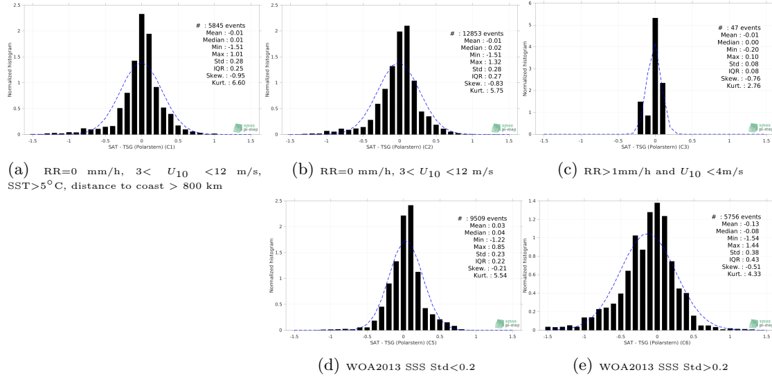
Figure 13: Normalized histogram of \Delta\text{SSS} (SMAP SSS L3 v5.0 - Monthly (JPL) - TSG (Polarstern)) for 5 different subdatasets corresponding to: RR=0 mm/h, 3 < U_{10} < 12 m/s, SST>5°C, distance to coast > 800 km (a), RR=0 mm/h, 3 < U_{10} < 12 m/s (b), RR>1mm/h and U_{10} < 4 m/s (c), WOA2013 SSS Std<0.2 (d), WOA2013 SSS Std>0.2 (e).
