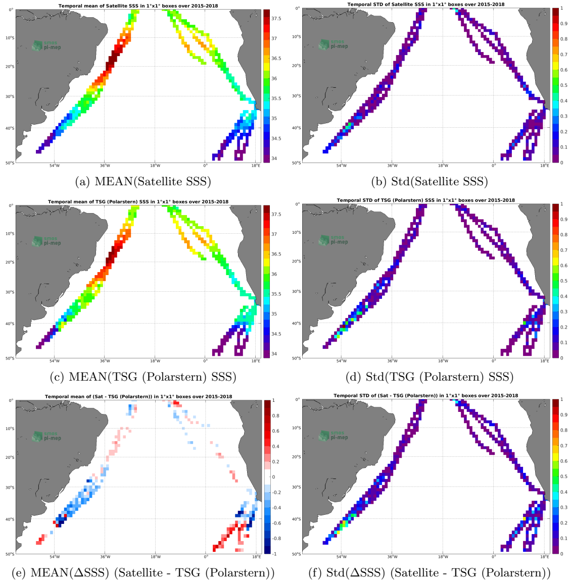
Figure 6: Temporal mean (left) and Std (right) of SSS from SMAP SSS L3 v5.0 - Monthly (JPL) (top), TSG (Polarstern) (middle), and of \Delta SSS (Satellite - TSG (Polarstern)). Only match-up pairs are used to generate these maps.
