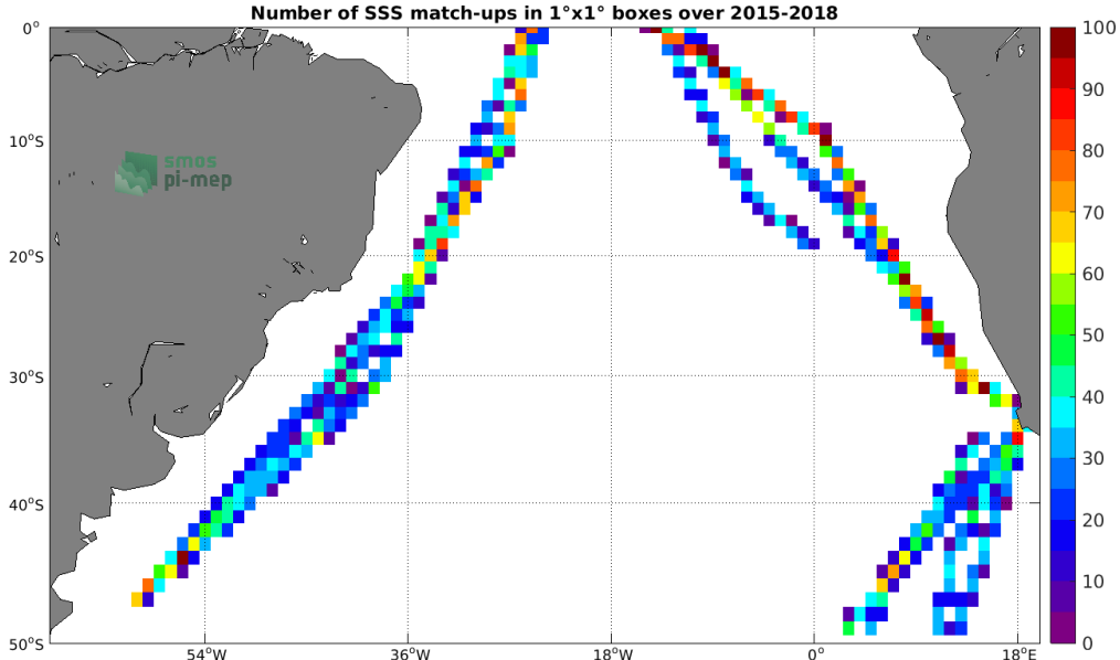
Figure 4: Number of SSS match-ups between TSG (Polarstern) SSS and the SMAP SSS L3 v5.0 - Monthly (JPL) SSS product for the South Atlantic Ocean Pi-MEP region over 1°x1° boxes and for the full satellite product period.
