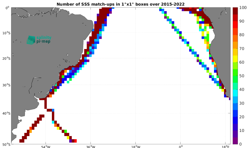
Figure 5: Number of SSS match-ups between TSG (LEGOS-DM) SSS and the SMAP SSS L3 v5.0 - Monthly (JPL) SSS product for the South Atlantic Ocean Pi-MEP region over 1^\circ \times 1^\circ boxes and for the full satellite product period.
