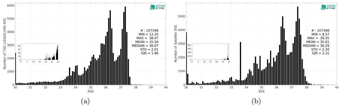
Figure 3: Histograms of SSS from TSG (LEGOS-DM) (a) and SMAP SSS L3 v5.0 - Monthly (JPL) (b) considering all match-up pairs per bins of 0.1 over the South Atlantic Ocean Pi-MEP region and for the full satellite product period.
