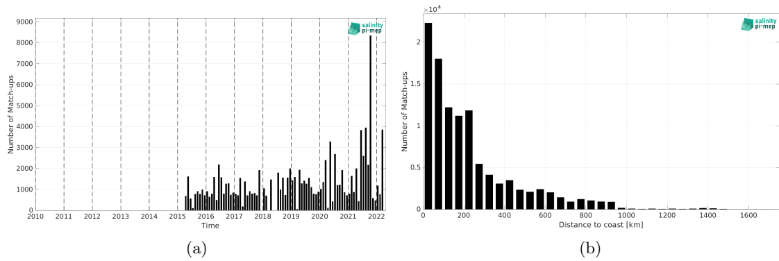
Figure 2: Number of match-ups between TSG (LEGOS-DM) and SMAP SSS L3 v5.0 - Monthly (JPL) SSS as a function of time (a) and as function of the distance to coast (b) over the South Atlantic Ocean Pi-MEP region and for the full satellite product period.
