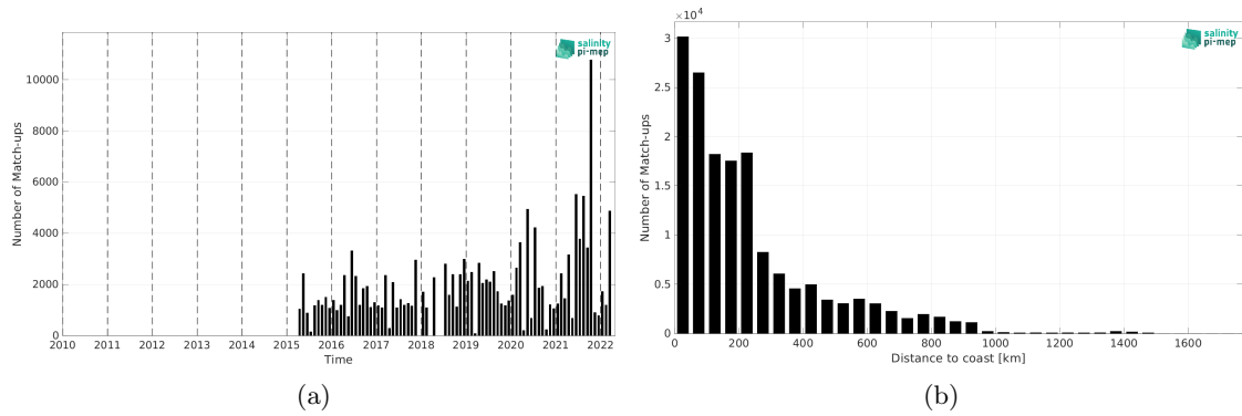
Figure 1: Number of match-ups between TSG (LEGOS-DM) and SMAP SSS L3 v5.0 - Monthly (JPL) SSS as a function of time (a) and as function of the distance to coast (b) over the South Atlantic Ocean Pi-MEP region and for the full satellite product period.
