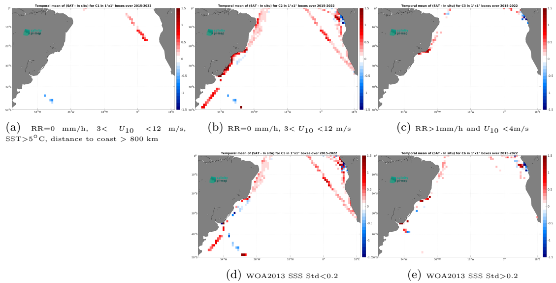
Figure 12: Temporal mean gridded over spatial boxes of size 1^\circ \times 1^\circ of \Delta SSS (SMAP SSS L3 v5.0 - Monthly (JPL) - TSG (LEGOS-DM)) for 5 different subdatasets corresponding to:RR=0 mm/h, 3 < U_{10} < 12 m/s, SST >5^\circ\text{C} , distance to coast > 800 km (a), RR=0 mm/h, 3 < U_{10} < 12 m/s (b), RR >1 mm/h and U_{10} < 4 m/s (c), WOA2013 SSS Std <0.2 (d), WOA2013 SSS Std >0.2 (e).
