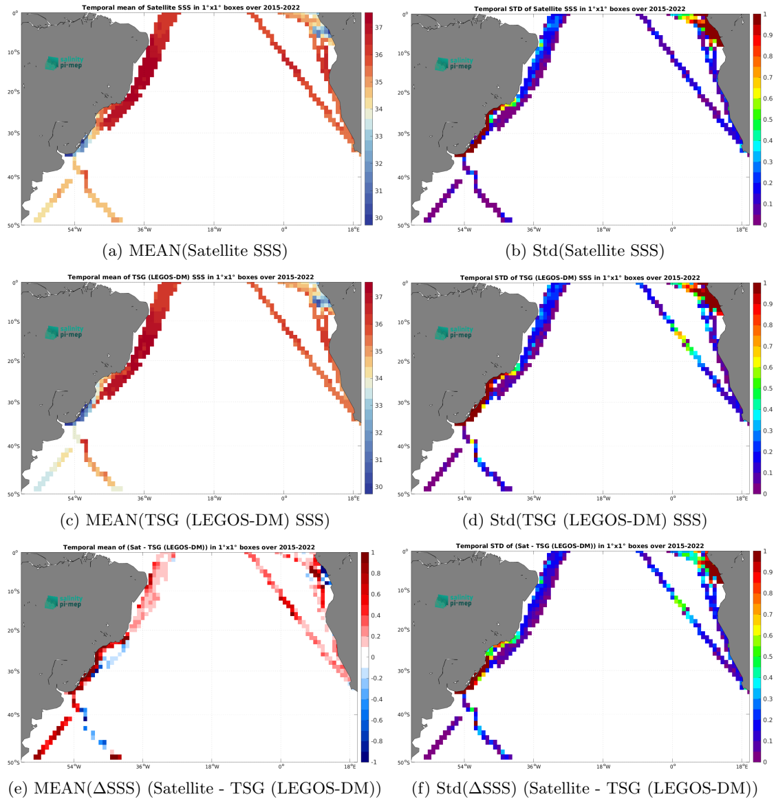
Figure 6: Temporal mean (left) and Std (right) of SSS from SMAP SSS L3 v5.0 - Monthly (JPL) (top), TSG (LEGOS-DM) (middle), and of \Delta SSS (Satellite - TSG (LEGOS-DM)). Only match-up pairs are used to generate these maps.
